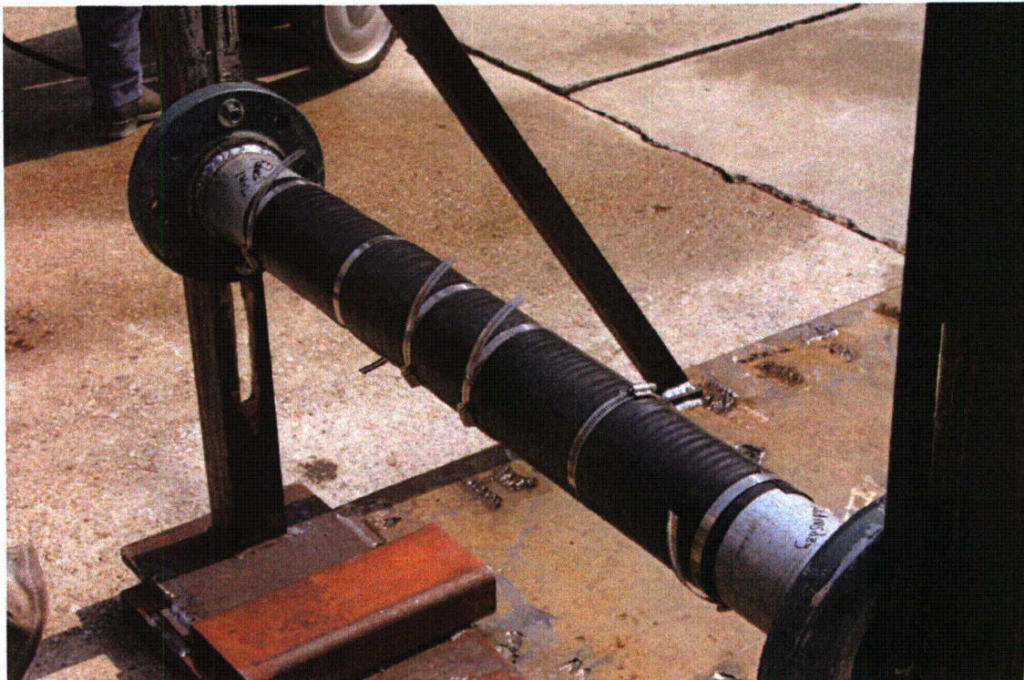
Figure A5-40 Scotch 77 Fire Retardant Tape Test 1 Pre-Test Picture
