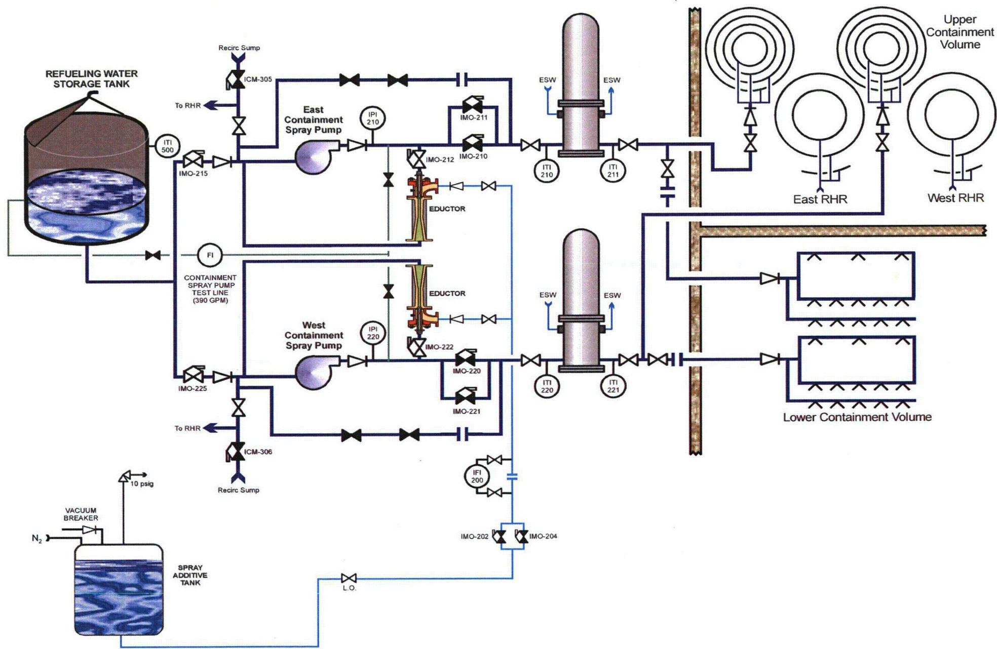
Figure A4-15 CTS
