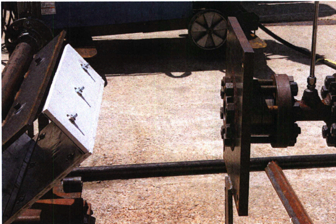
Figure A5-36 Marinite Test 13 Pre-Test Picture
