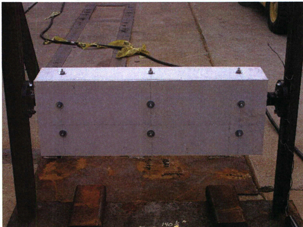
Figure A5-3 Marinite Test 2 Pre-Test Picture
