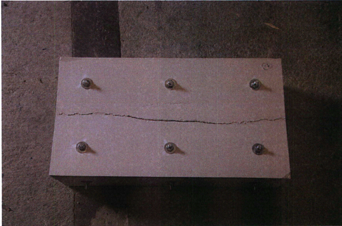
Figure A5-17 Marinite Test 7 Post-Test Picture
