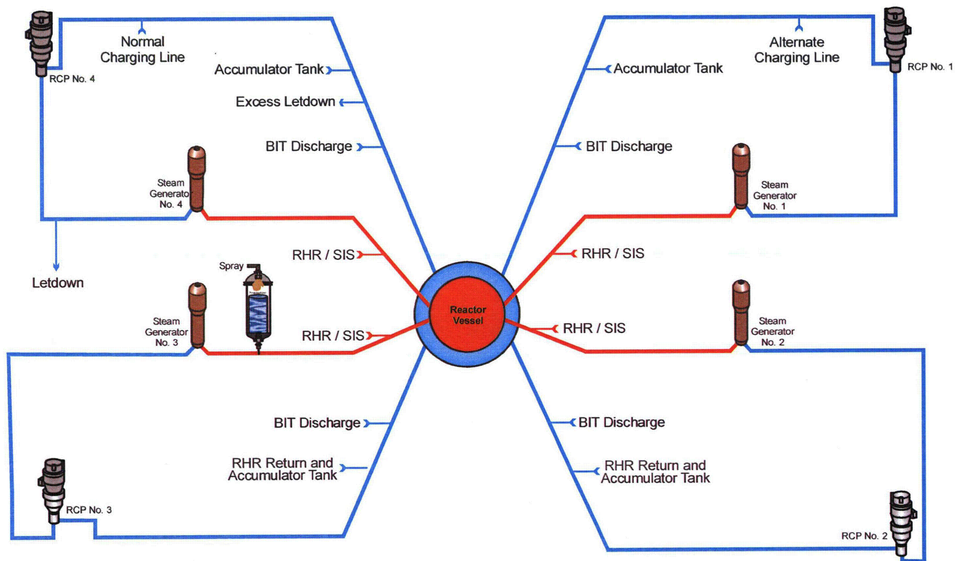
Figure A4-11 RCS
