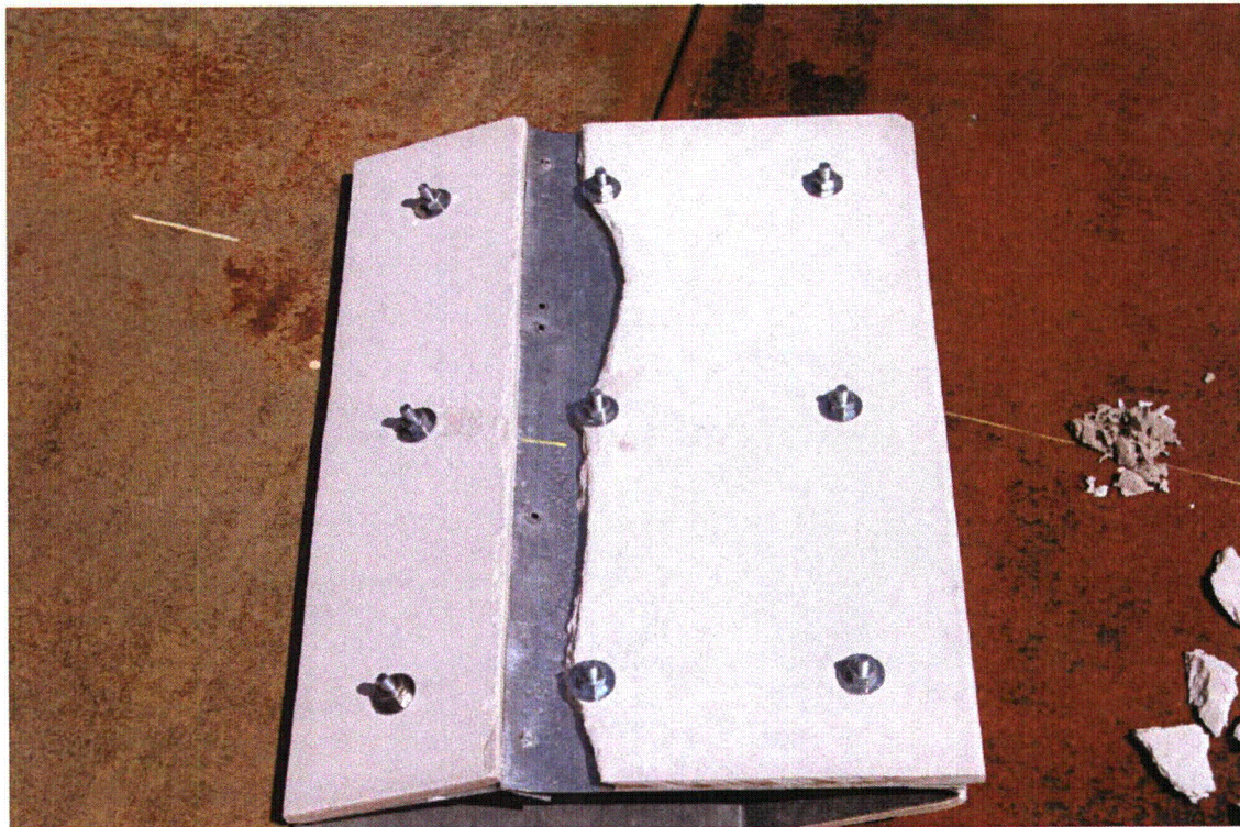
Figure A5-38 Marinite Test 13 Post-Test Picture
