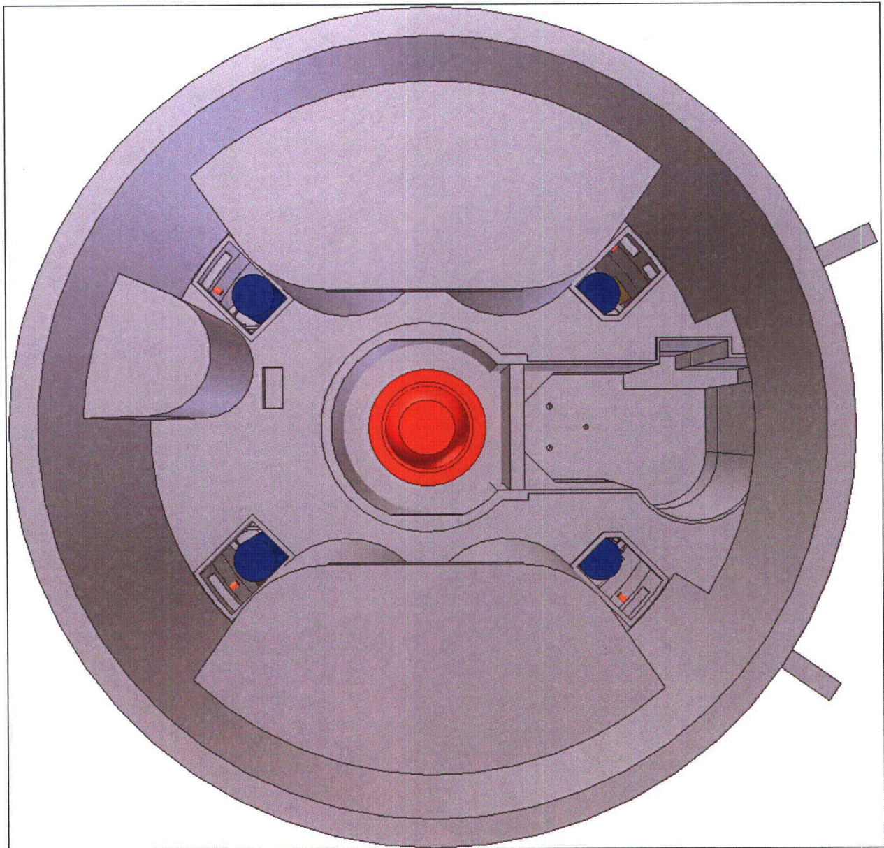
Figure A4-2 – Plan View of Unit 1 Upper Containment CAD Model
