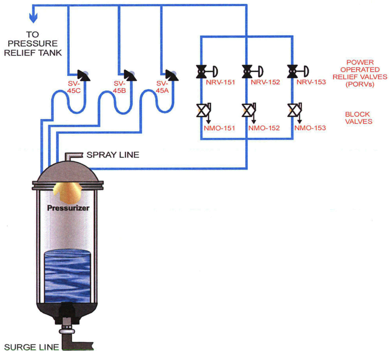
Figure A4-12 PZR Safety and Relief Valve Piping
