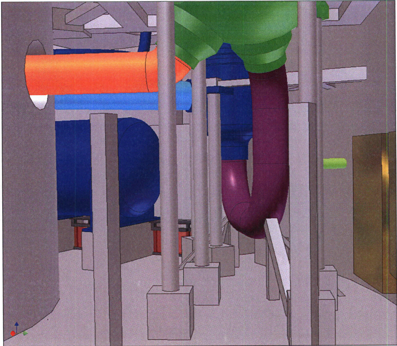
Figure A4-9 – Close-up of Unit 1 Loop 4 Piping, Equipment, and Supports CAD Model
