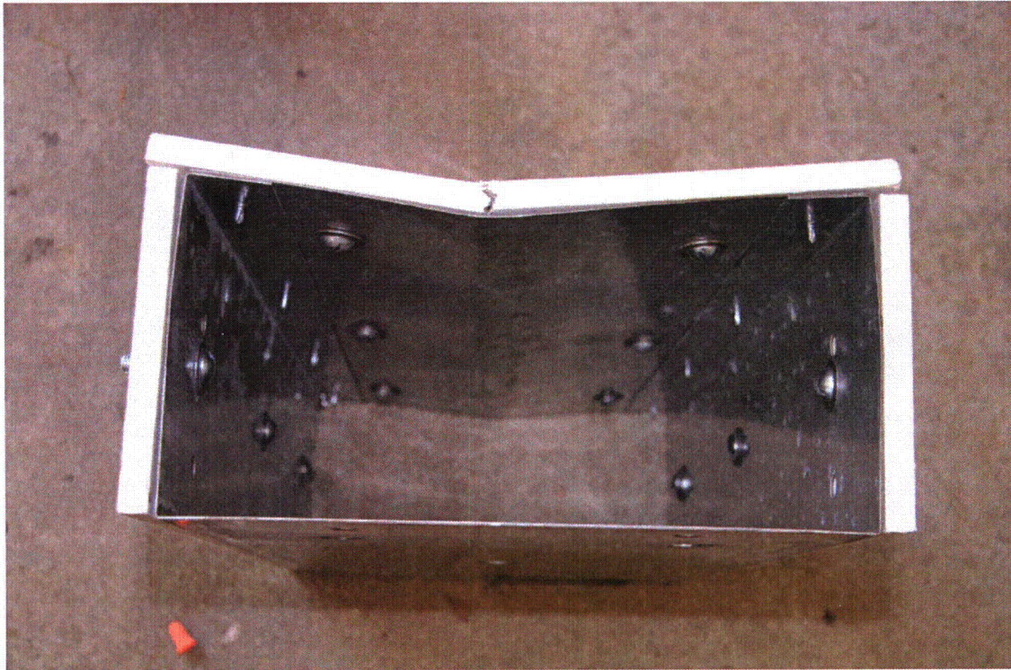
Figure A5-35 Marinite Test 12 Post-Test Picture
