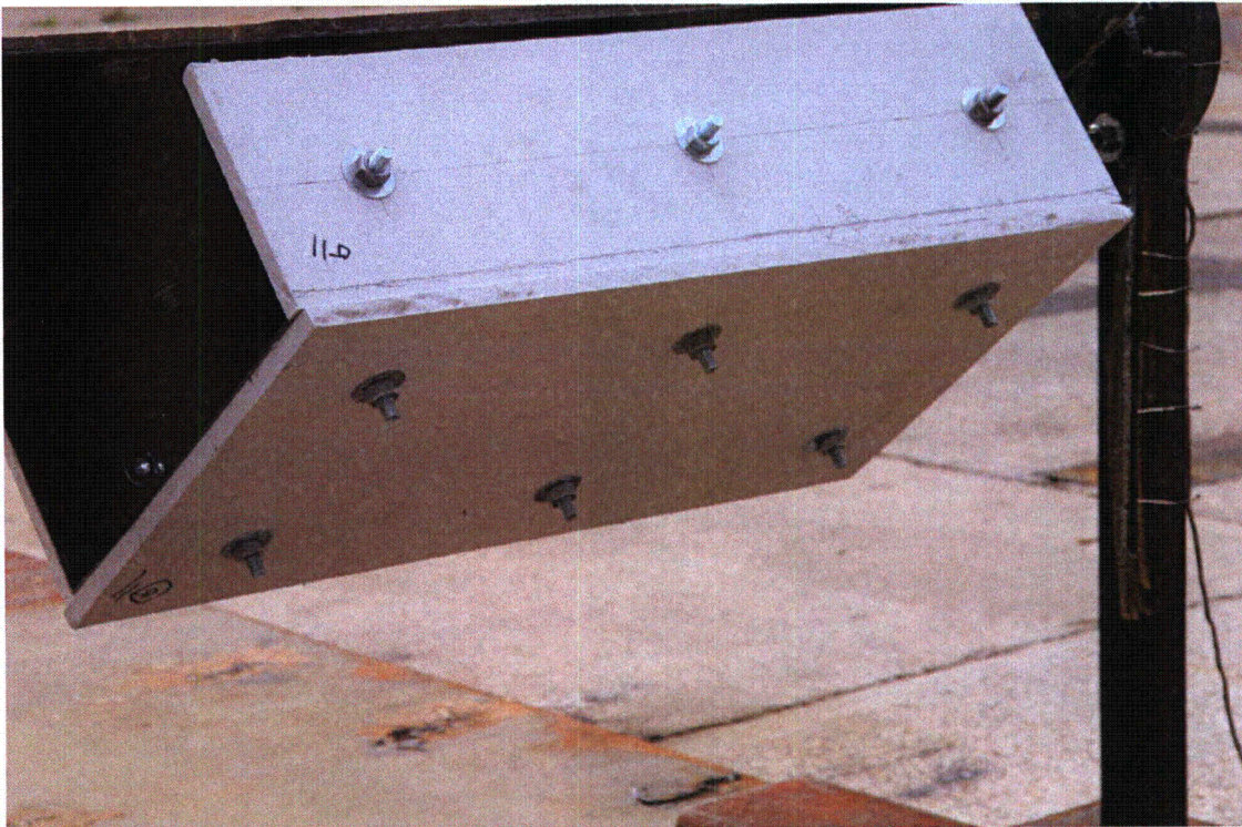
Figure A5-23 Marinite Test 9 Pre-Test Picture
