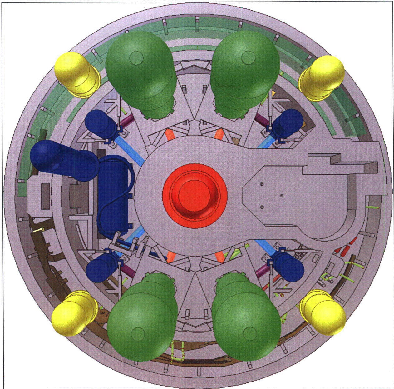
Figure A4-3 – Plan View of Unit 1 Lower Containment CAD Model
