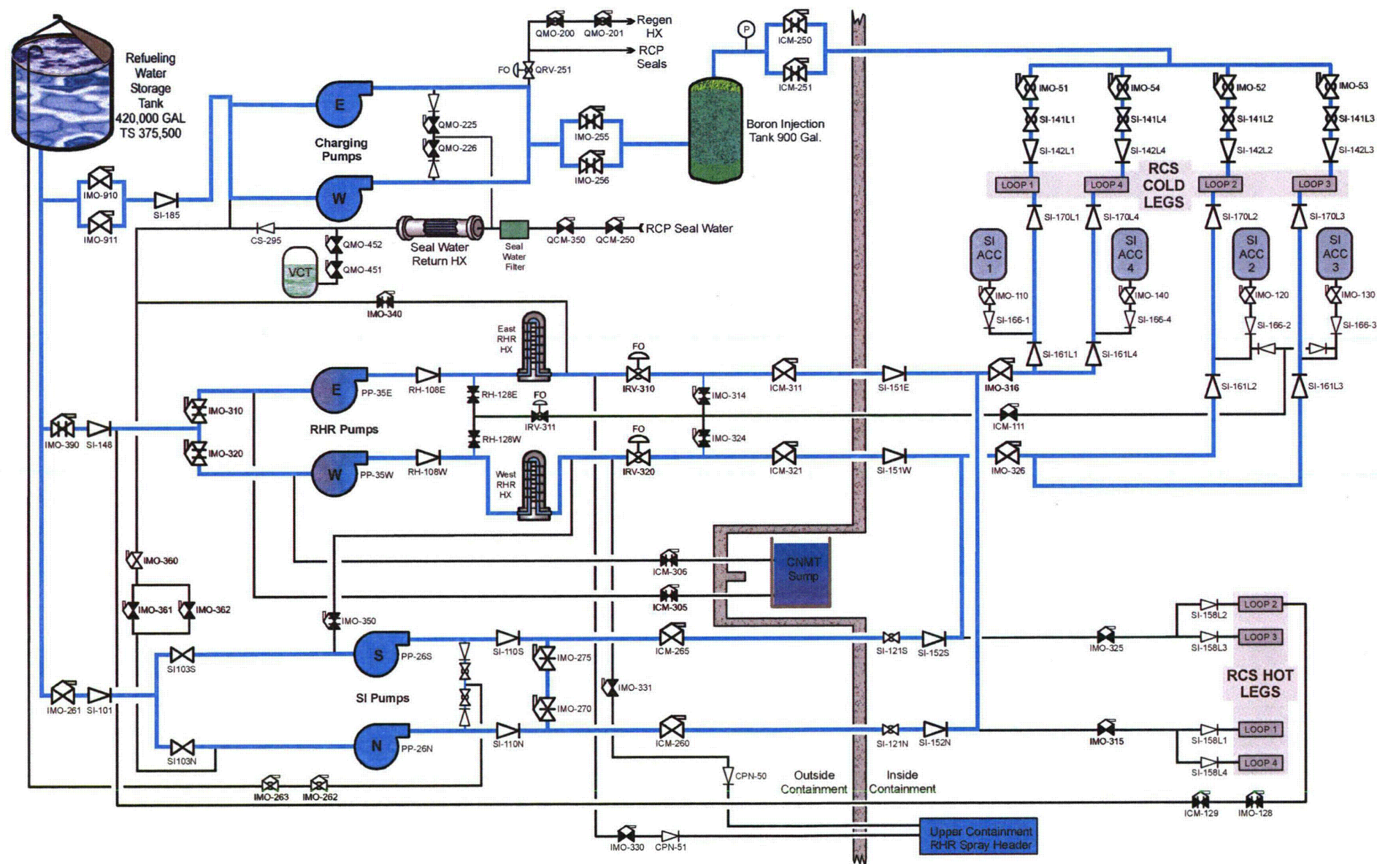
Figure A4-13 ECCS Injection
