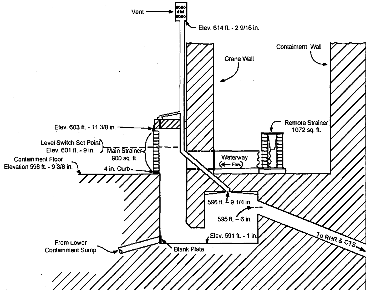
Figure A4-1 General Arrangement of Recirculation Sump
