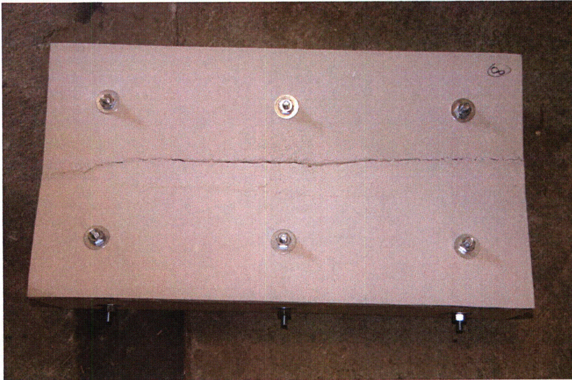
Figure A5-21 Marinite Test 8 Post-Test Picture
