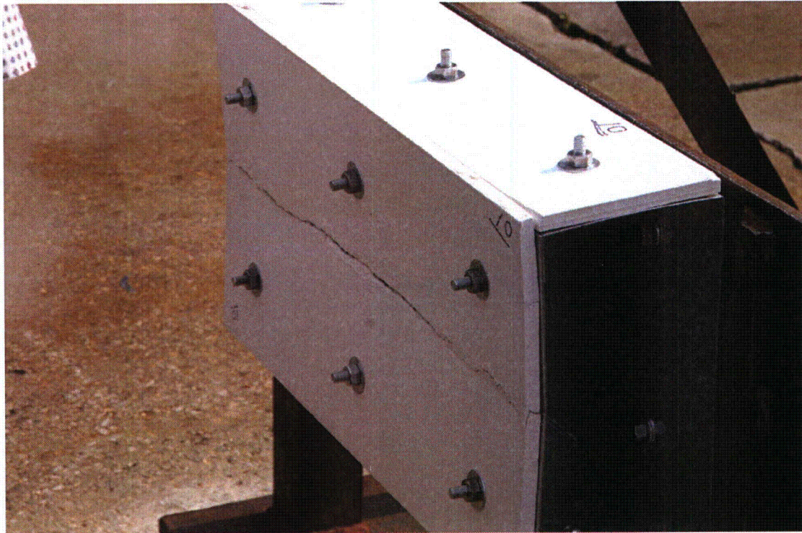
Figure A5-27 Marinite Test 10 Post-Test Picture
