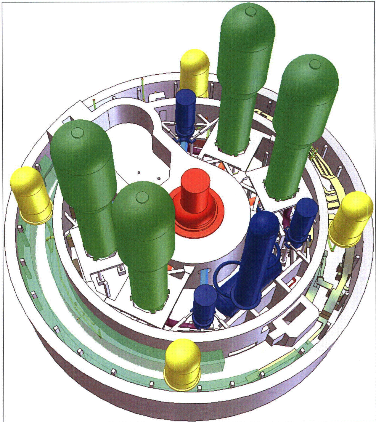
Figure A4-6 – Northeast Isometric View of Unit 1 Lower Containment CAD Model
