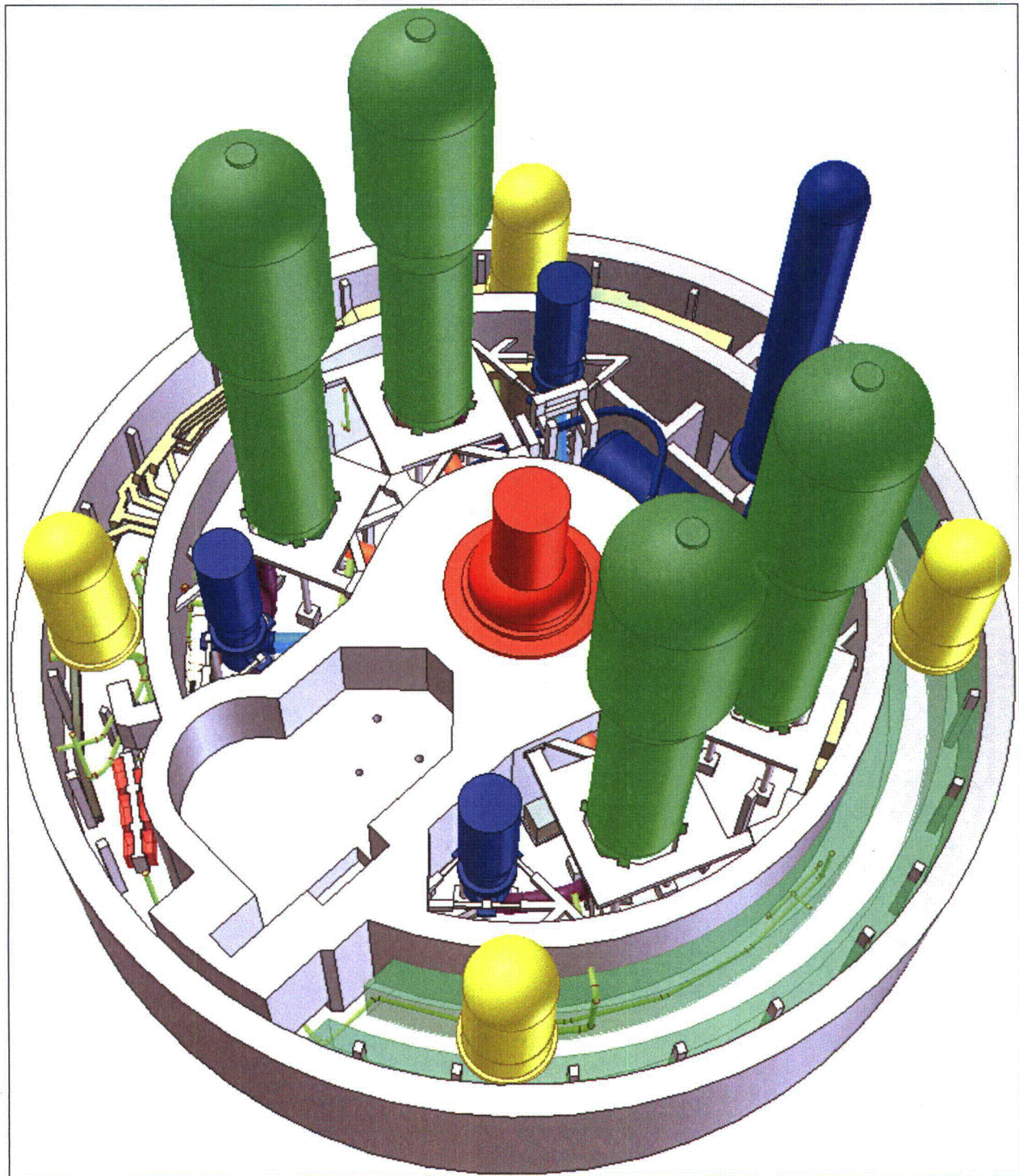
Figure A4-5 – Southeast Isometric View of Unit 1 Lower Containment CAD Model
