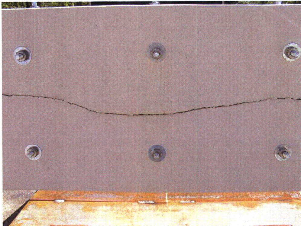
Figure A5-10 Marinite Test 5 Post-Test Picture
