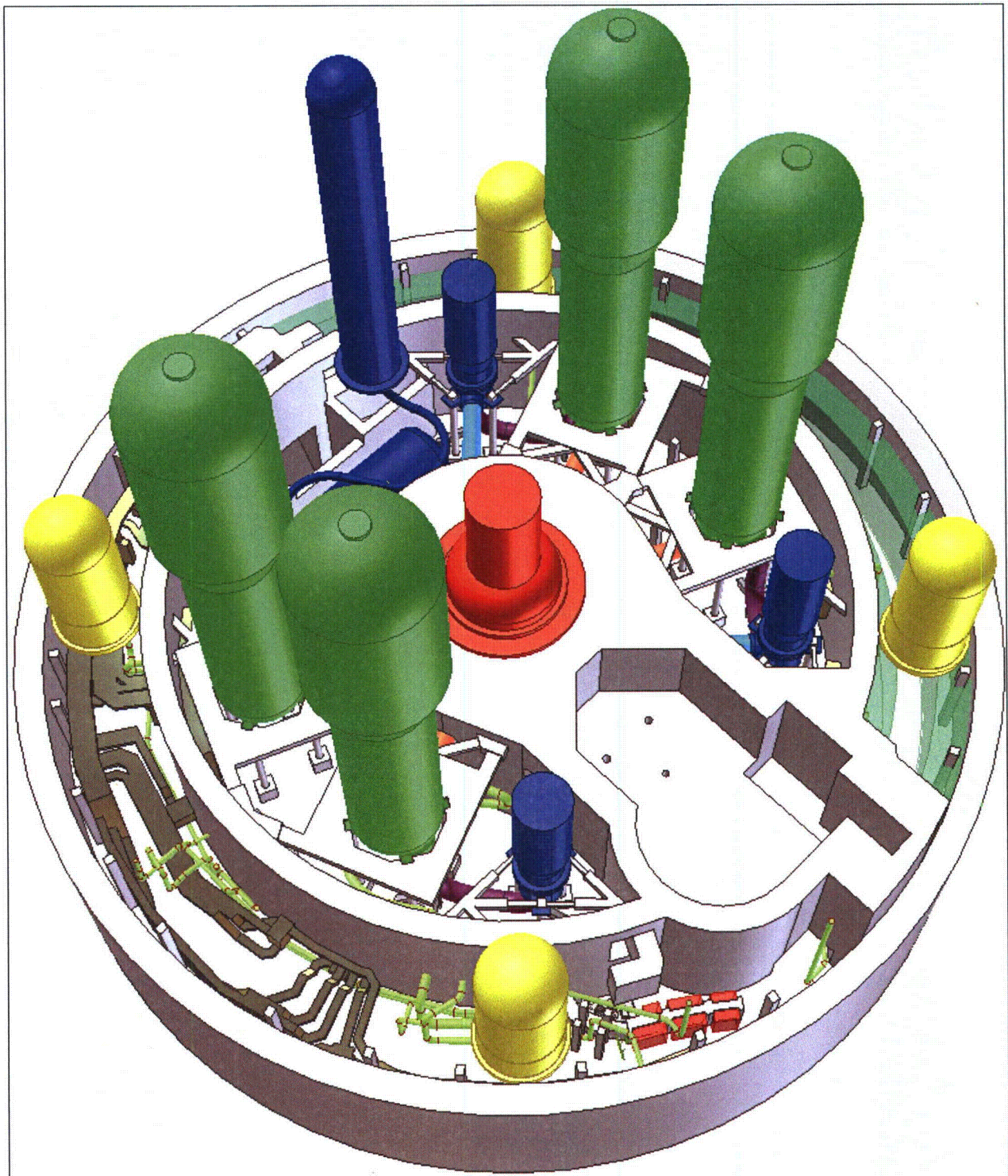
Figure A4-4 – Southwest Isometric View of Unit 1 Lower Containment CAD Model
