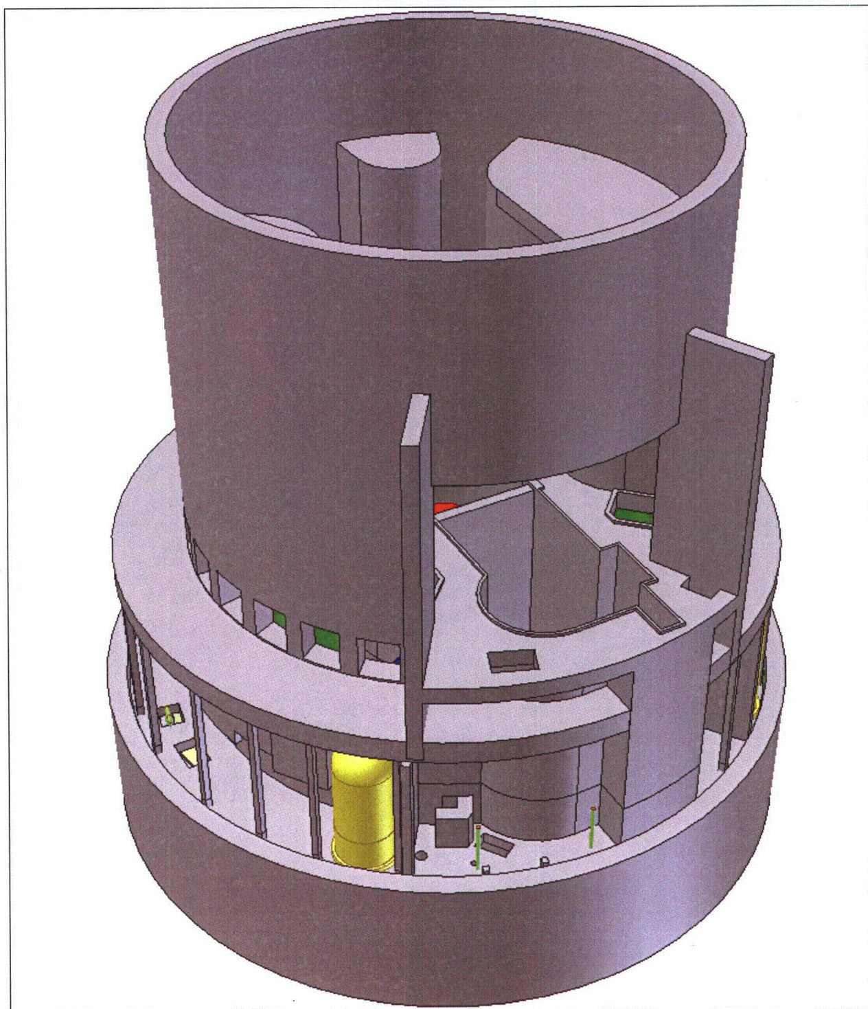
Figure A4-8 – Isometric View of Unit 1 Area Outside Crane Wall CAD Model
