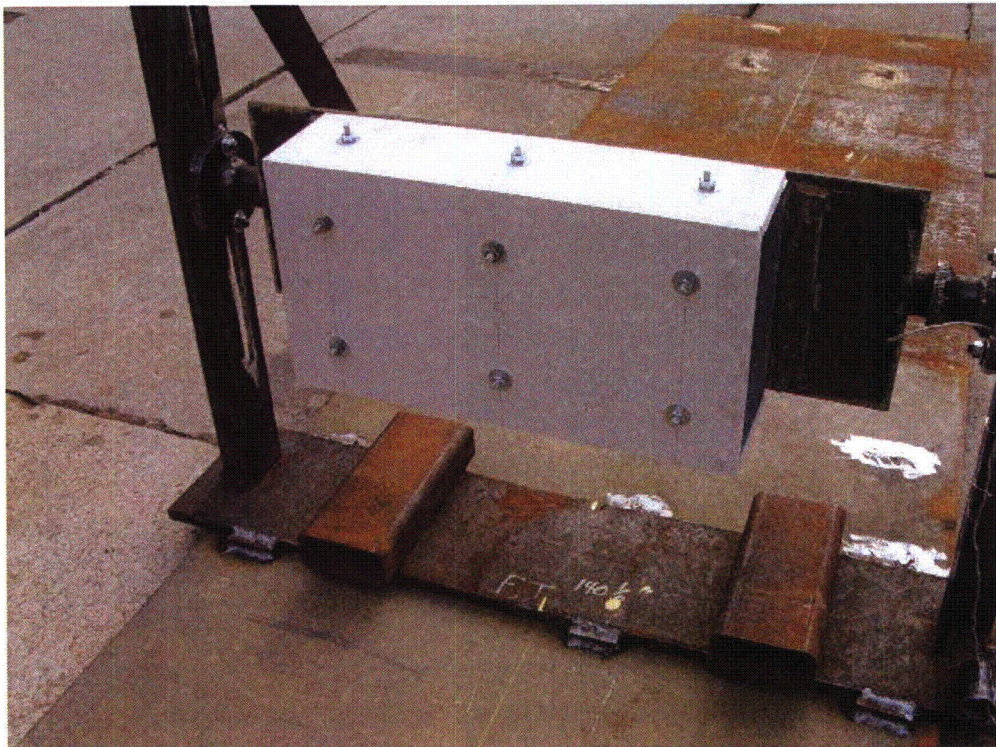
Figure A5-12 Marinite Test 6 Pre-Test Picture
