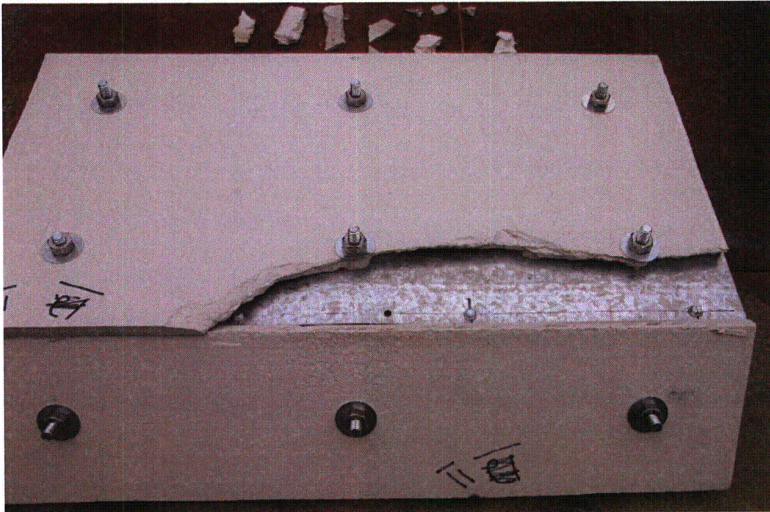
Figure A5-31 Marinite Test 11 Post-Test Picture
