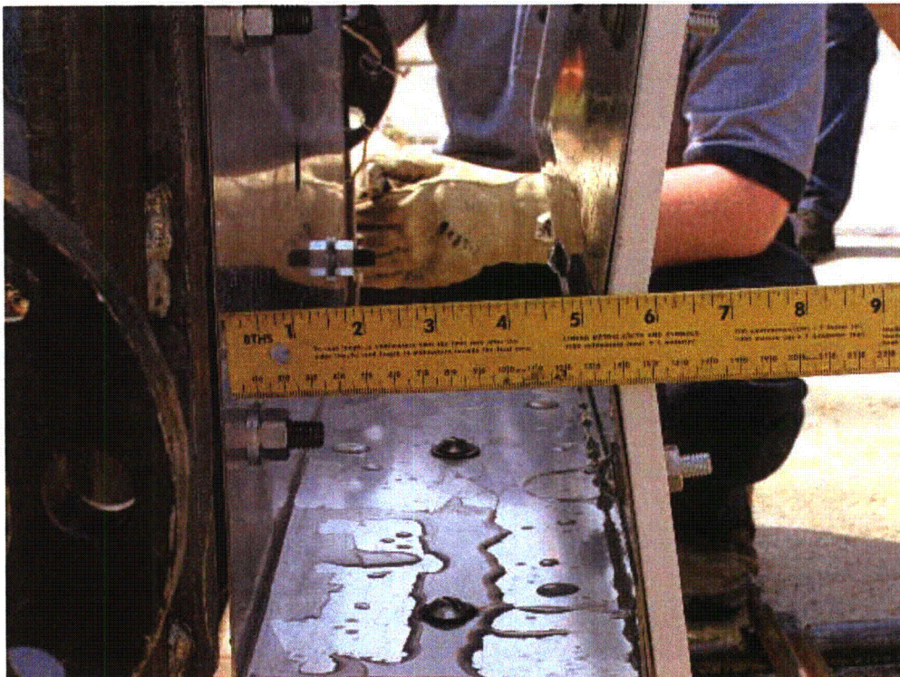
Figure A5-14 Marinite Test 6 Post-Test Picture
