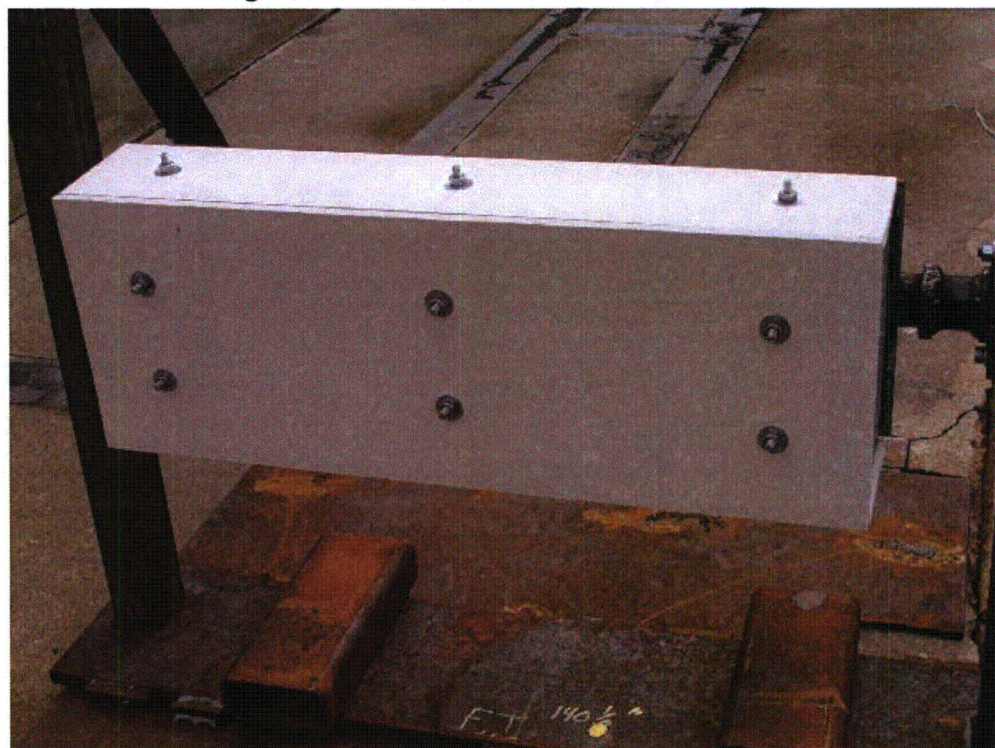
Figure A5-4 Marinite Test 2 Post-Test Picture
