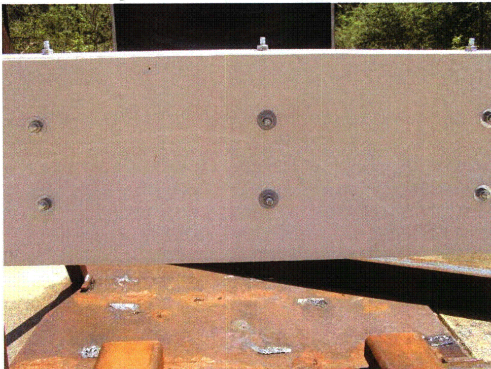
Figure A5-8 Marinite Test 4 Post-Test Picture
