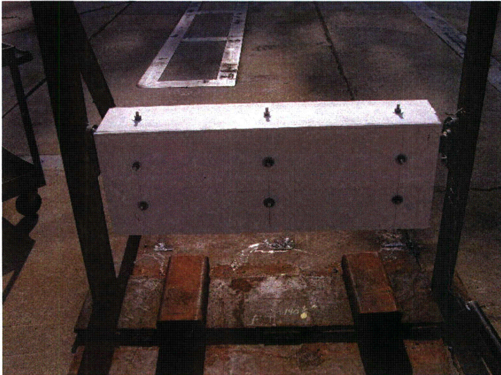
Figure A5-5 Marinite Test 3 Pre-Test Picture
