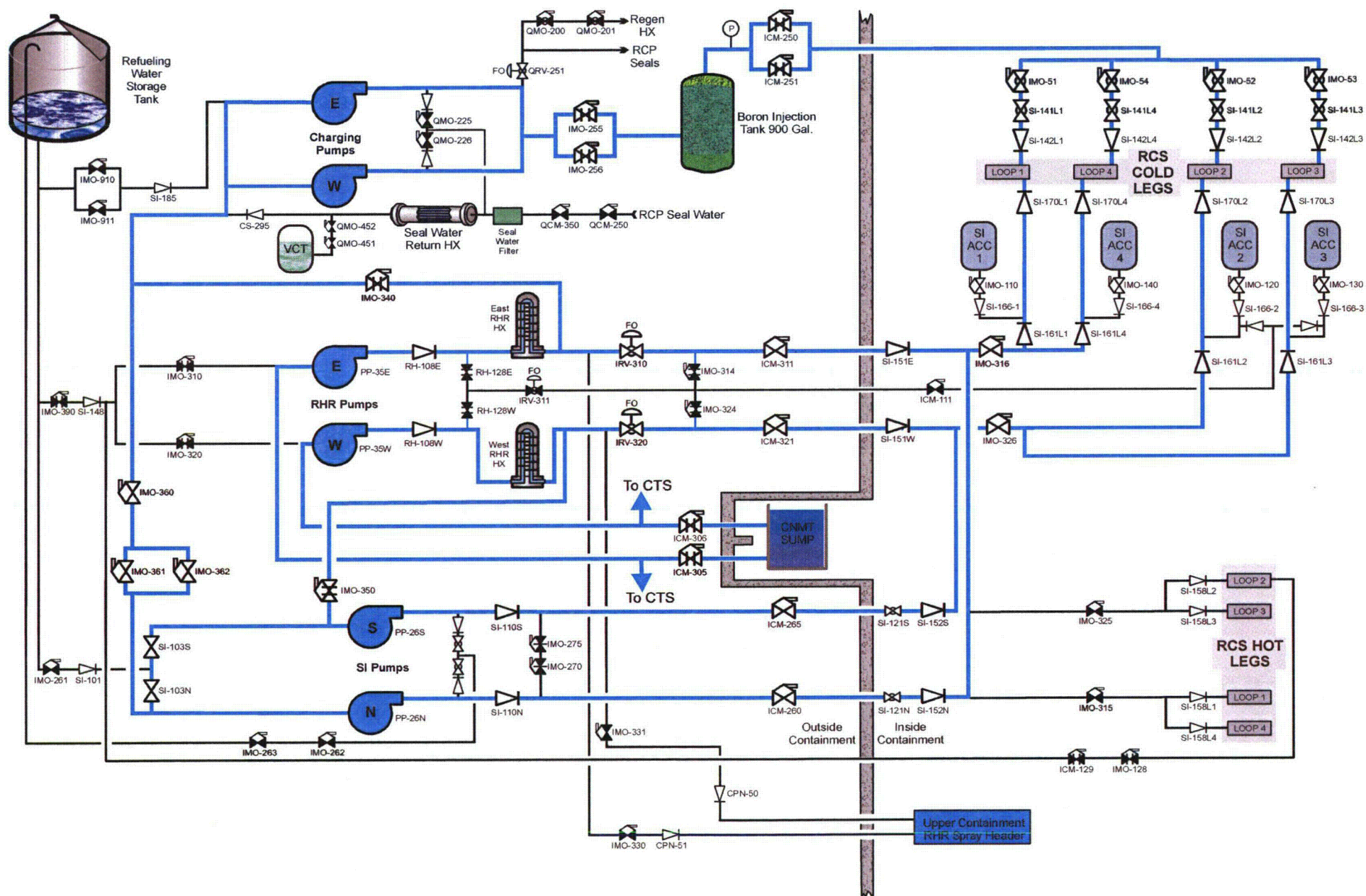
Figure A4-14 ECCS Recirculation
