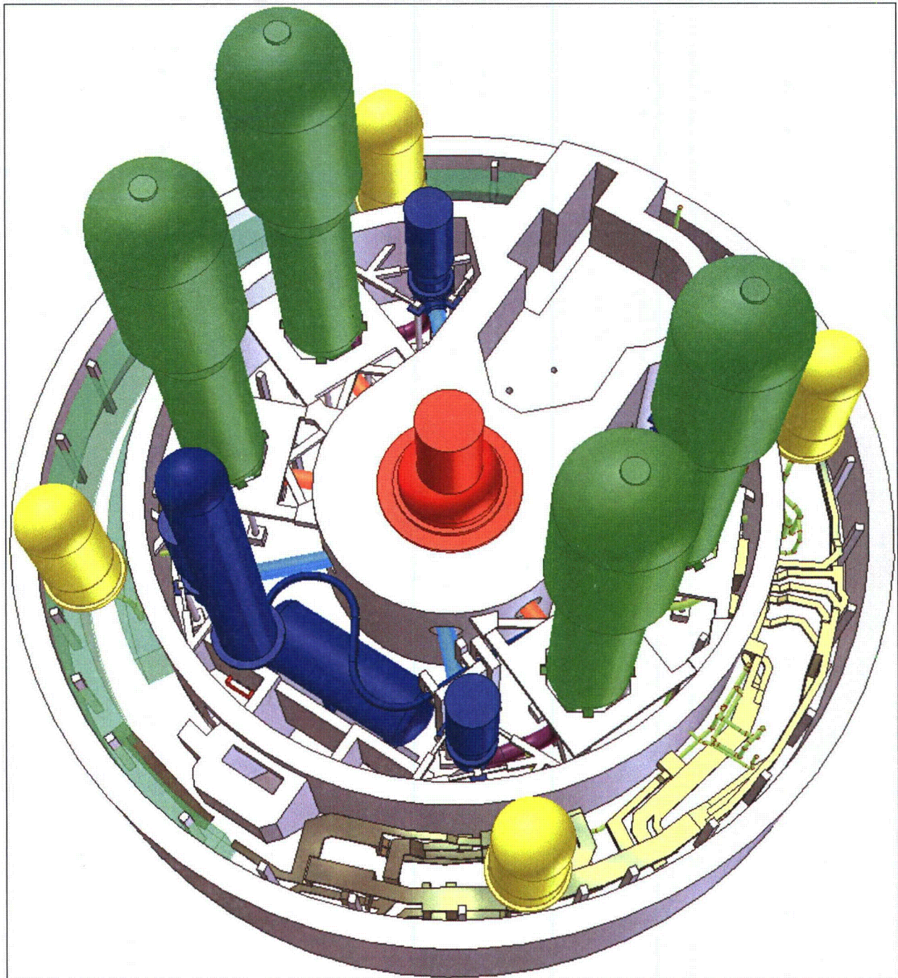
Figure A4-7 – Northwest Isometric View of Unit 1 Lower Containment CAD Model
