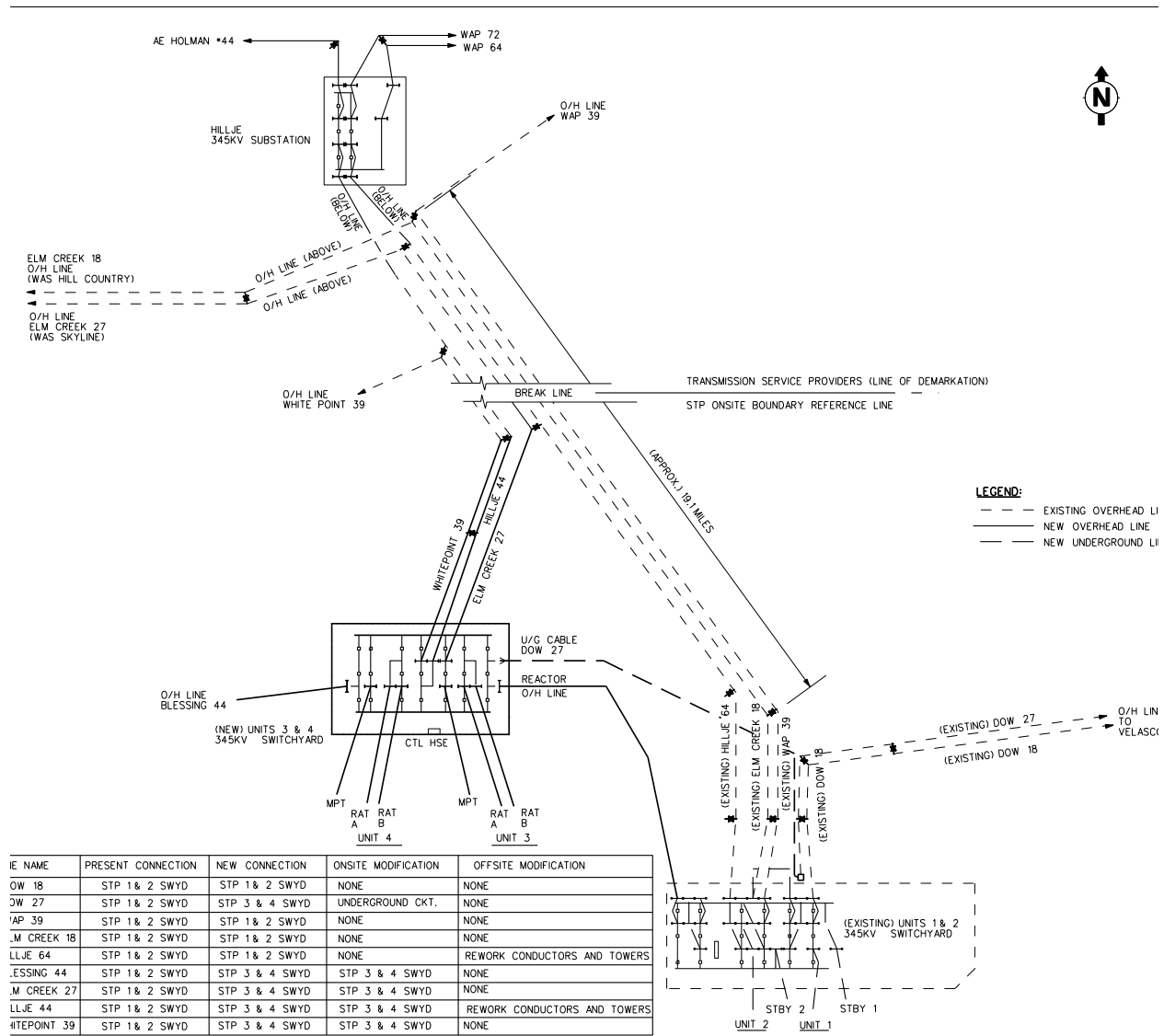
Figure 3.7-6 345kV Transmission Configuration for STP 1 &amp; 2 and STP 3 &amp; 4
