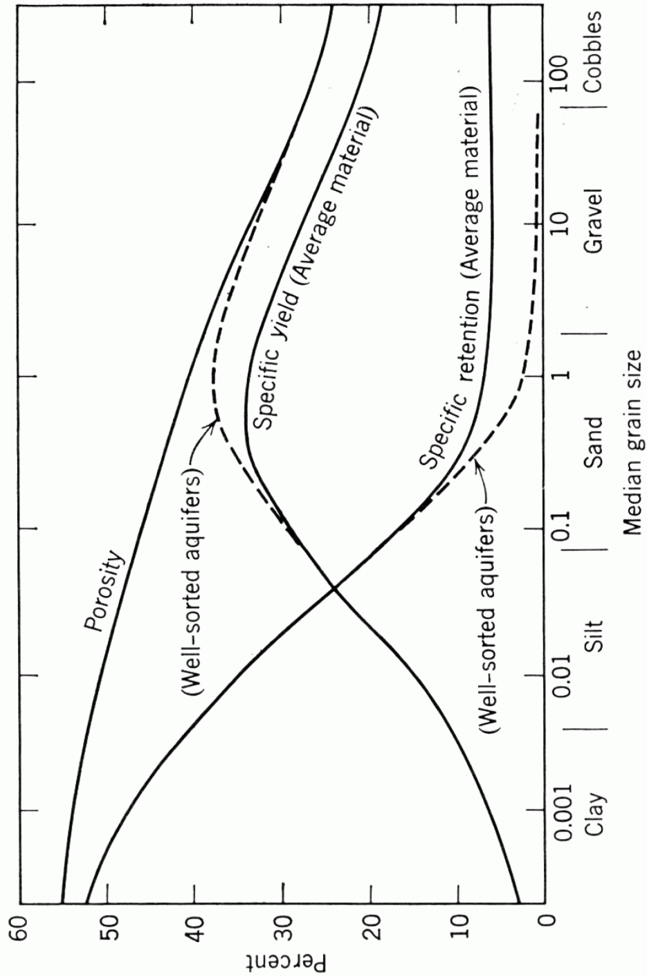
Figure 2.3.1-33 Relationship of Porosity, Specific Yield, and Specific Retention (Reference 2.3.1-28)
