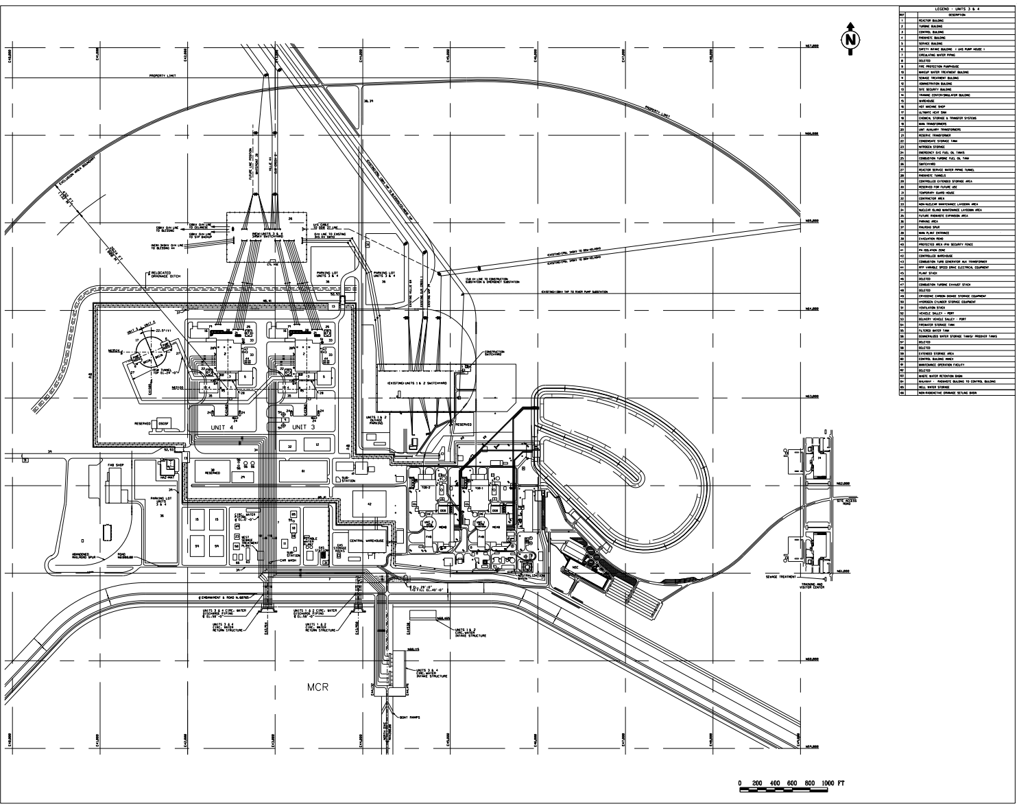
Figure 1.1-1 Site Layout
