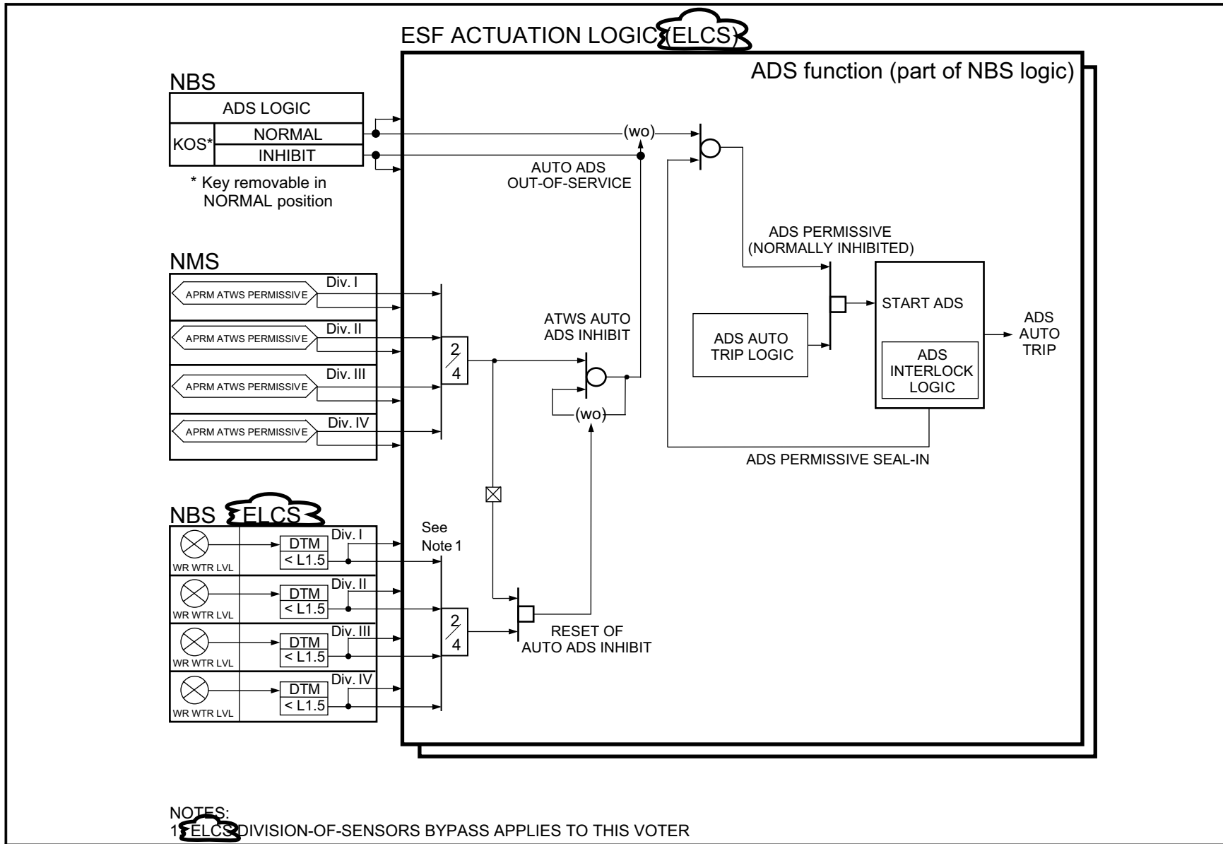
Figure 15E-1c ATWS Mitigation Logic (SLCS Initiation, Feedwater Runback)
