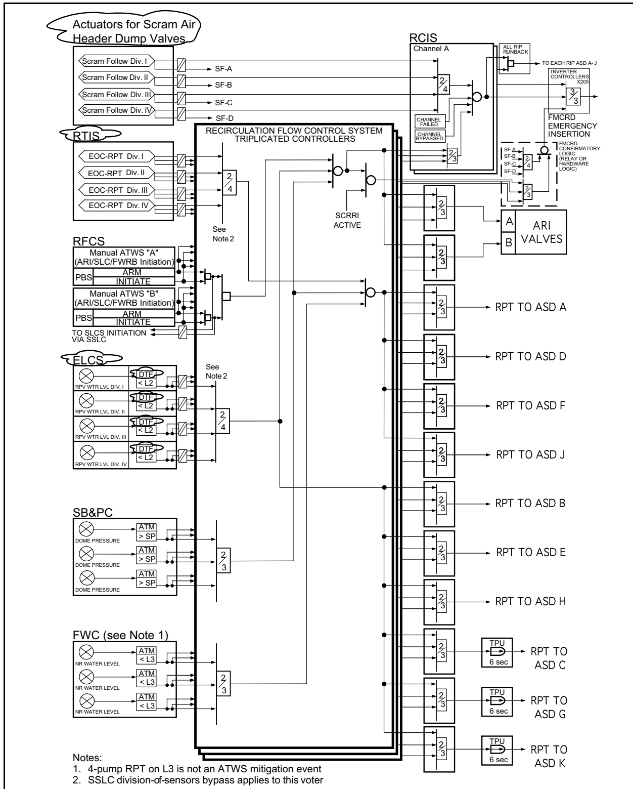
Figure 15E-1a ATWS Mitigation Logic (ARI, FMCRD Run-In, RPT, Manual Initiation)
