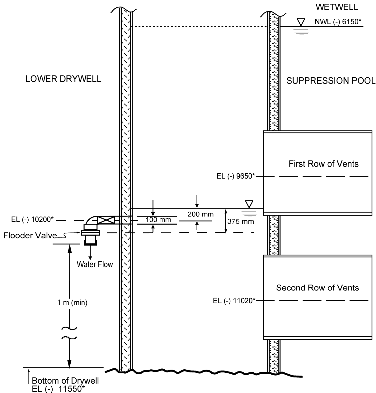
Figure 9.5-3 Lower Drywell Flooder System Arrangement/Configuration
