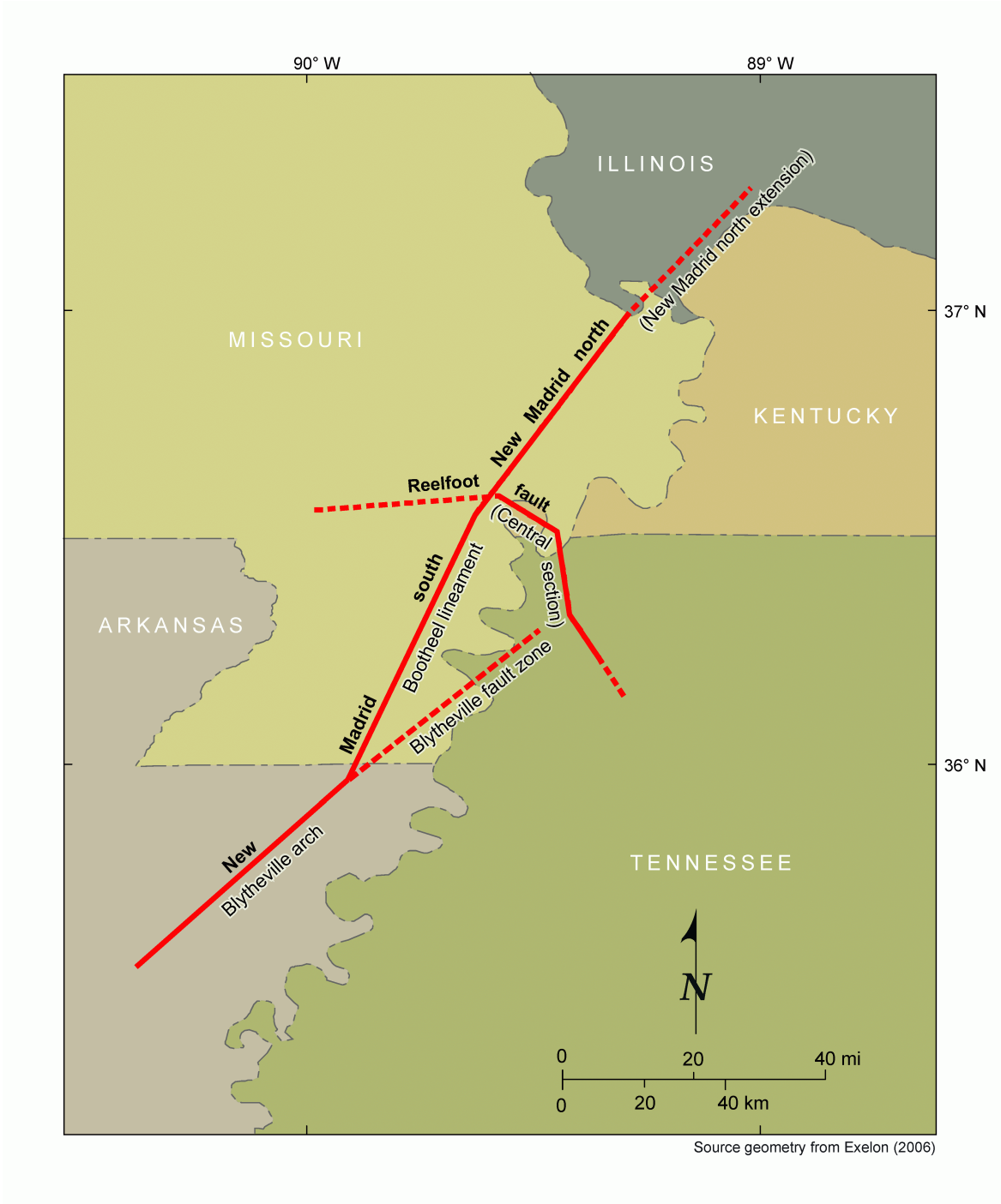
Figure 2.5S.2-12 New Madrid Faults from Clinton ESP Source Model
