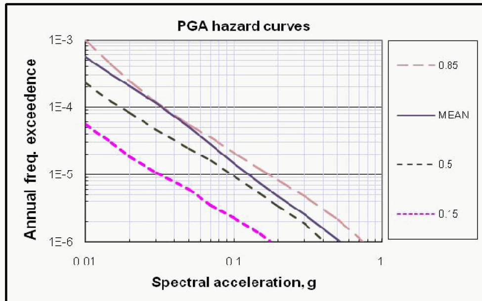
Figure 2.5S.2-18 Mean and Fractile PGA Rock Hazard Curves
