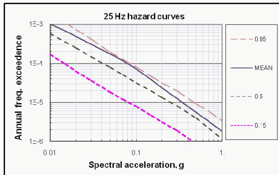
Figure 2.5S.2-19 Mean and Fractile 25 Hz Rock Hazard Curves
