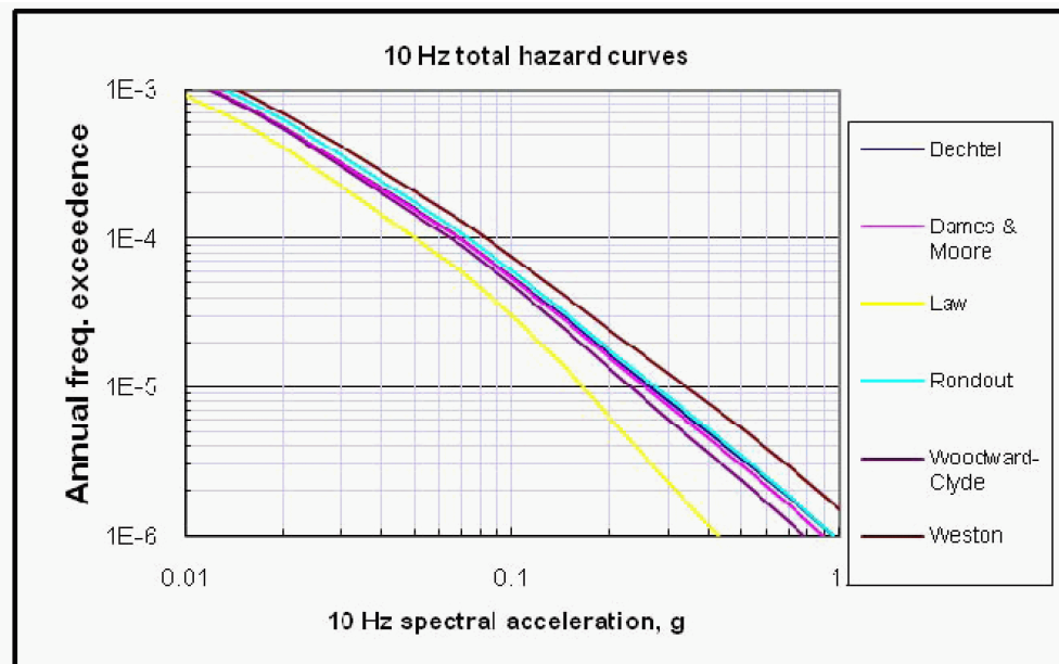
Figure 2.5S.2-14 Mean 10 Hz Rock Hazard Curves by EST
