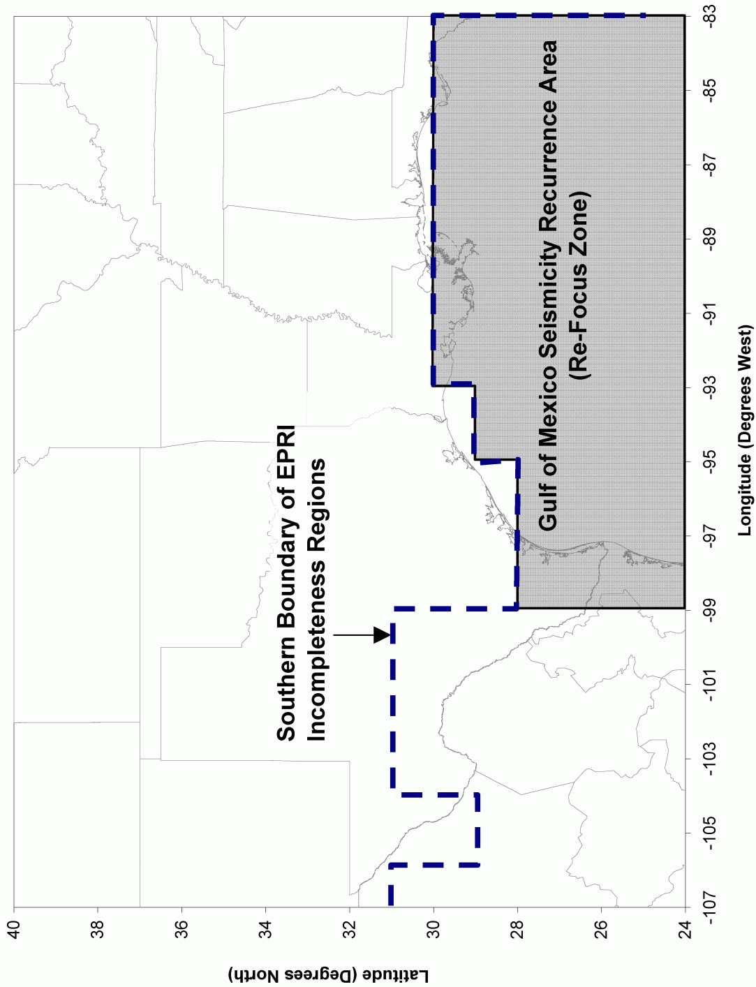
Figure 2.5S.2-7 Southern Boundary of EPR Incompleteness Regions (Reference 2.5S.2-3) and Gulf of Mexico Seismicity Recurrence Area (Re-Focus Zone)
