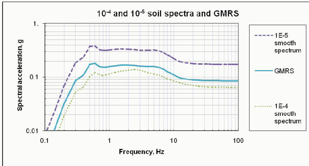
Figure 2.5S.2-52 Smooth 10^{-4} and 10^{-5} Soil UHRS, and Resulting GMRS
