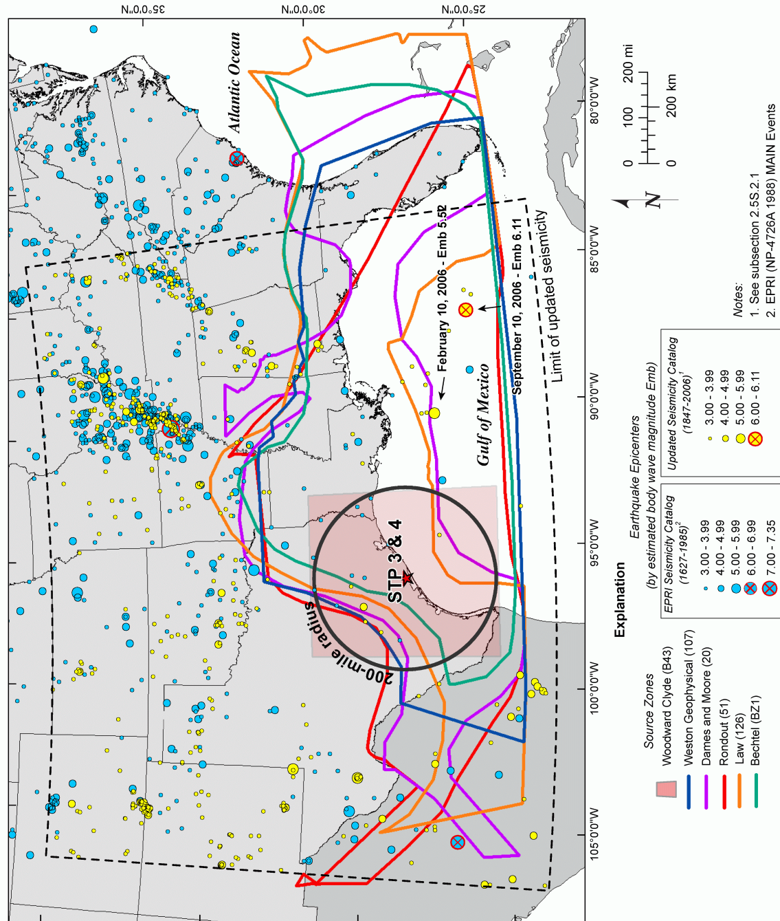
Figure 2.5S.2-8 EPRSI EST Gulf Coast Background Source Zones
