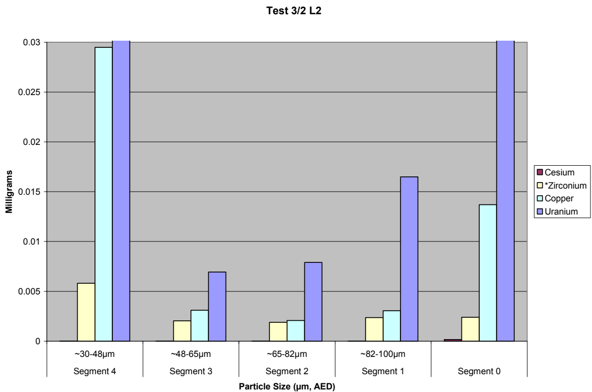
Figure A3.2A.10 Test 3/2 (A) LPS L2 Metals Analysis Distribution, mg
