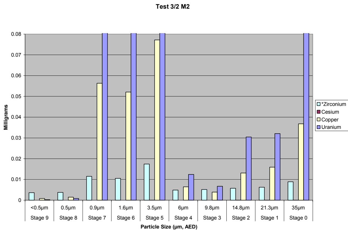
Figure A3.2A.9 Test 3/2 (A) Marple M2 Metals Analysis Distribution, mg
