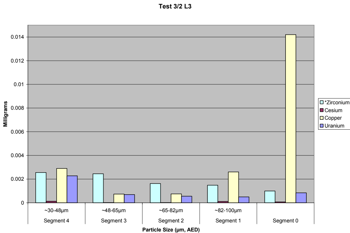
Figure A3.2A.12 Test 3/2 (A) LPS L3 Metals Analysis Distribution, mg
