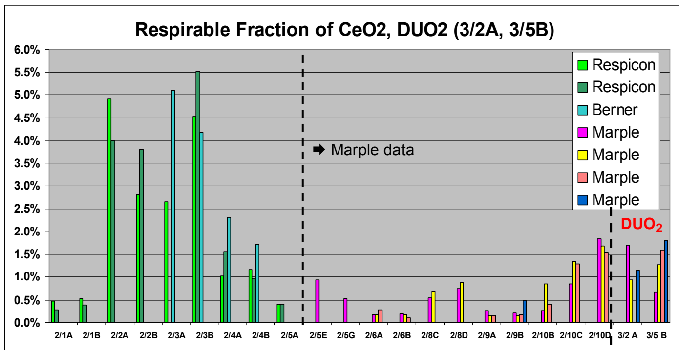
Figure 7.1 Phases 2, 2+, and 3 Test Results for CeO 2 and DUO 2 Respirable Fractions
