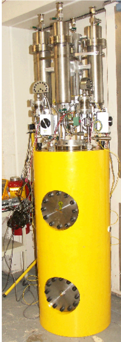
Figure 5.4 Phase 3 Test Chamber and Aerosol Sampling Systems
