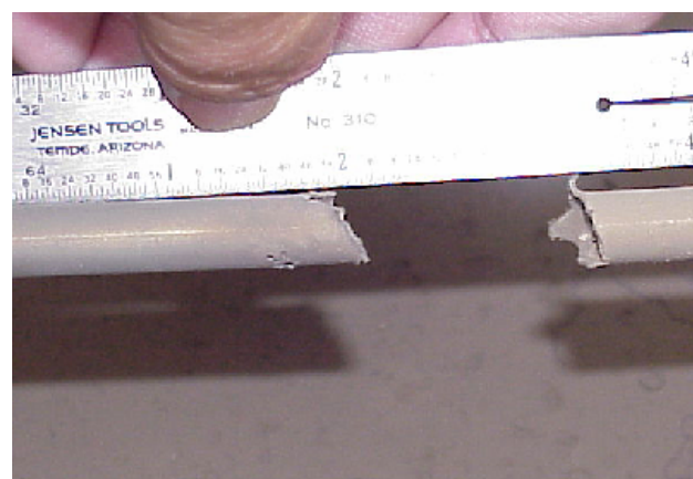
Figure 6.7 Test 2/10F Post-test Rodlet
