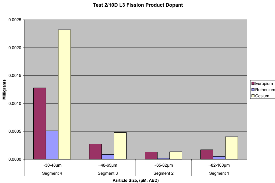
Figure A2.10D.68 Test 2/10D LPS L3 Fission Product Dopant Distribution, mg
