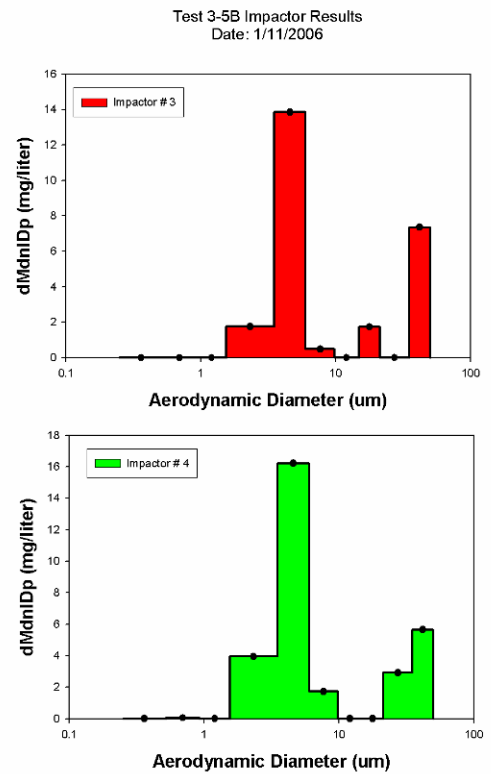
Figure A3.5B.17 Test 3/2 (A) Marple #3 Size Distribution
