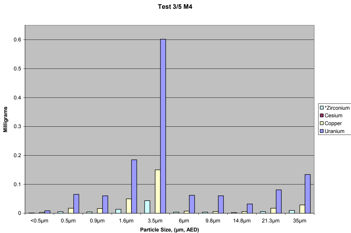
Figure A3.5B.27 Test 3/5 (B) Marple M4 Metals Analysis Distribution, mg
