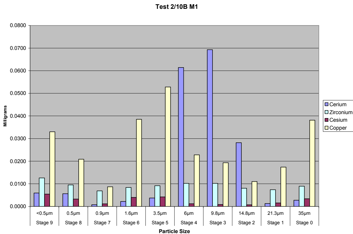
Figure A2.10B.27 Test 2/10B Marple #1 Metals Analysis Distribution, mg
