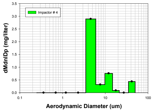
Figure A2.10B.24 Test 2/10B Marple #3 Size Distribution
