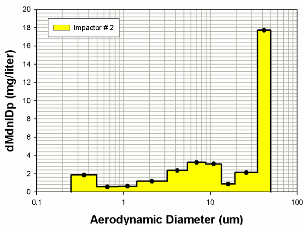
Figure A2.10C.39 Test 2/10C Marple #1 Size Distribution
