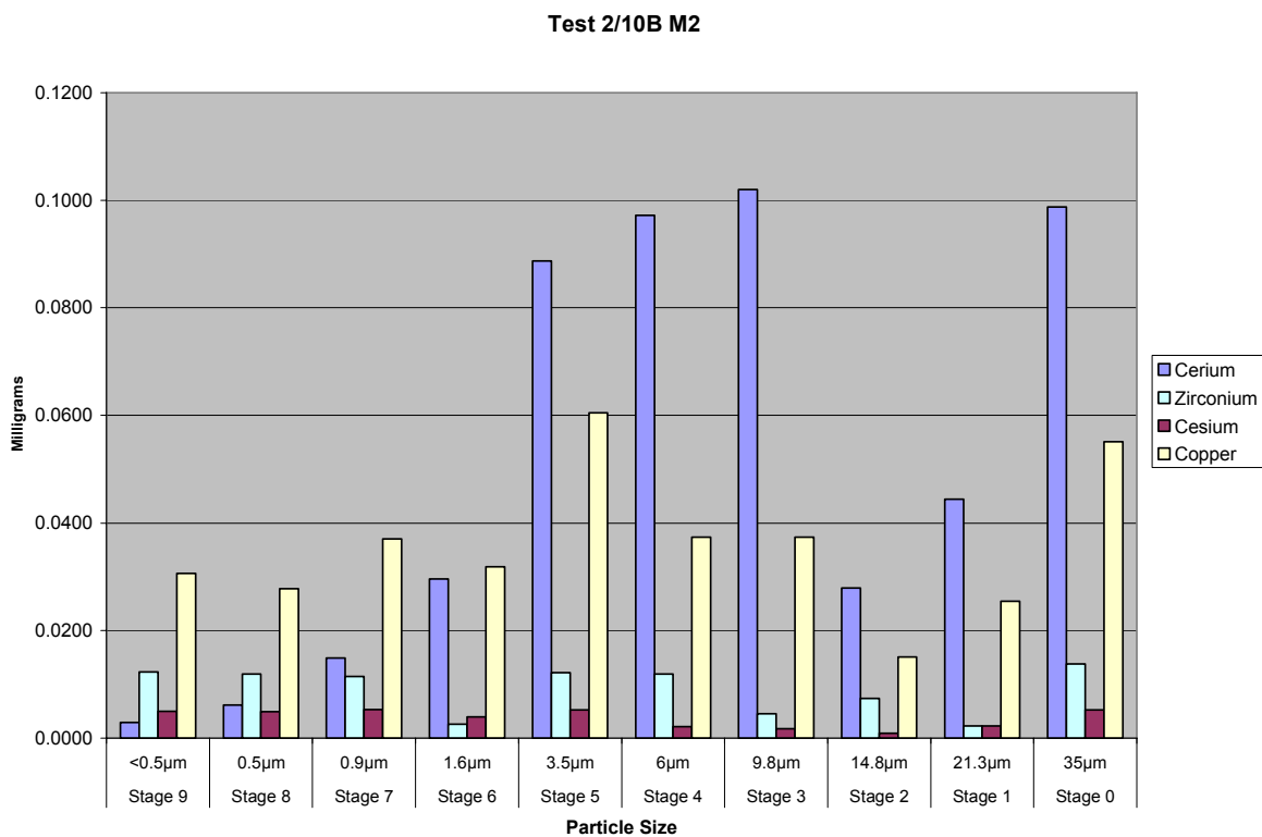
Figure A2.10B.31 Test 2/10B Marple #2 Metals Analysis Distribution, mg
