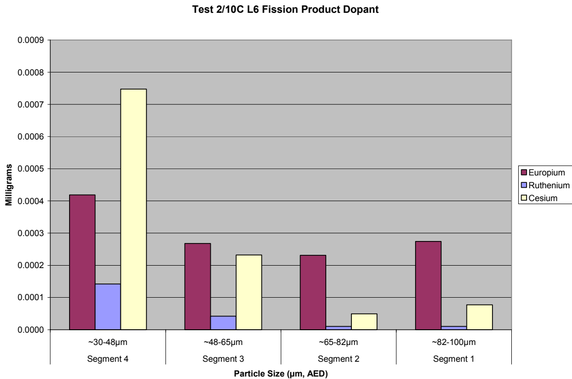
Figure A2.10C.57 Test 2/10C LPS L6 Fission Product Dopant Distribution, mg
