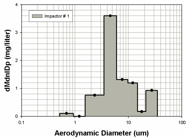
Test 2-10F Impactor Results Date: 08/18/2005
