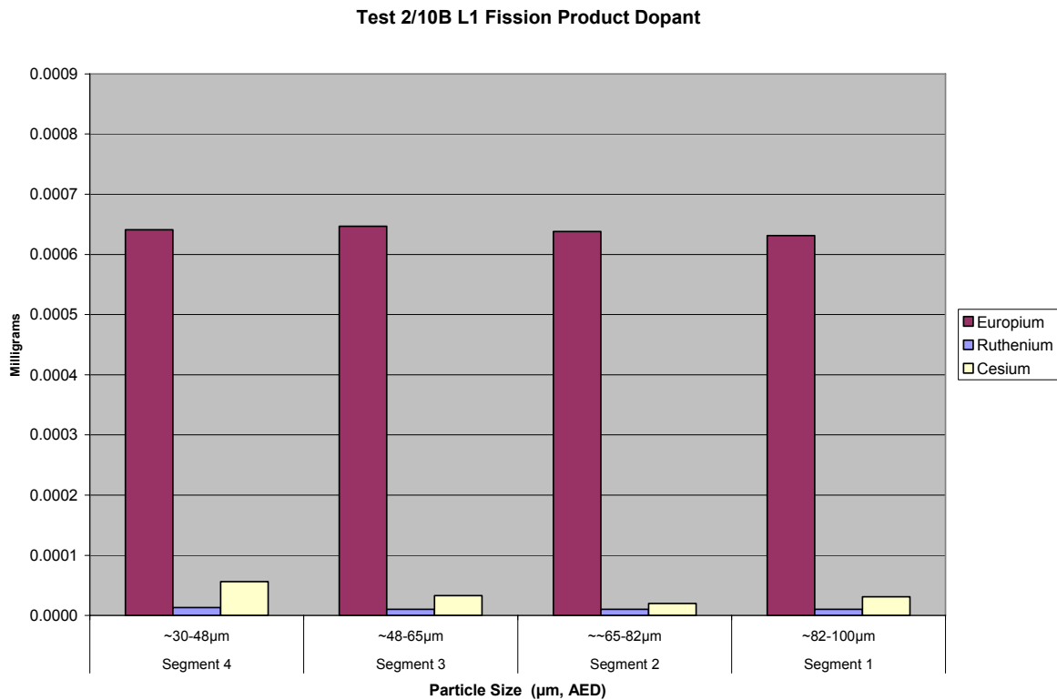
Figure A2.10B.30 Test 2/10B LPS #1 Fission Product Dopant Distribution, mg
