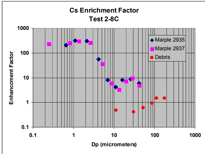
Figure 7.7 Differential Cesium EF, Test 2/8C
