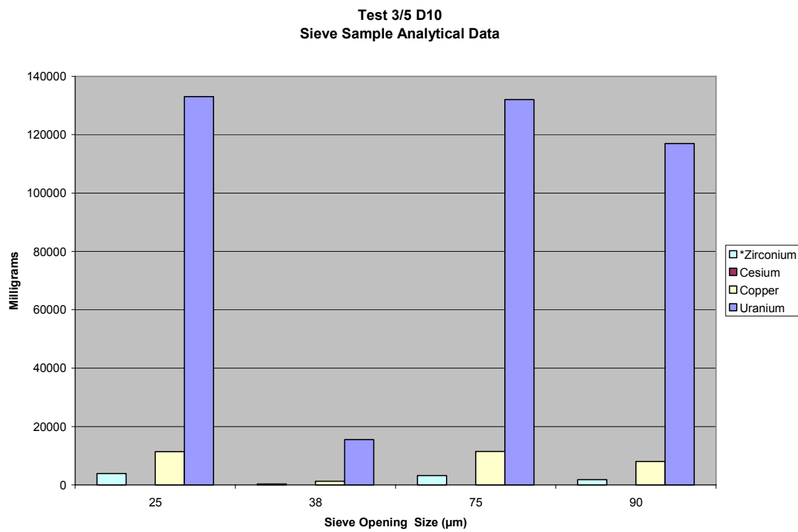
Figure A3.5B.20 Test 3/5 (B) Metals Weight Percent Distribution, Impact Debris Fractions
