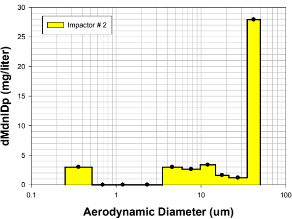
Figure A2.10B.22 Test 2/10B Marple #1 Size Distribution
