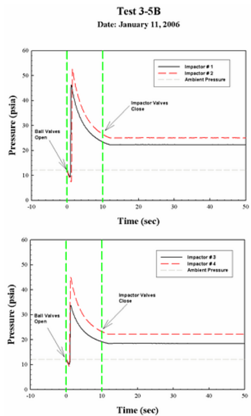
Figure 6.39 Test 3/5 (B) Aerosol Sampler Pressures
