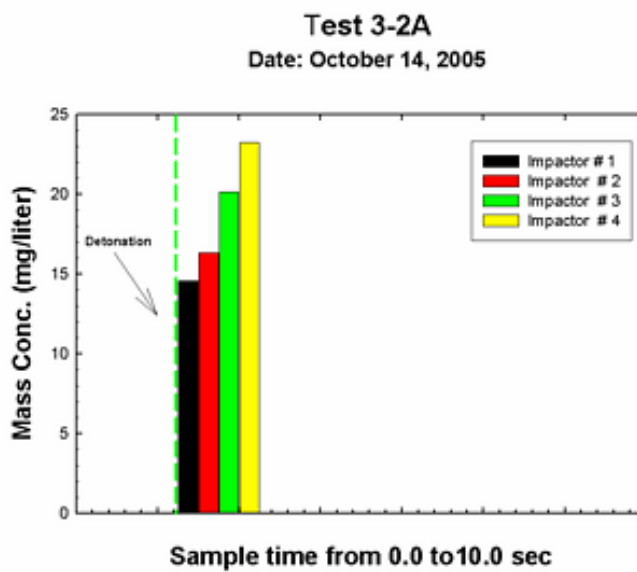
Figure A3.2A.5 Test 3/2 (A) Marple Impactor Mass Concentration Data
