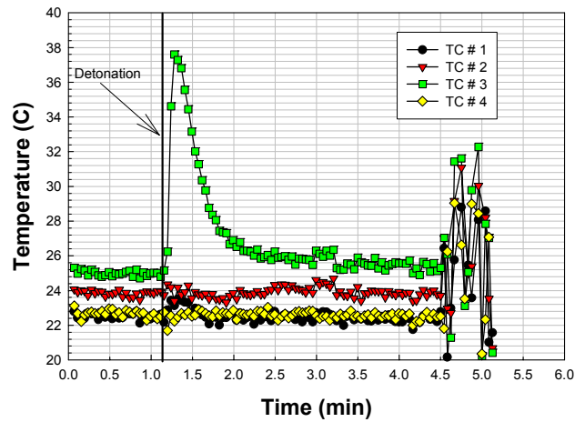
Figure 6.22 Test 2/9A Aerosol Sampler Pressures and Temperatures
