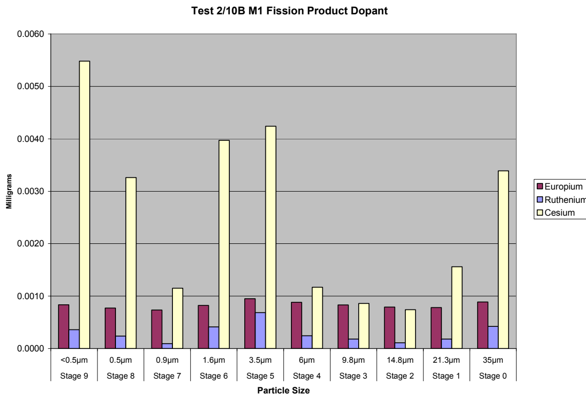
Figure A2.10B.28 Test 2/10B Marple #1 Fission Product Dopant Distribution, mg
