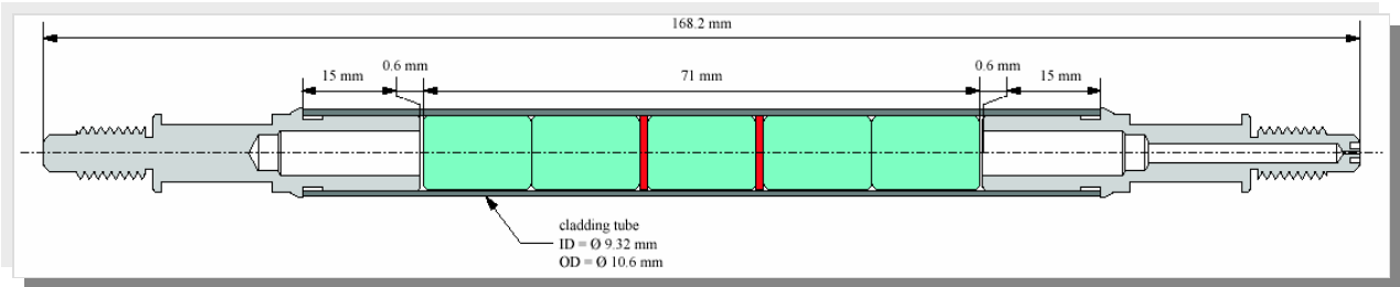
Figure 5.2 Schematic of Phase 3 DUO 2 Test Rodlet, DUR-4
