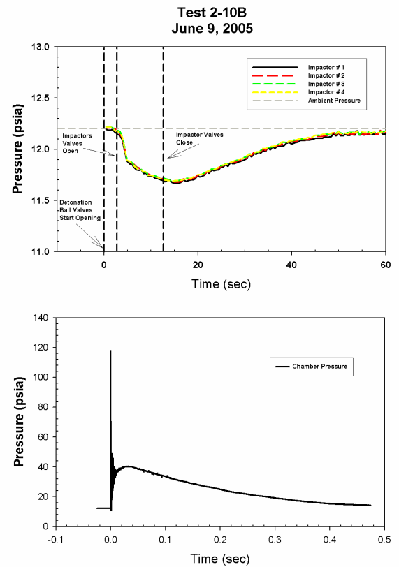
Figure 6.27 Test 2/10B Measured Pressures
