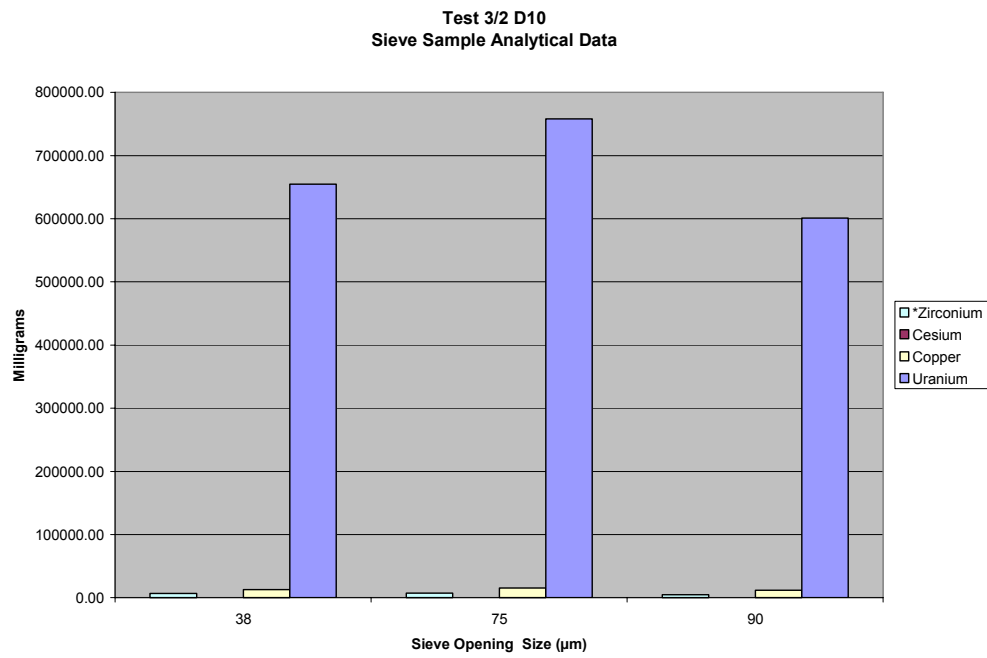
Figure A3.2A.6 Test 3/2 (A) Metals Weight Percent Distribution, Impact Debris Fractions
