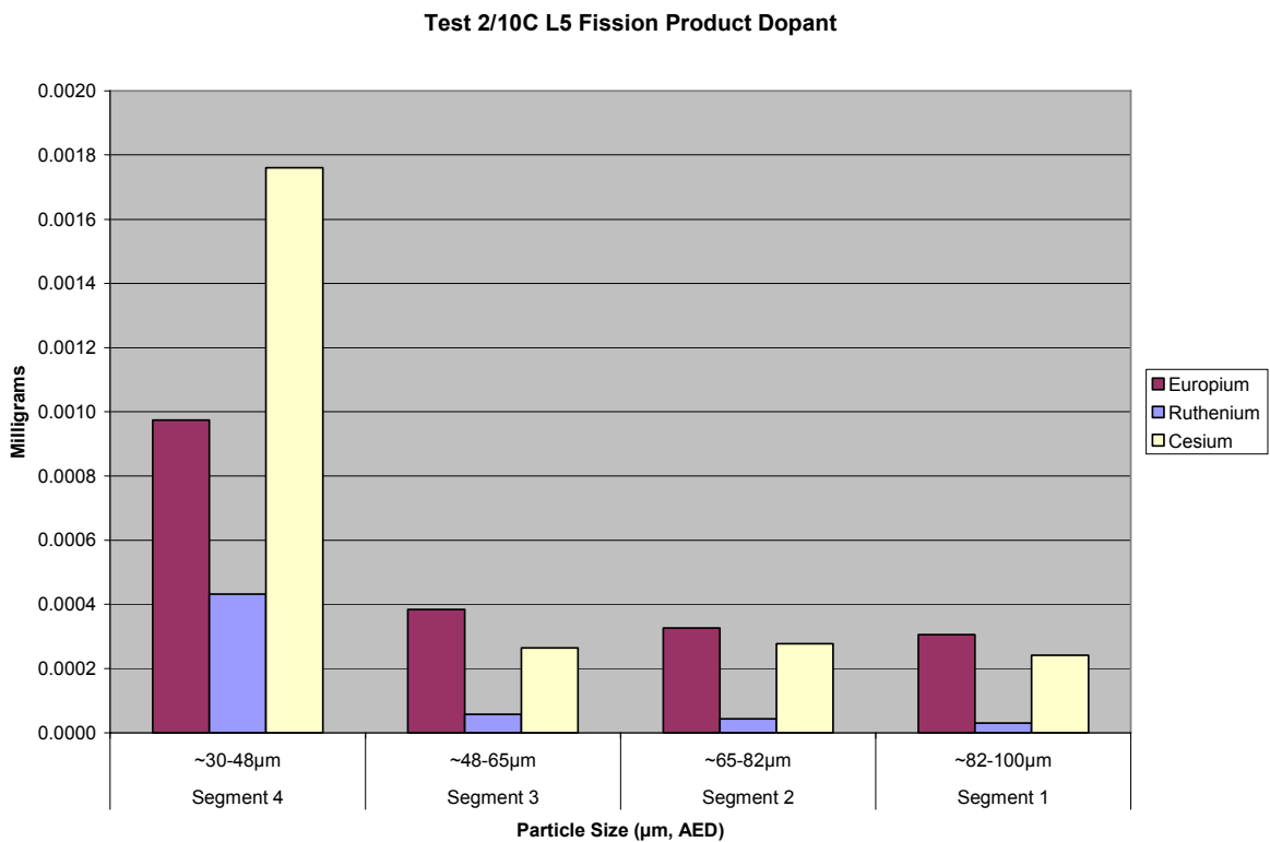
Figure A2.10C.53 Test 2/10C LPS L5 Fission Product Dopant Distribution, mg
