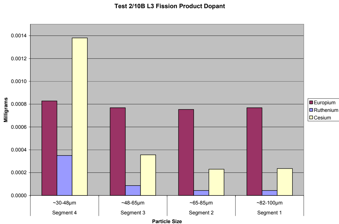
Figure A2.10B.38 Test 2/10B LPS #3 Fission Product Dopant Distribution, mg
