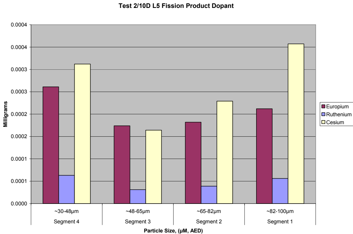
Figure A2.10D.72 Test 2/10D LPS L5 Fission Product Dopant Distribution, mg
