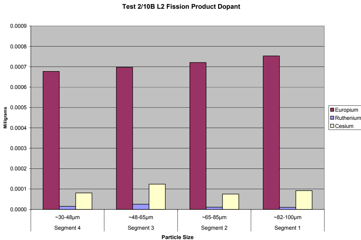
Figure A2.10B.34 Test 2/10B LPS #2 Fission Product Dopant Distribution, mg
