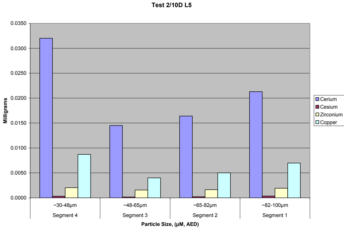
Figure A2.10D.71 Test 2/10D LPS L5 Metals Analysis Distribution, mg
