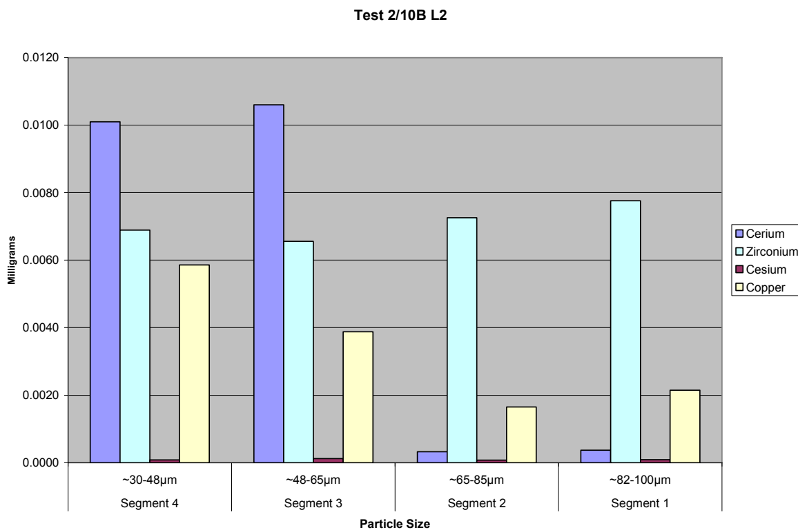
Figure A2.10B.33 Test 2/10B LPS #2 Metals Analysis Distribution, mg
