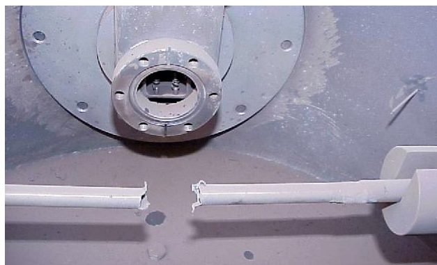
Figure 6.4 Test 2/10C Post-test Rodlet
