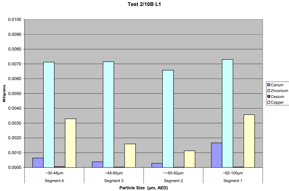
Figure A2.10B.29 Test 2/10B LPS #1 Metals Analysis Distribution, mg
