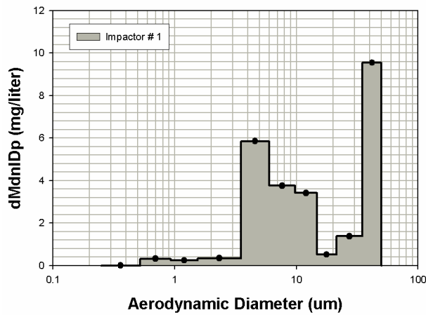
Test 2-10D Impactor Results Date: 07/27/2005
