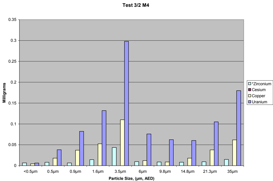
Figure A3.2A.13 Test 3/2 (A) Marple M4 Metals Analysis Distribution, mg
