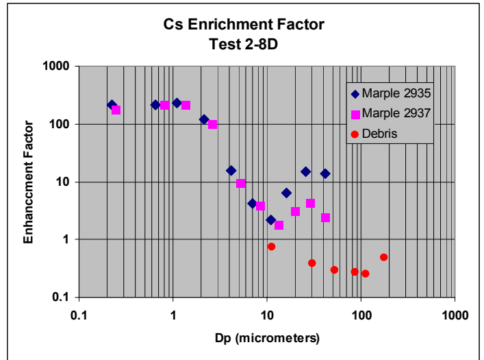
Figure 7.8 Differential Cesium EF, Test 2/8D
