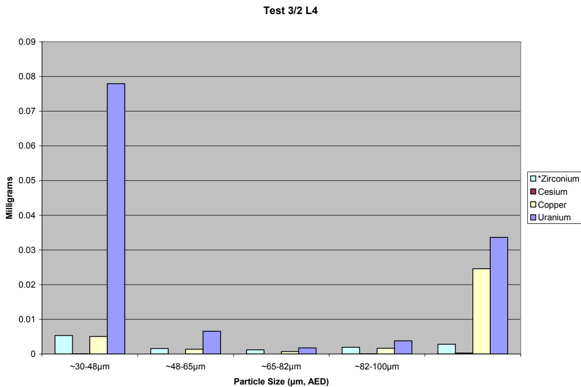
Figure A3.2A.14 Test 3/2 (A) LPS L4 Metals Analysis Distribution, mg
