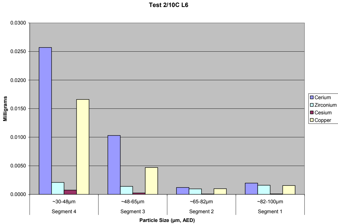
Figure A2.10C.56 Test 2/10C LPS L6 Metals Analysis Distribution, mg
