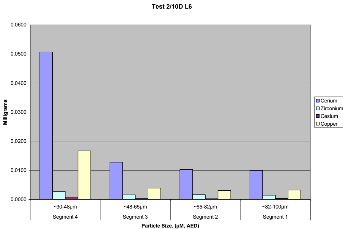
Figure A2.10D.75 Test 2/10D LPS L6 Metals Analysis Distribution, mg
