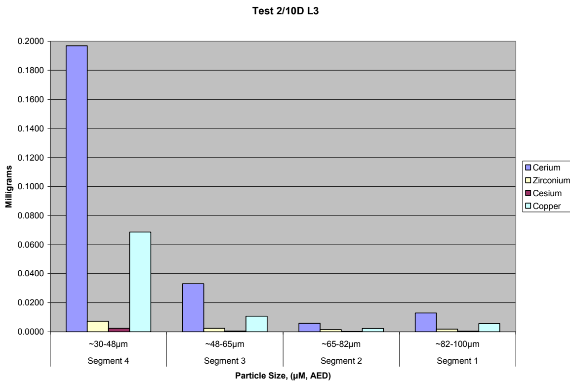
Figure A2.10D.67 Test 2/10D LPS L3 Metals Analysis Distribution, mg
