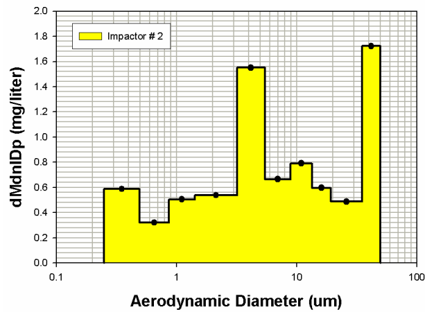
Figure A2.10F.82 Test 2/10F Marple #1 Size Distribution
