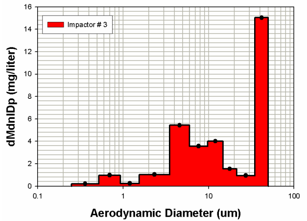
Test 2-10D Impactor Results Date: 07/27/2005
