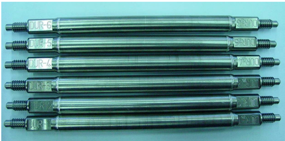
Figure 5.1 Photograph of Phase 3 \text{DUO}_2 Test Rodlets
