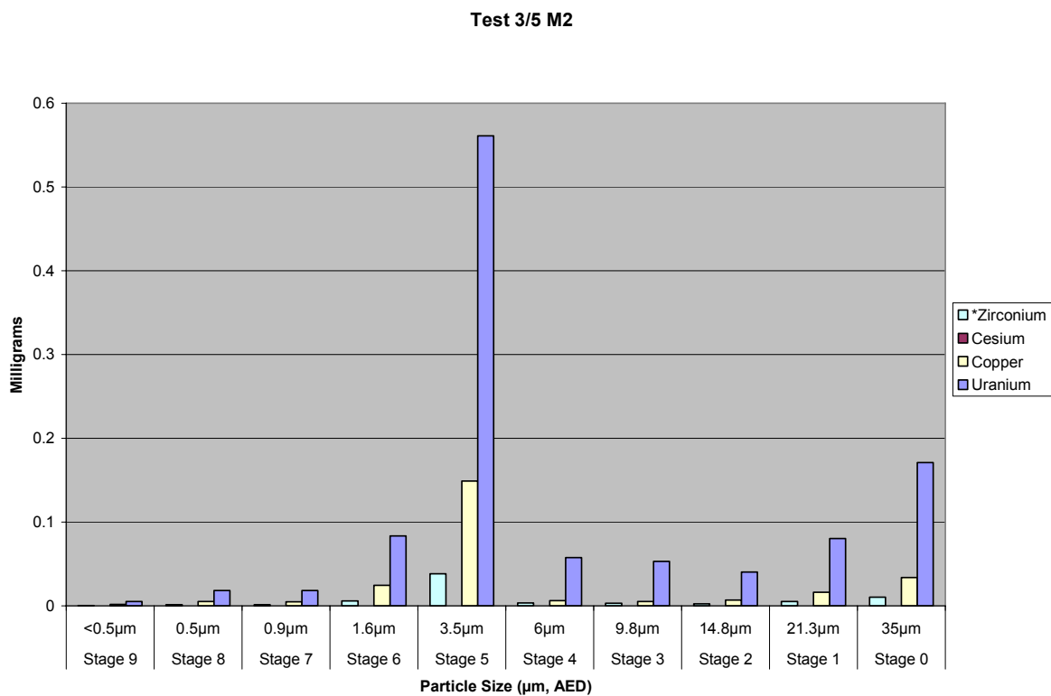
Figure A3.5B.23 Test 3/5 (B) Marple M2 Metals Analysis Distribution, mg
