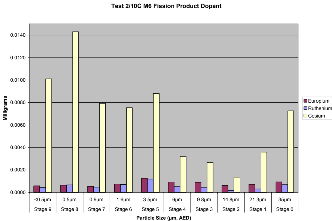
Figure A2.10C.55 Test 2/10C Marple M6 Fission Product Dopant Distribution, mg
