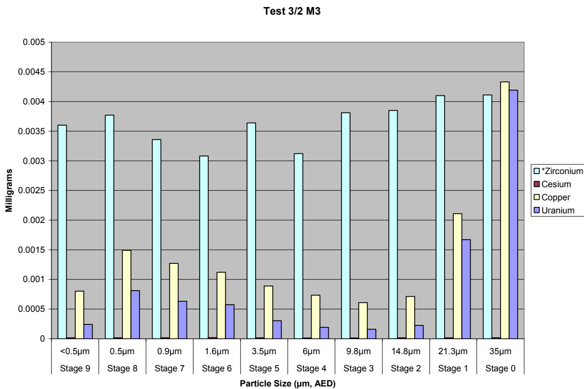
Figure A3.2A.11 Test 3/2 (A) Marple M3 Metals Analysis Distribution, mg
