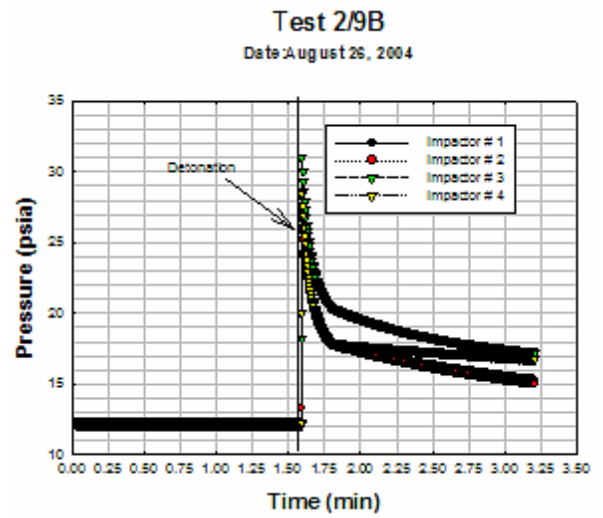
Figure 6.23 Test 2/9b Aerosol Sampler Pressures
