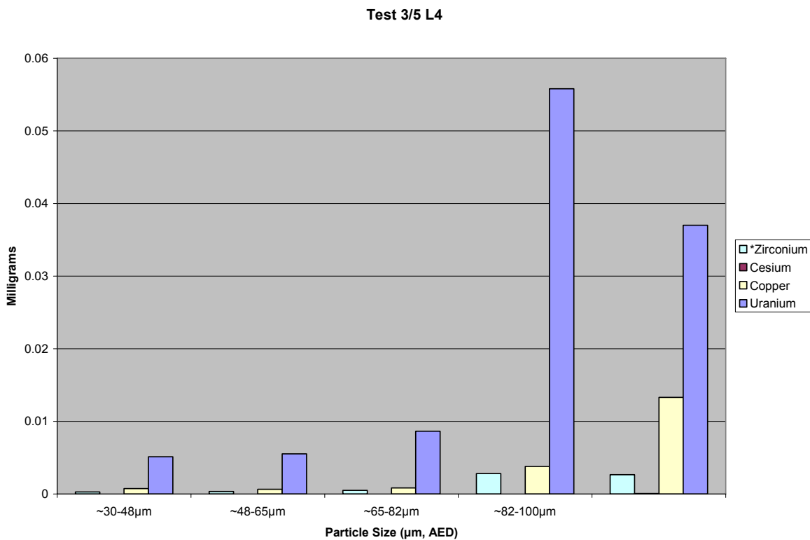
Figure A3.5B.28 Test 3/5 (B) LPS L4 Metals Analysis Distribution, mg
