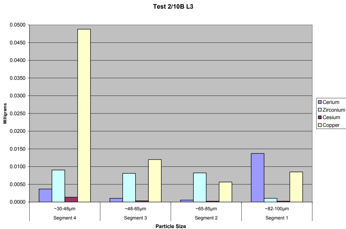
Figure A2.10B.37 Test 2/10B LPS #3 Metals Analysis Distribution, mg
