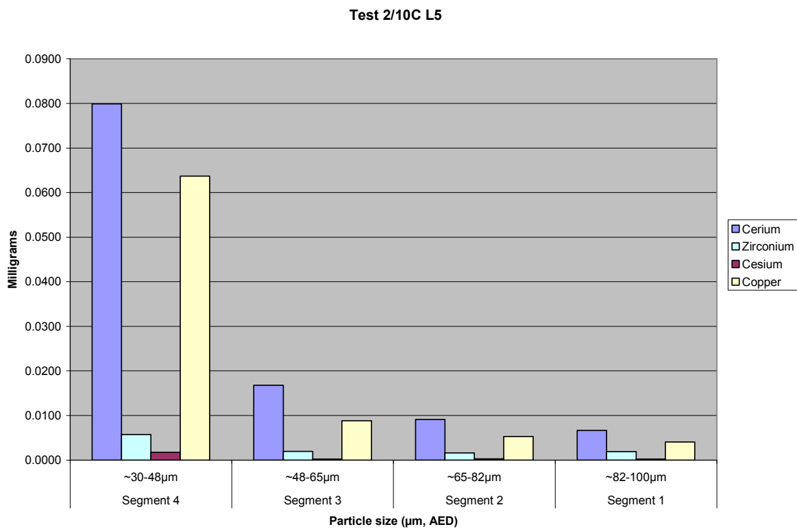
Figure A2.10C.52 Test 2/10C LPS L5 Metals Analysis Distribution, mg
