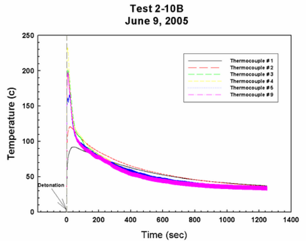
Figure 6.26 Test 2/10B Temperatures
