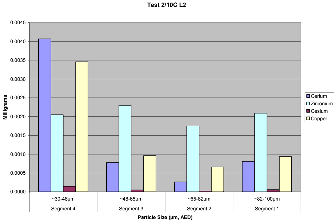
Figure A2.10C.48 Test 2/10C LPS L2 Metals Analysis Distribution, mg
