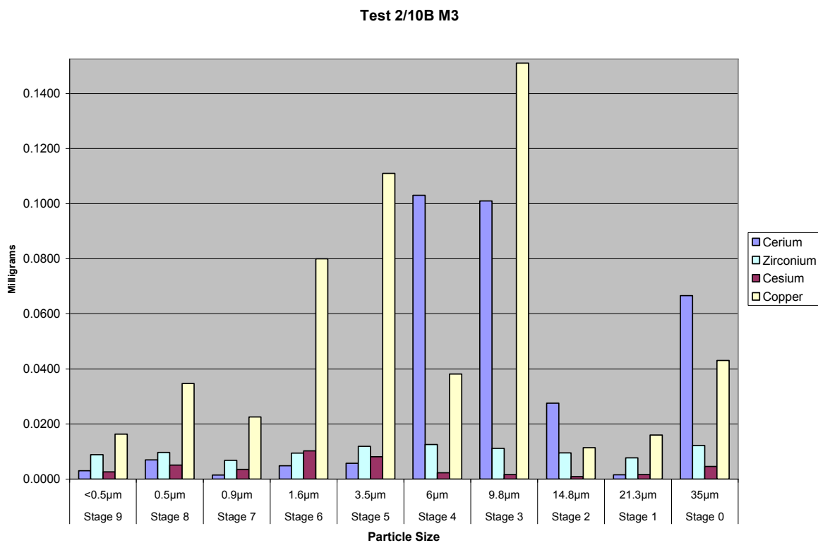
Figure A2.10B.35 Test 2/10B Marple #3 Metals Analysis Distribution, mg
