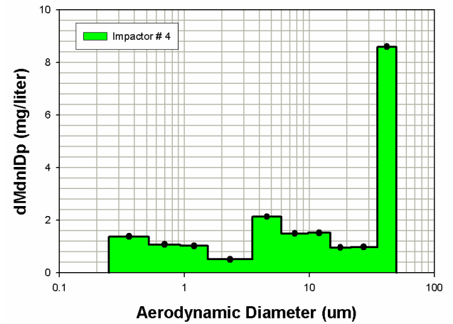
Figure A2.10F.84 Test 2/10F Marple #3 Size Distribution
