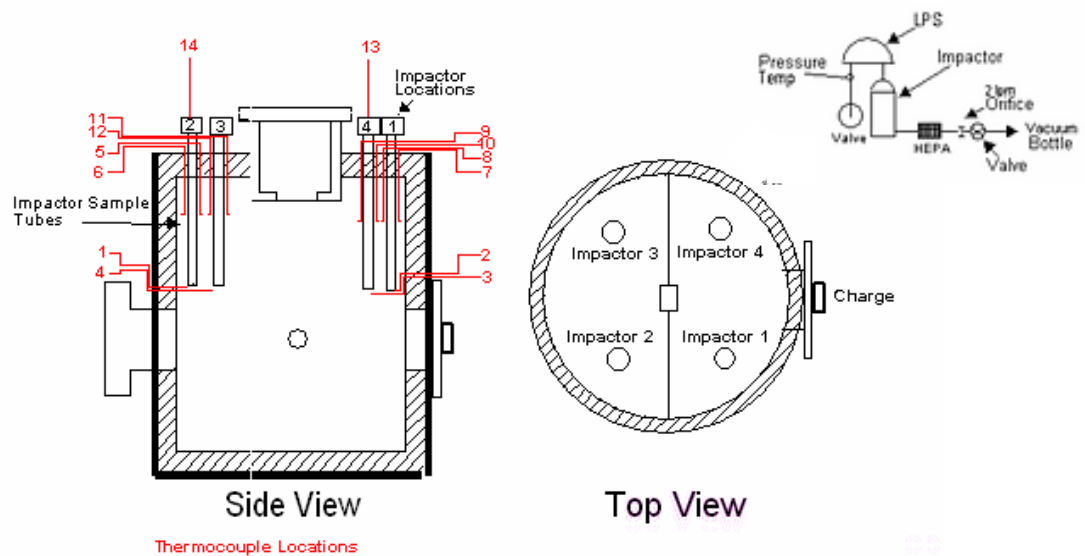
Figure 4.9 Schematic of Phase 2+ Test Chamber Instrumentation and Aerosol System
