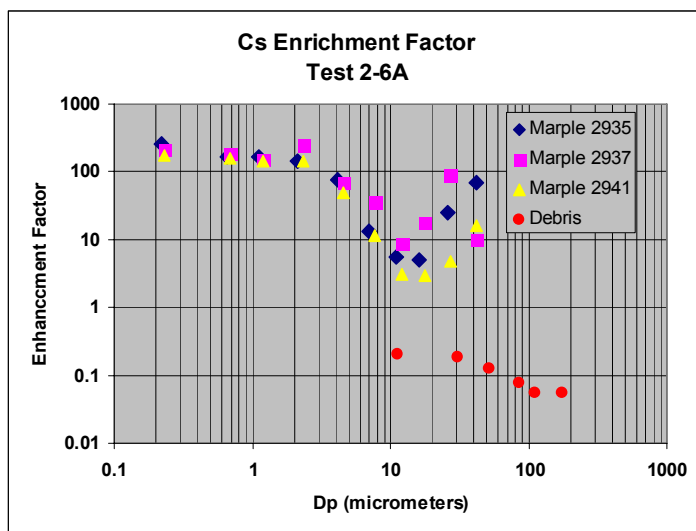
Figure 7.5 Differential Cesium EF, Test 2/6A
