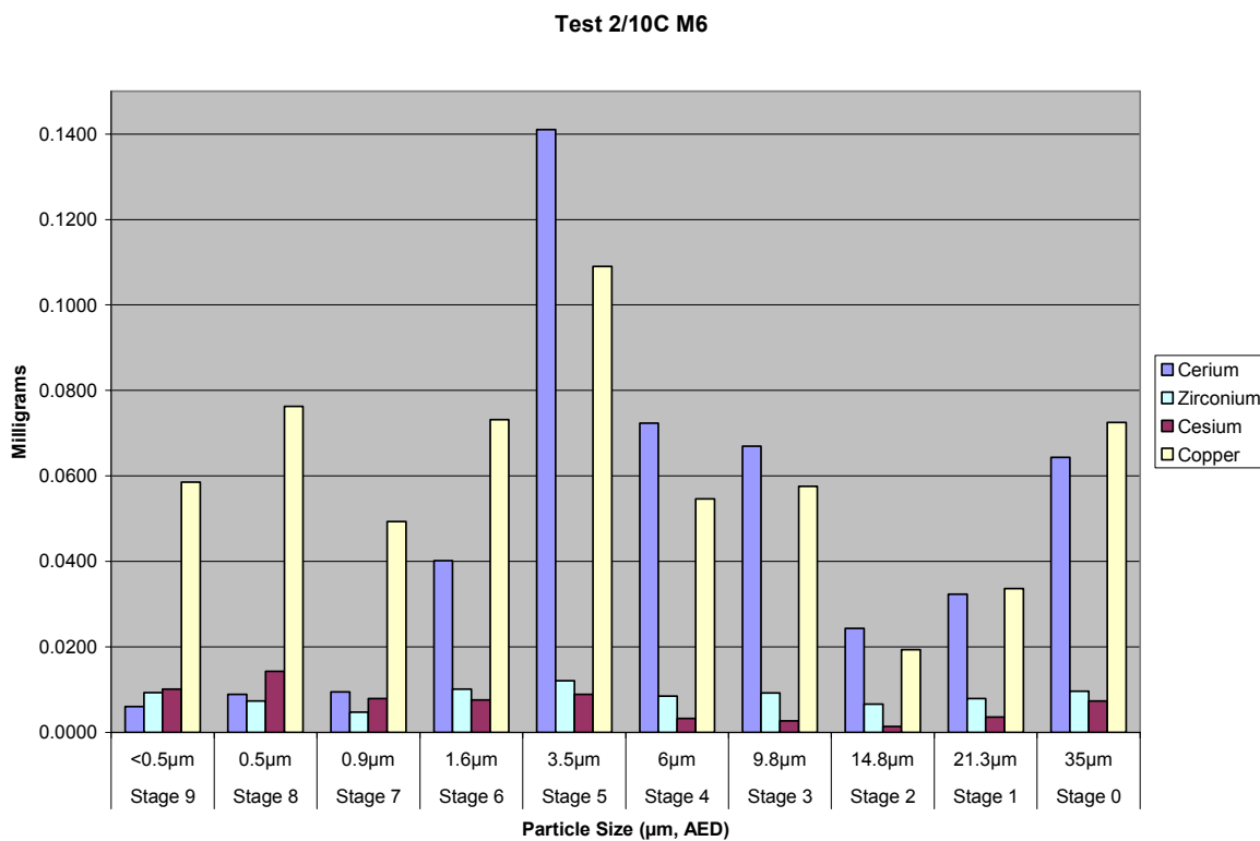
Figure A2.10C.54 Test 2/10C Marple M6 Metals Analysis Distribution, mg
