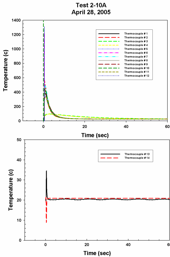
Figure 6.25 Test 2/10A Temperatures
