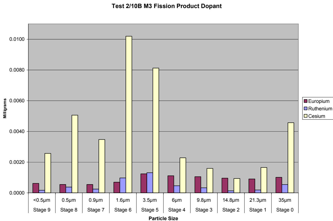
Figure A2.10B.36 Test 2/10B Marple #3 Fission Product Dopant Distribution, mg
