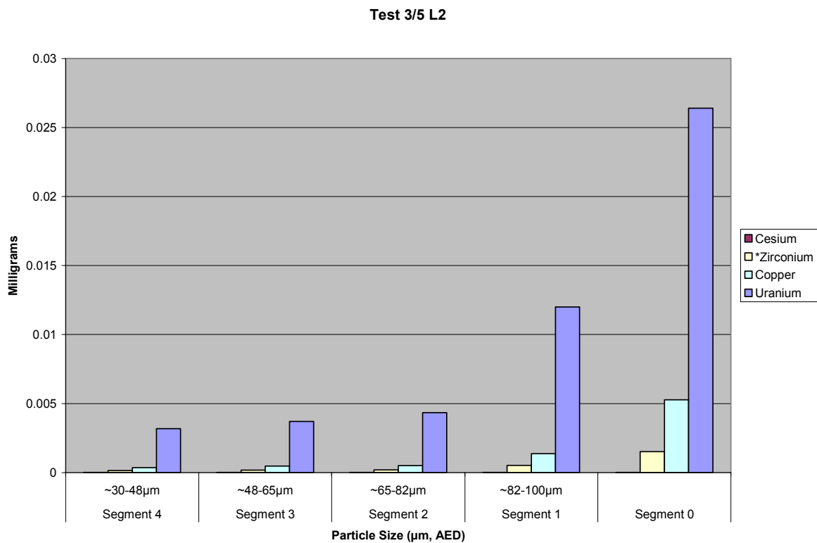
Figure A3.5B.24 Test 3/5 (B) LPS L2 Metals Analysis Distribution, mg
