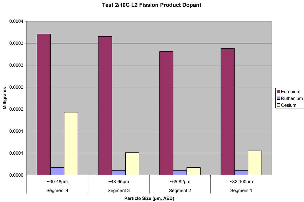
Figure A2.10C.49 Test 2/10C LPS L2 Fission Product Dopant Distribution, mg
