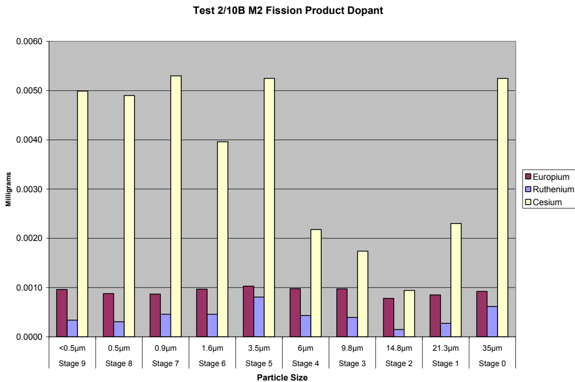
Figure A2.10B.32 Test 2/10B Marple #2 Fission Product Dopant Distribution, mg
