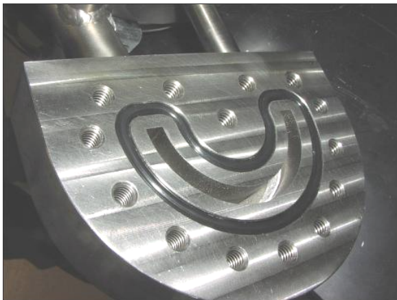
Figure 4.7 Inside of LPS Component
