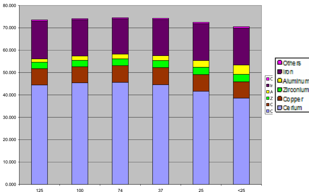
Figure A2.9A.5 Test 2/9A Weight % Distribution of Major Metals, Bottom #1 Impact Debris
