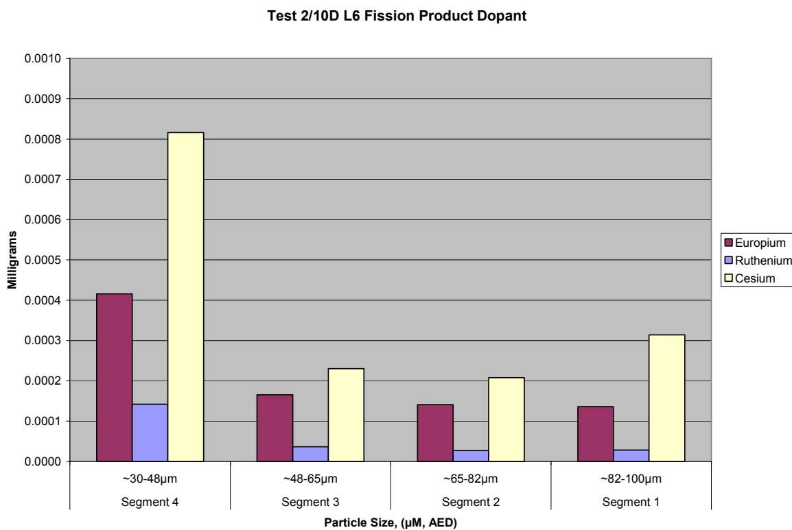
Figure A2.10D.76 Test 2/10D LPS L6 Fission Product Dopant Distribution, mg
