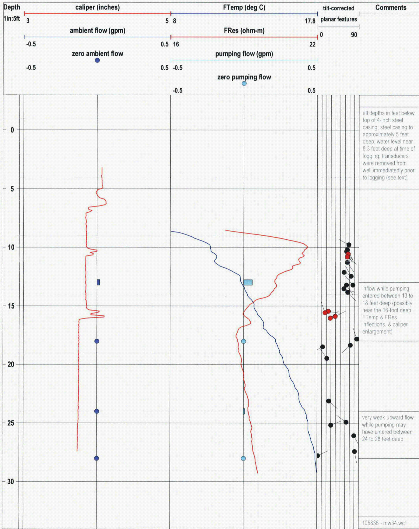
Well: GZA / Buchanan, NY - MW-34 conventional logs
