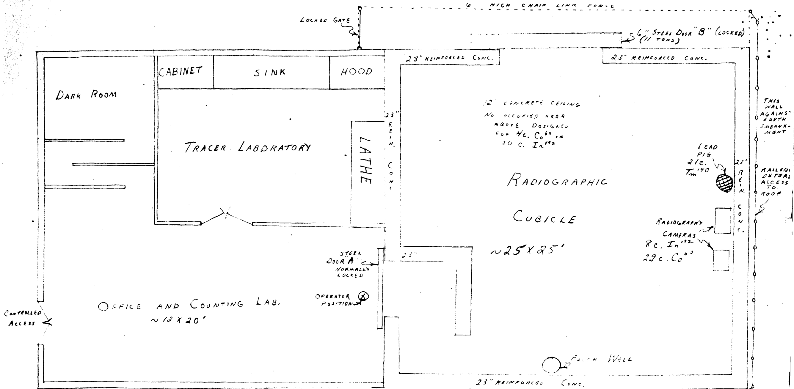
RADIOISOTOPE LAB AND ASSOCIATED FACILITIES THE MARTIN CO. BALTIMORE, MD. EXHIBIT 1.
