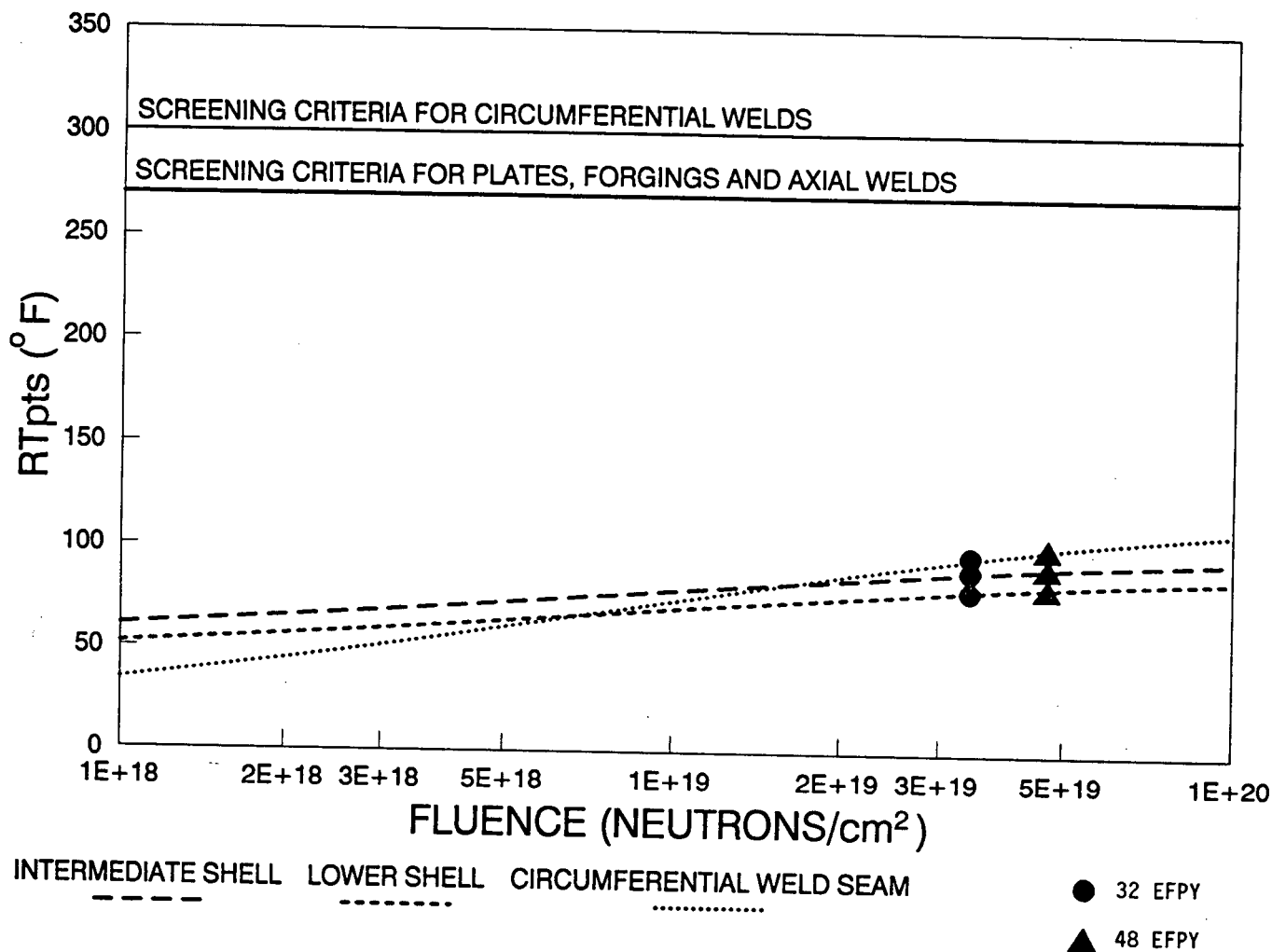
Figure 2. RT_{PTS} versus Fluence Curves for Watts Bar Unit 2 Limiting Material - Circumferential Seam Weld.
