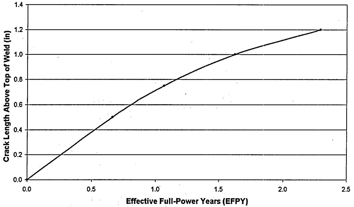
Figure 8.13 Approximate time in effective full-power years (EFPY) to grow the upper tip of a long axial crack in Nozzle 3 to various heights above the top of the weld.
