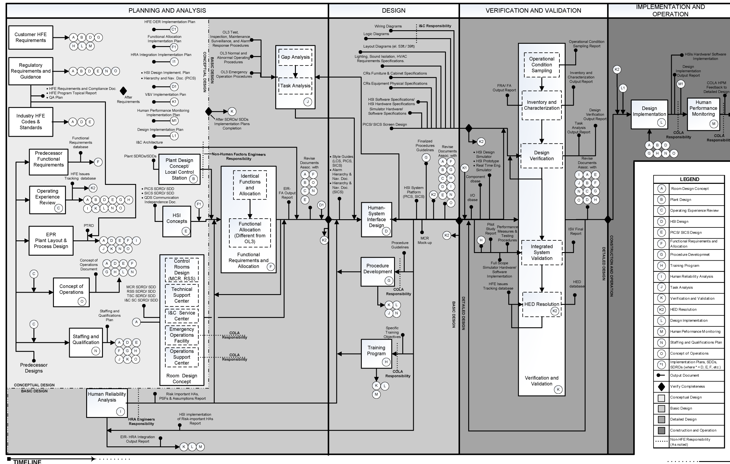
Figure 18.1-2—HFE Design Control Process
