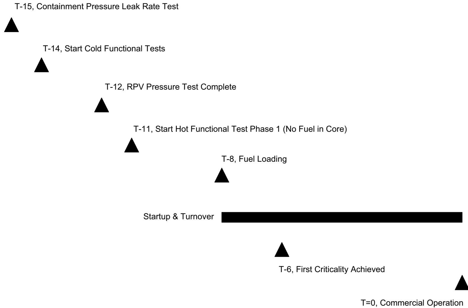
Figure 14.2-1—U.S. EPR Commissioning Milestones
