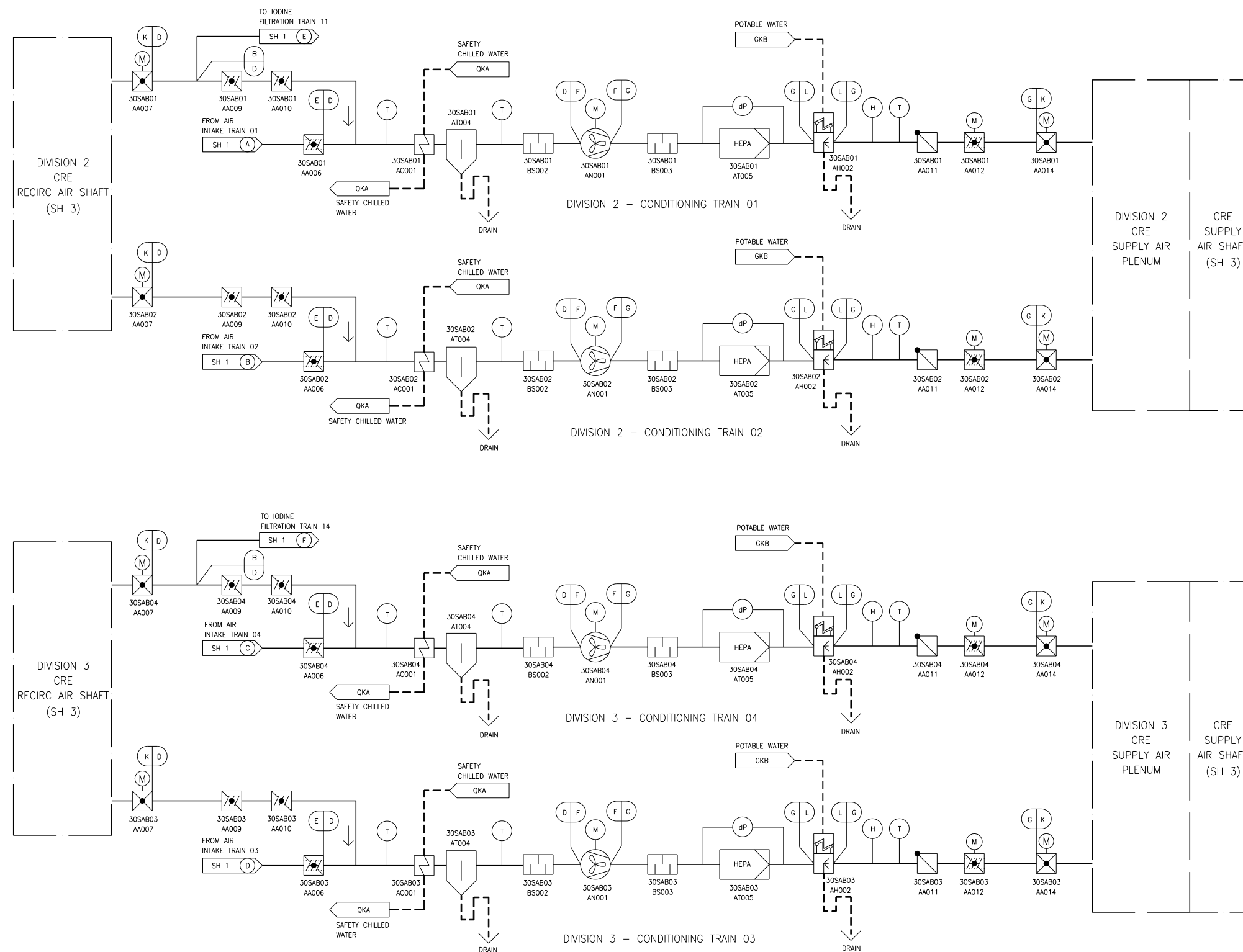
Figure 9.4.1-1—Control Room Air Intake and Iodine Filtration Train Subsystems
