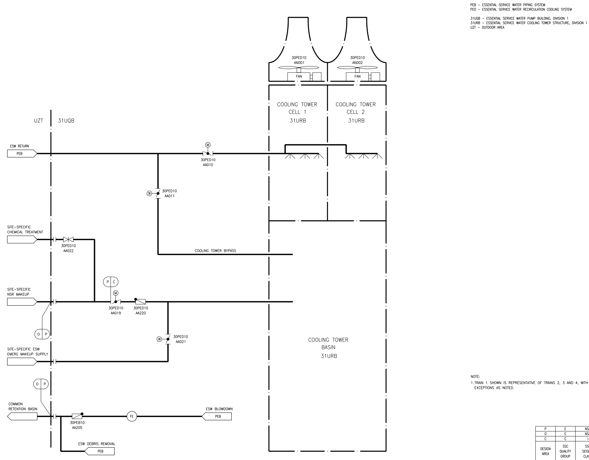
Figure 9.2.5-1—Ultimate Heat Sink Piping and Instrumentation Diagram
