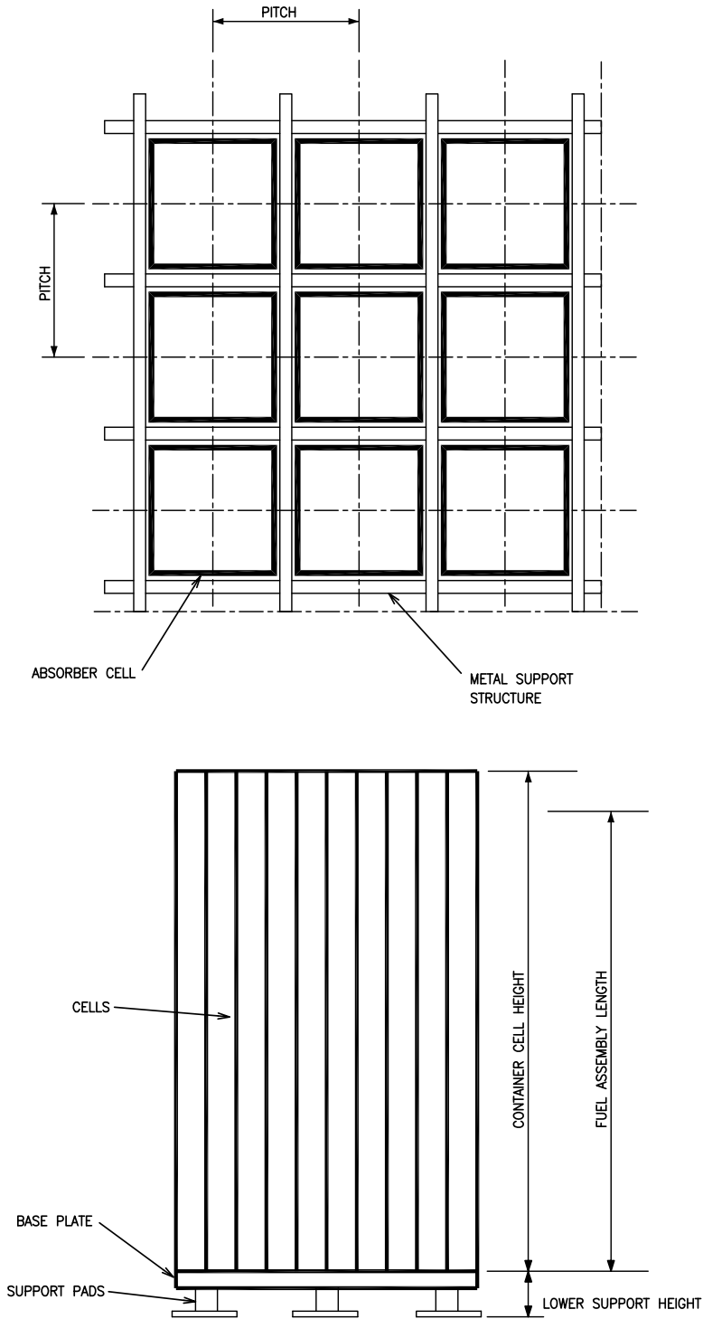
Figure 9.1.2-2—Typical New and Spent Fuel Storage Rack Cross-Sections
