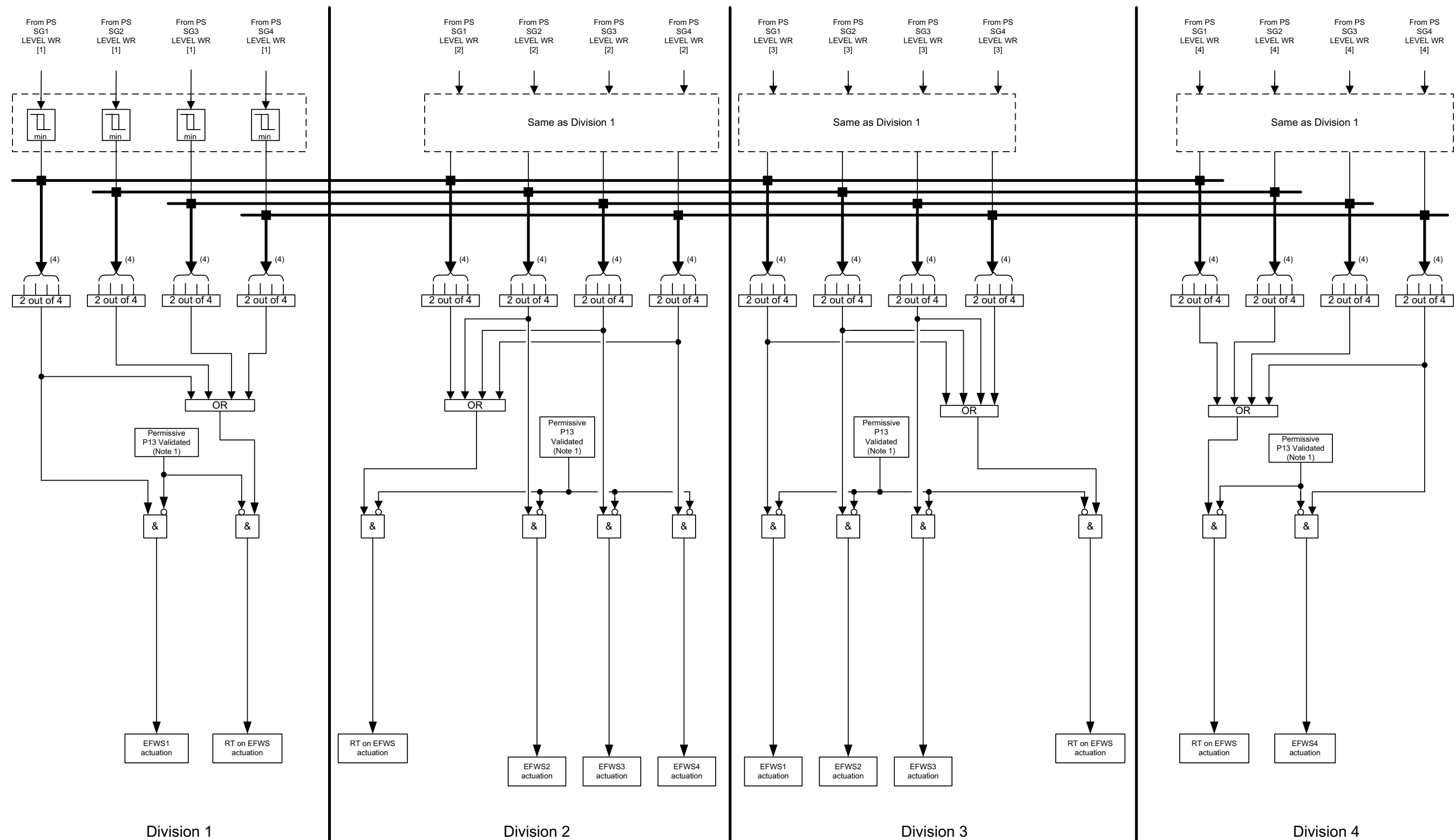
Figure 7.8-3—EFW Actuation
