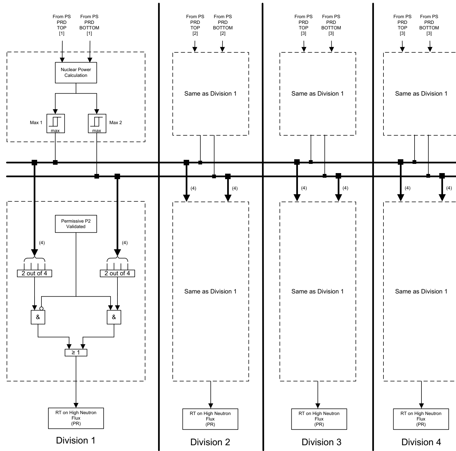
Figure 7.8-1—RT on High Neutron Flux
