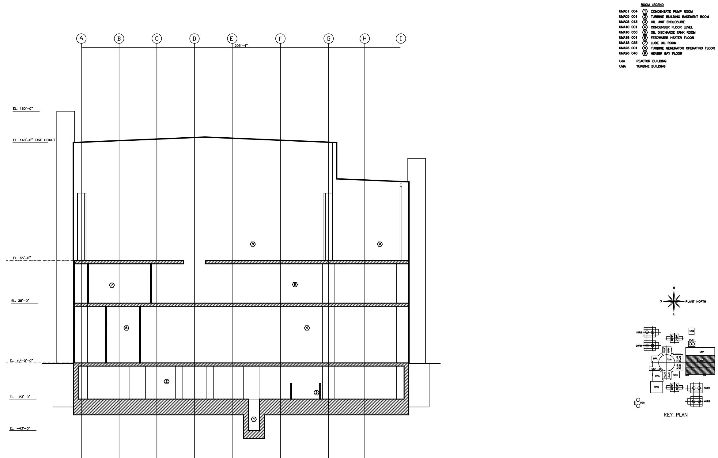
Figure 1.2-49—[[ Turbine Building General Arrangement Section C-C (Alternate) ]]
