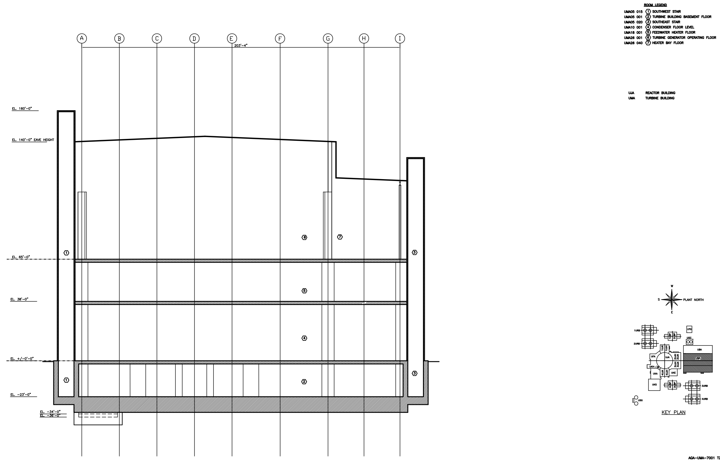
Figure 1.2-47—[[ Turbine Building General Arrangement Section B-B (Alternate) ]]
