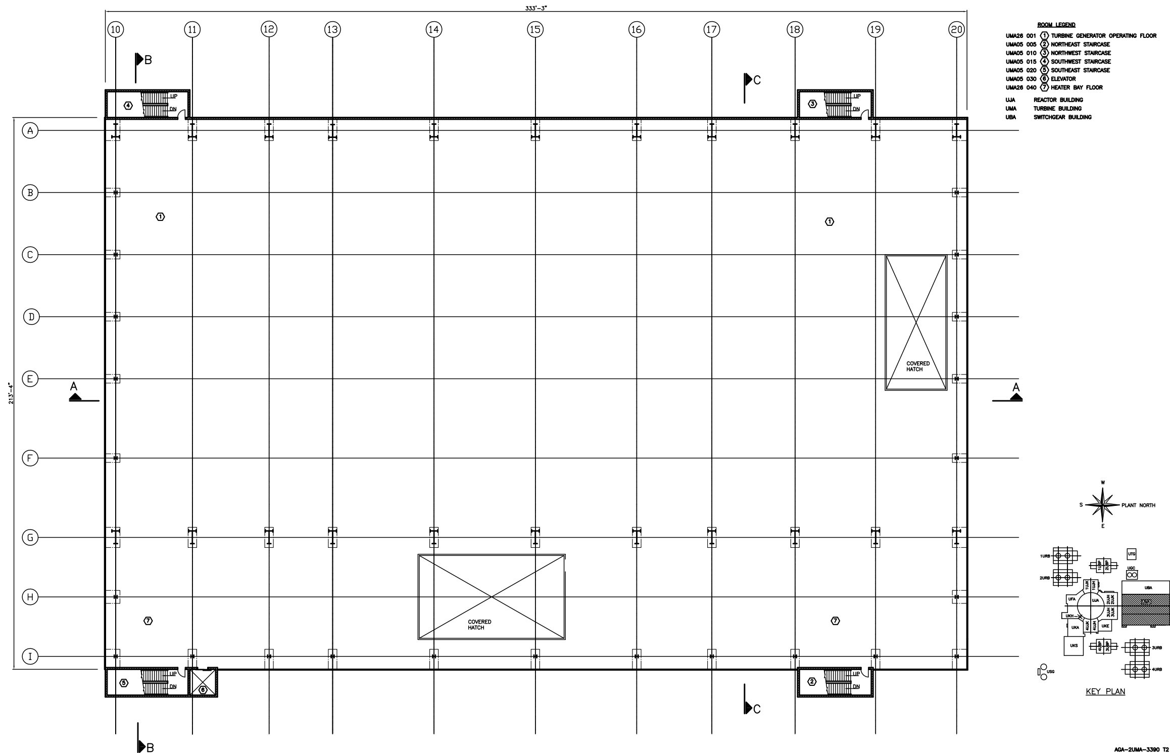
Figure 1.2-36—[[ Turbine Building General Arrangement Plan View Elevation 65'-0" ]]
