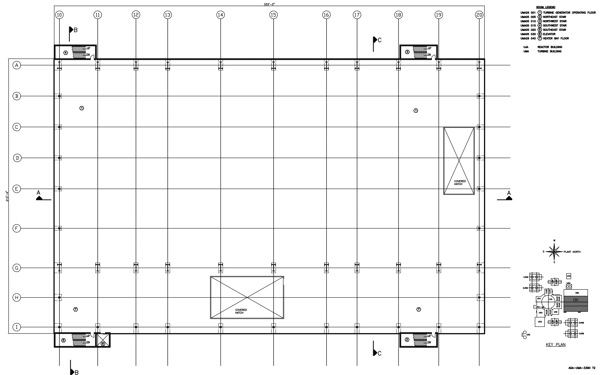
Figure 1.2-38—[[ Turbine Building General Arrangement Plan View Elevation 65'-0" (Alternate) ]]
