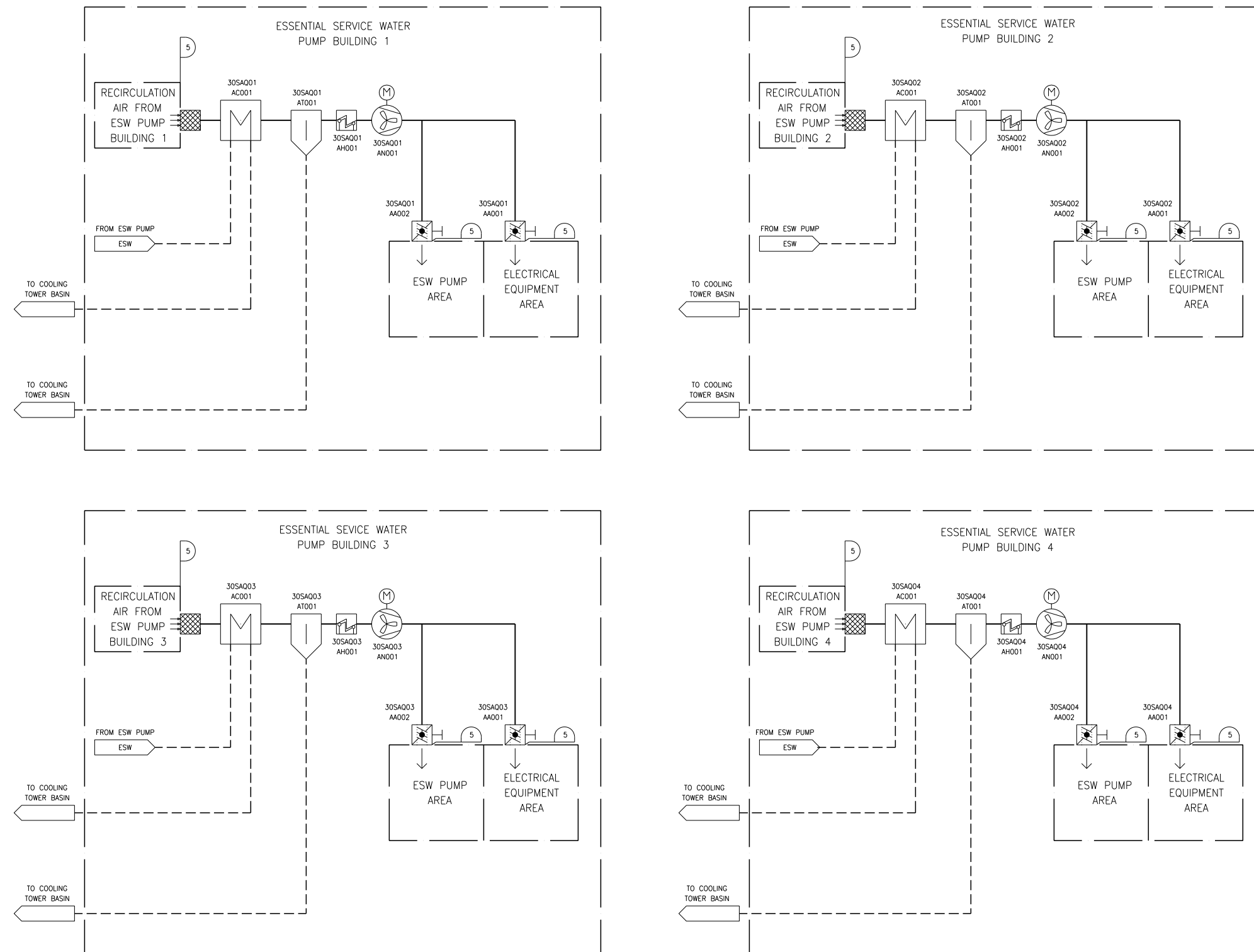
Figure 2.6.13-1—Essential Service Water Pump Building Ventilation System Functional Arrangement
