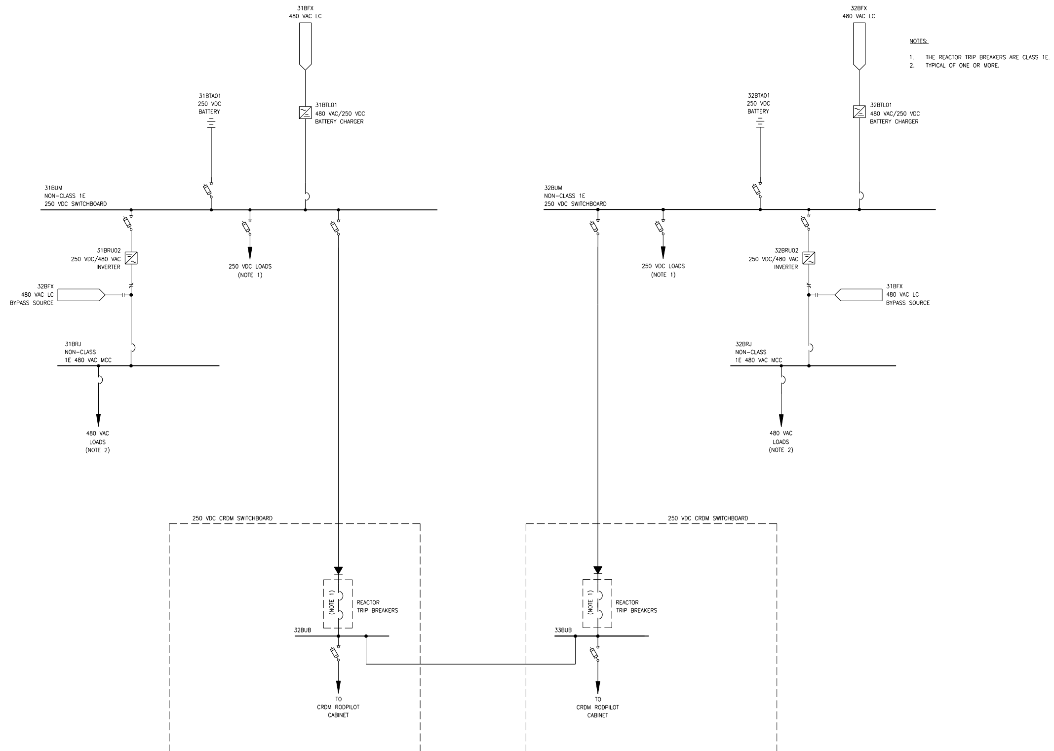
Figure 2.5.7-1—Non-Class 1E Uninterruptible Power Supply System Functional Arrangement
