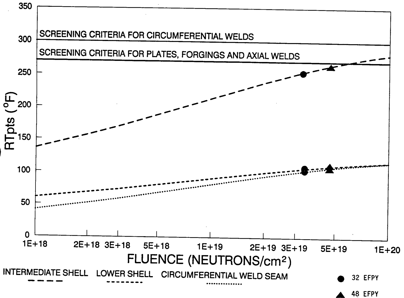
Figure 2. RT_{PTS} versus Fluence Curves for Watts Bar Unit 1 Limiting Material - Intermediate Shell Forging.
