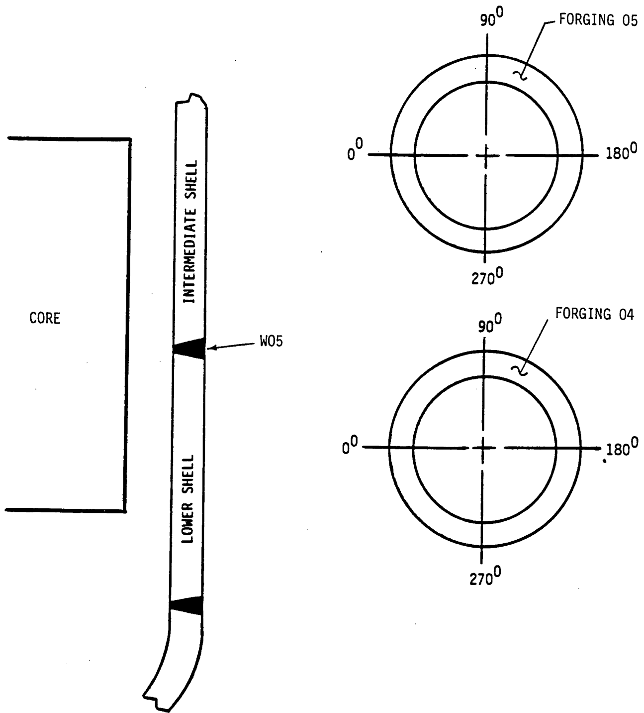
Figure 1. Identification and Location of Beltline Region Material for the Watts Bar Unit 1 Reactor Vessel
