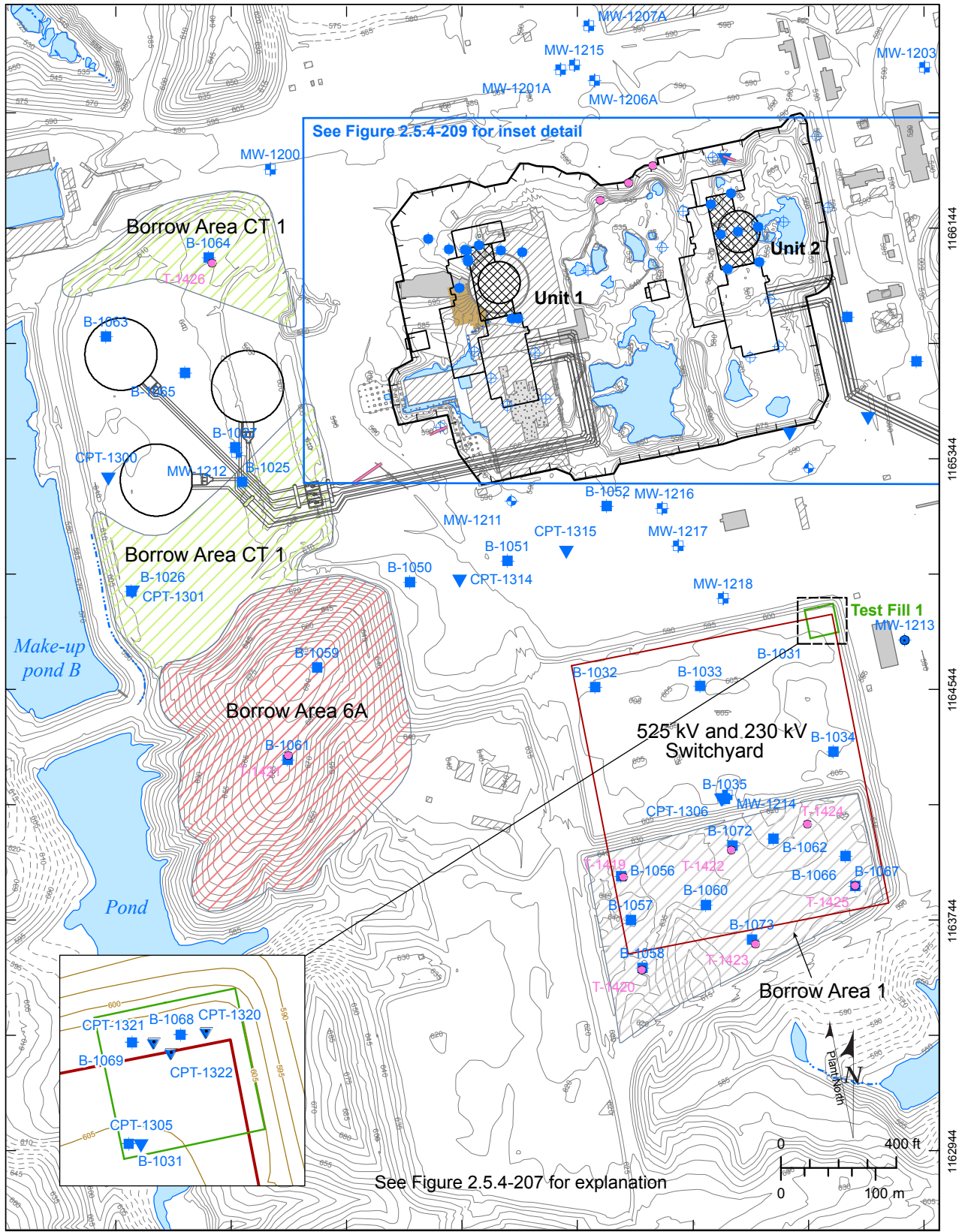
WILLIAM STATES LEE III NUCLEAR STATION UNITS 1 & 2 Potential Borrow Area Locations and Excavation Limits FIGURE 2.5.4-242 Rev 0
