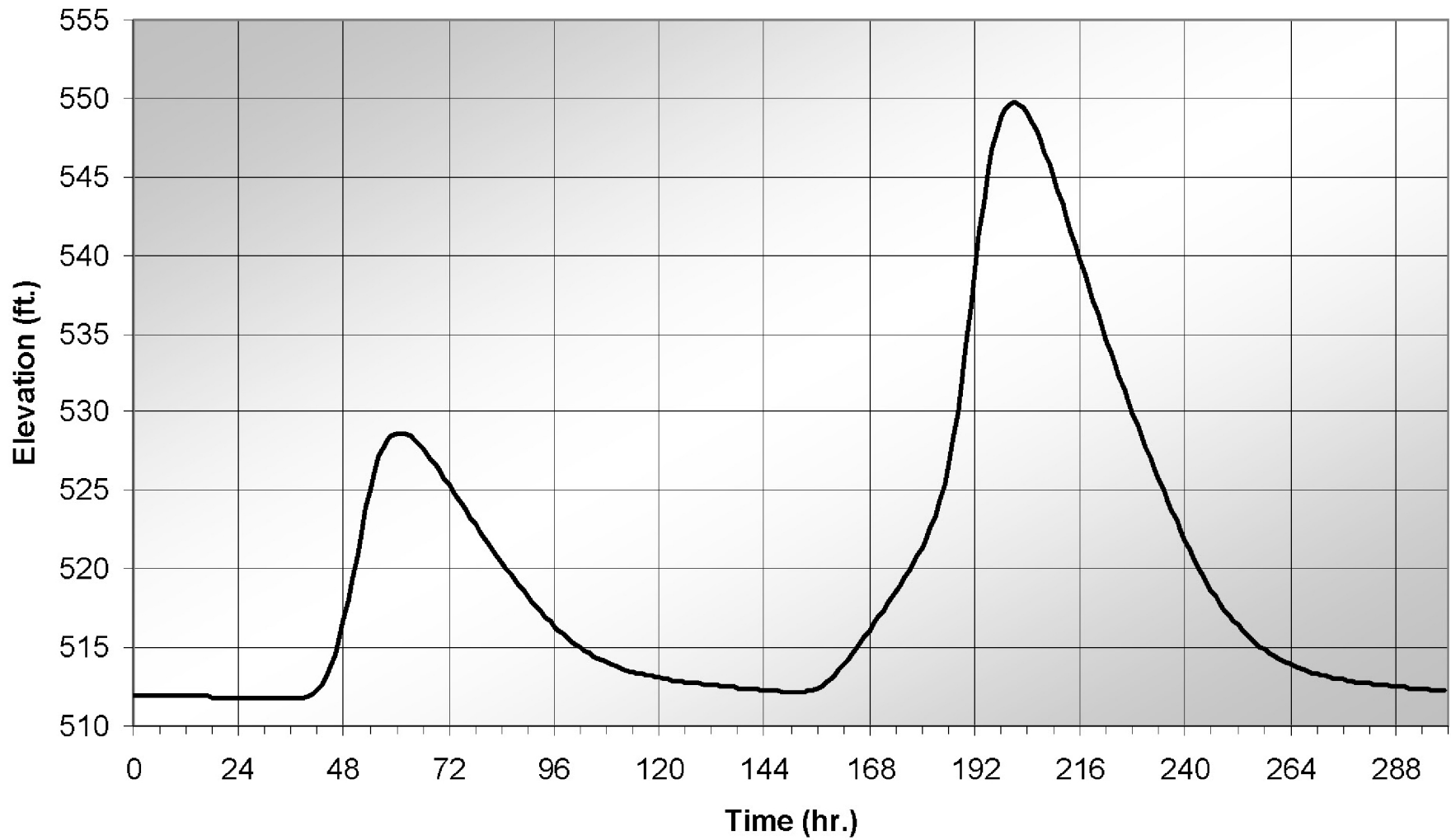
WILLIAM STATES LEE III NUCLEAR STATION UNITS 1 & 2 PMF Elevation Hydrograph, Broad River at Lee Nuclear Station FIGURE 2.4.3-229 Rev 0
