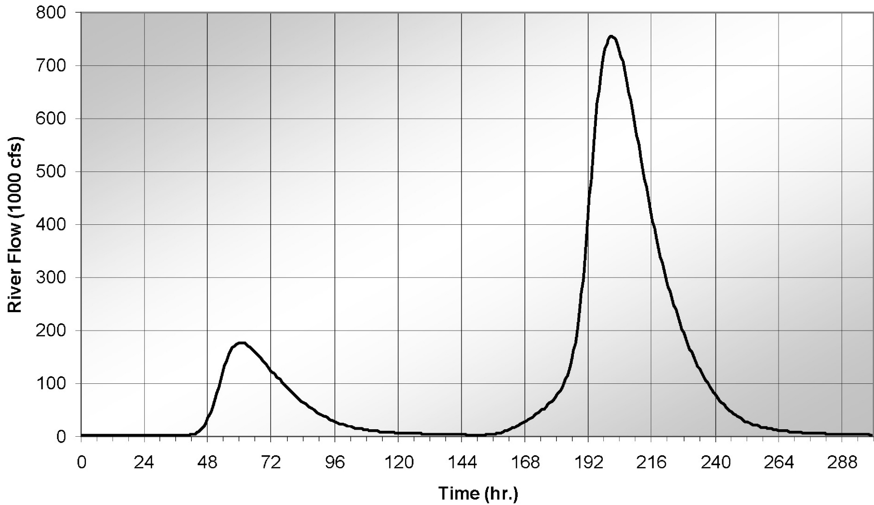
WILLIAM STATES LEE III NUCLEAR STATION UNITS 1 & 2 PMF Hydrograph, Broad River at Lee Nuclear Station FIGURE 2.4.3-226 Rev 0
