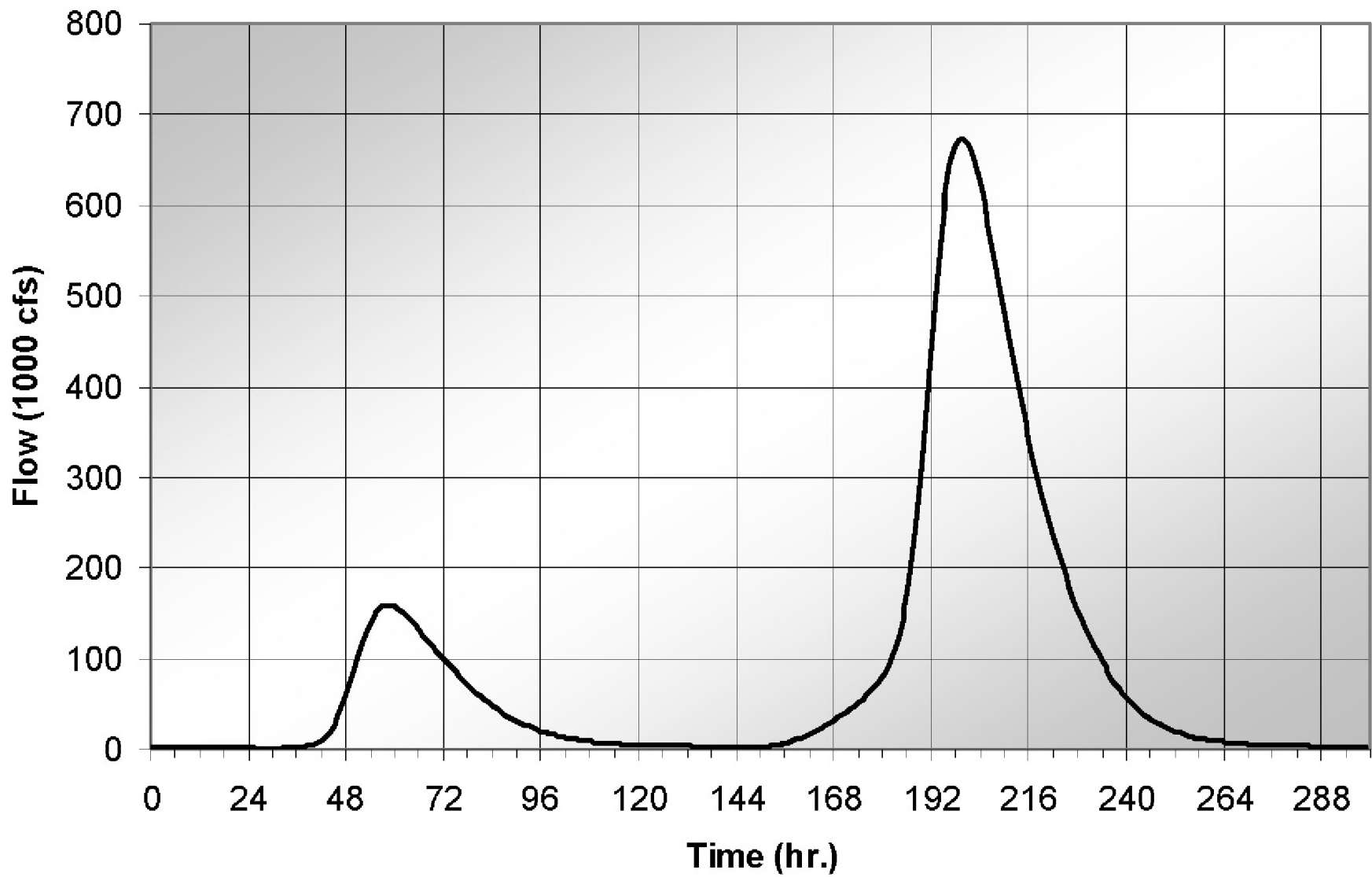
WILLIAM STATES LEE III NUCLEAR STATION UNITS 1 & 2 Gaston Shoals Dam PMF Combined Inflow Hydrograph FIGURE 2.4.3-218 Rev 0
