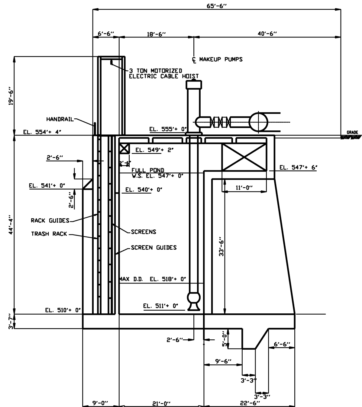
SECTION 1-1
