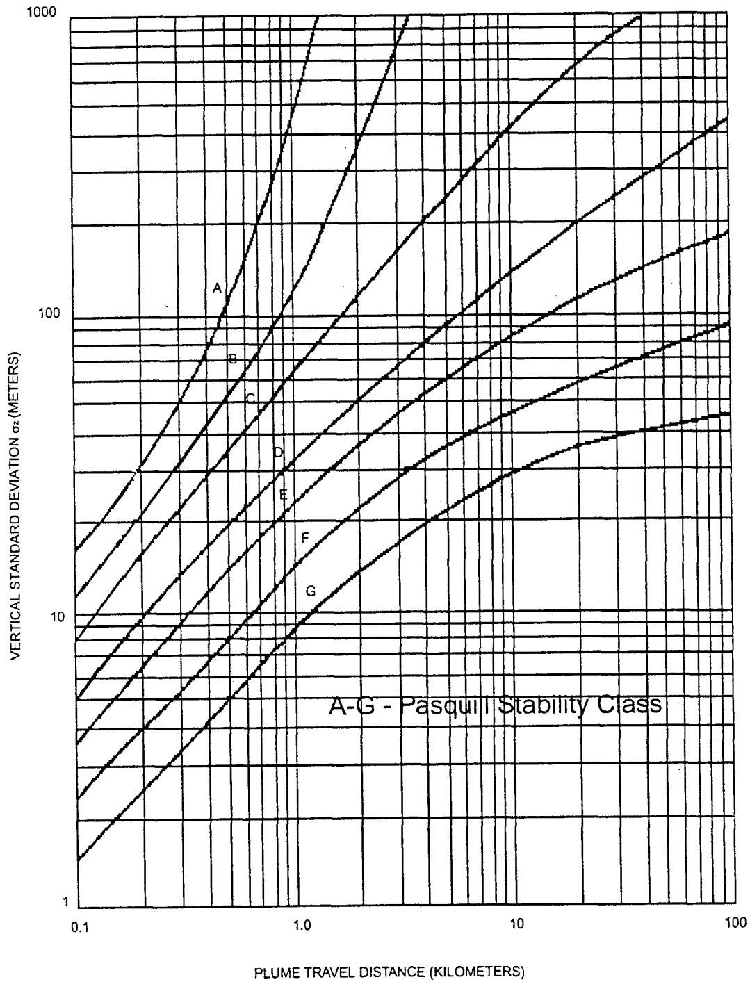
Figure 7.5 - VERTICAL STANDARD DEVIATION OF MATERIAL IN A PLUME
