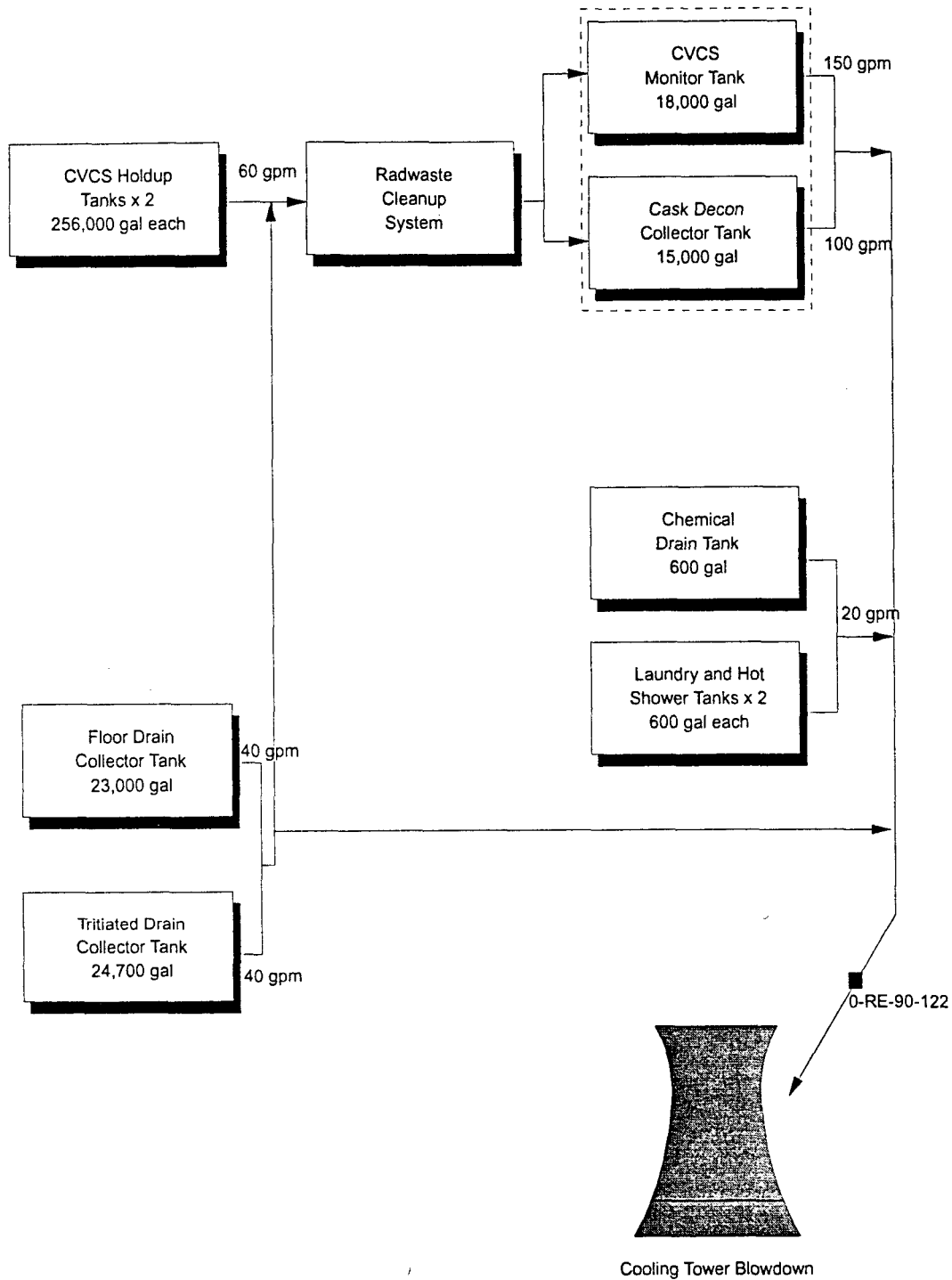
Figure 6.2 - LIQUID RADWASTE SYSTEM
