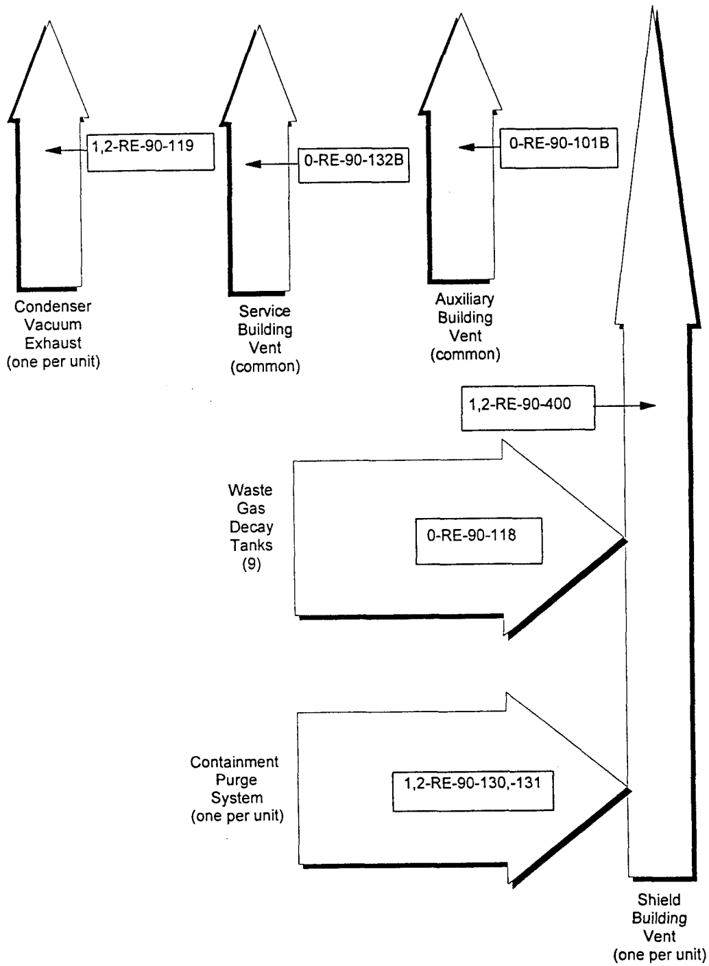
Figure 7.1 - GASEOUS EFFLUENT RELEASE/DISCHARGE POINTS
