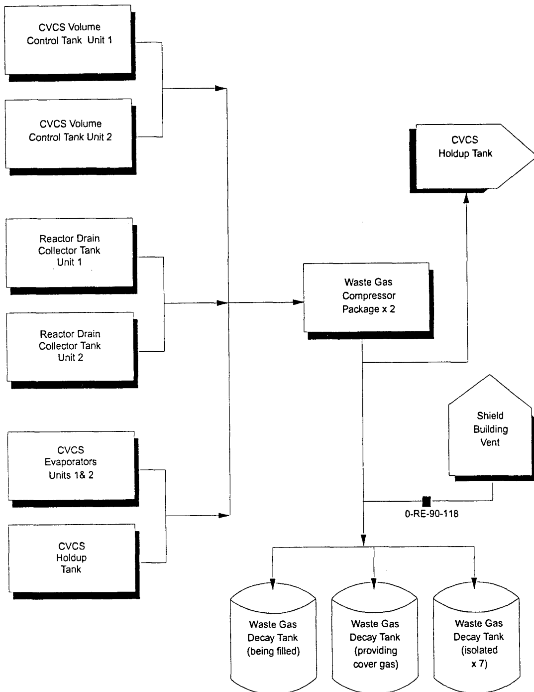
Figure 7.3 - GASEOUS RADWASTE TREATMENT SYSTEM
