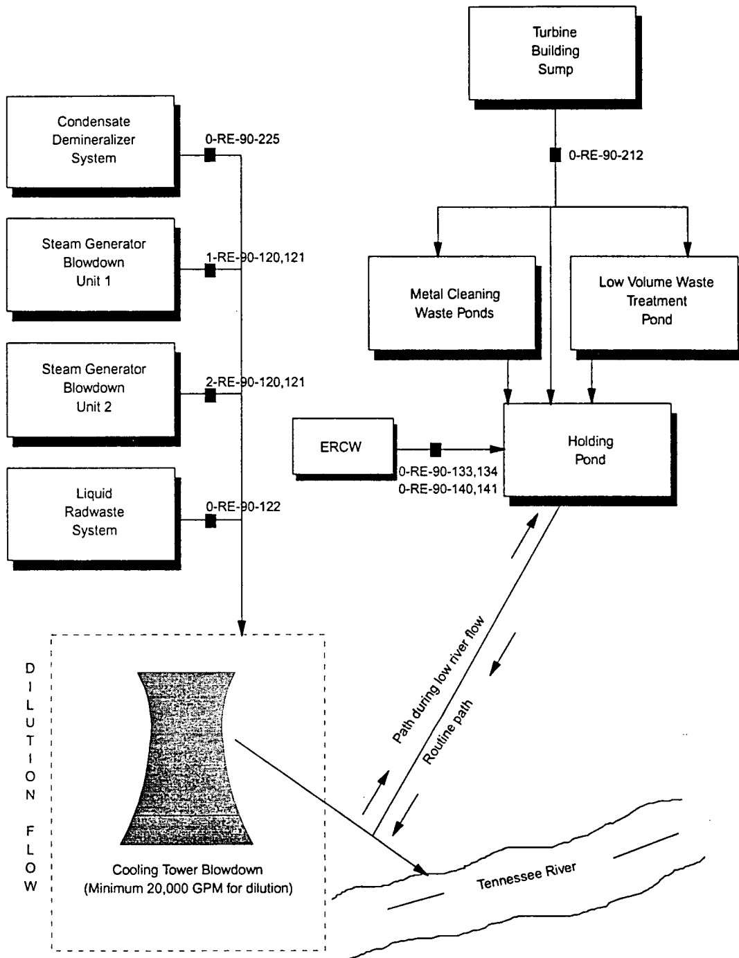
Figure 6.1 - LIQUID EFFLUENT RELEASE POINTS
