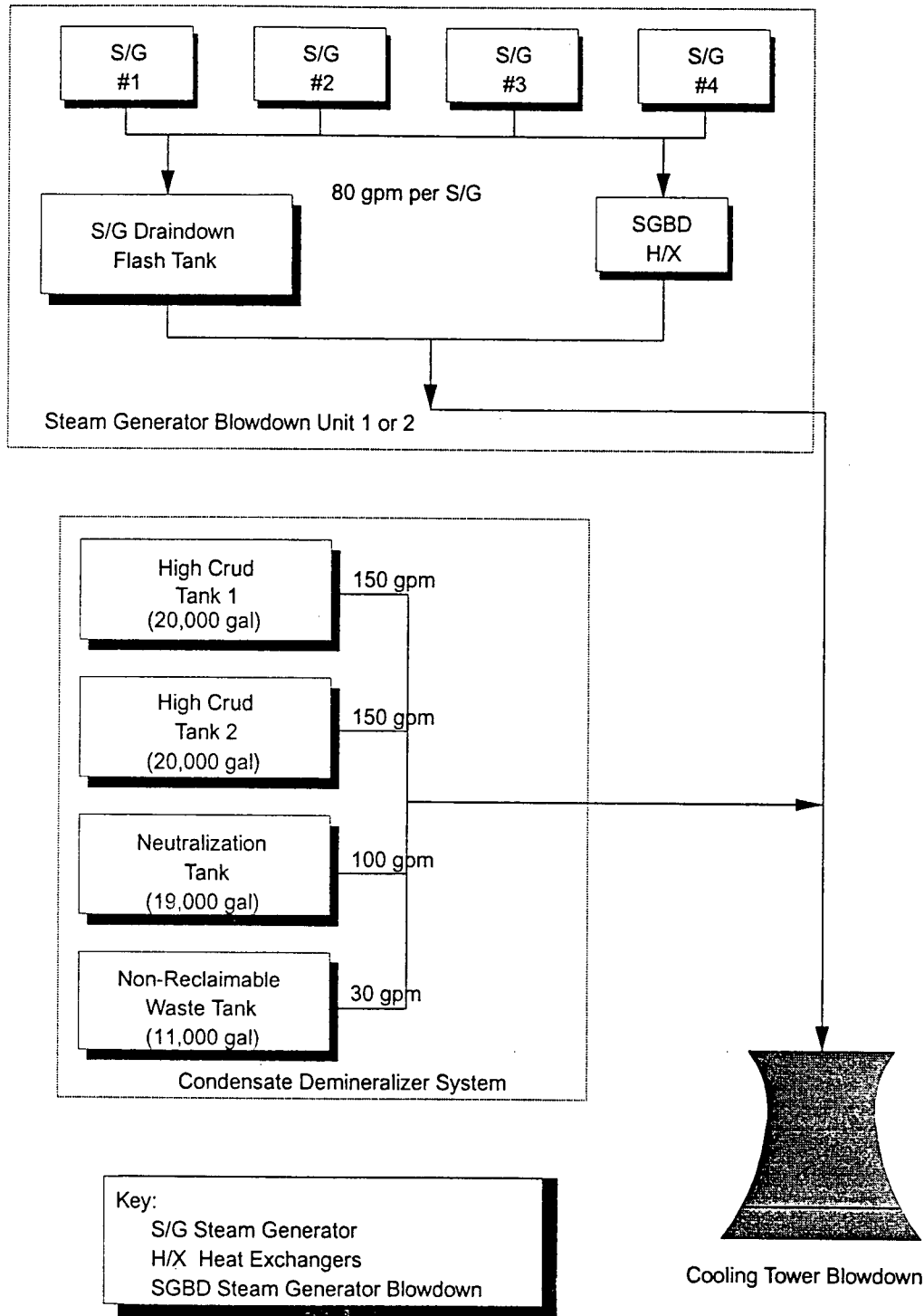
Figure 6.3 - STEAM GENERATOR BLOWDOWN/CONDENSATE DEMINERALIZER
