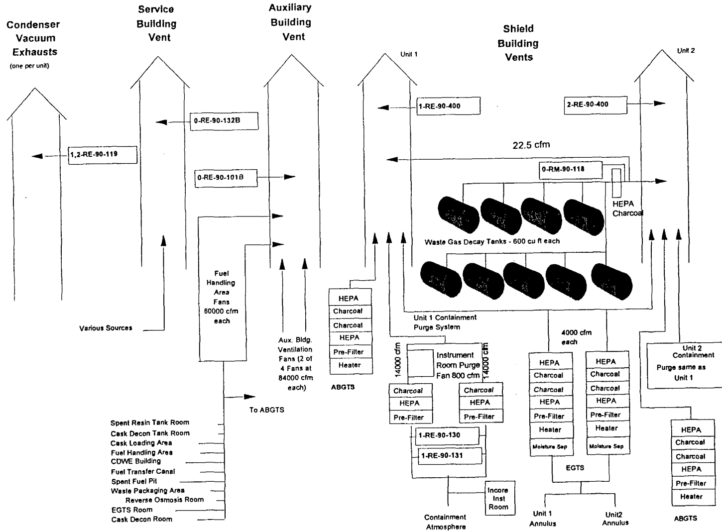
Figure 7.2 - DETAIL OF GASEOUS RELEASE/DISCHARGE POINTS
