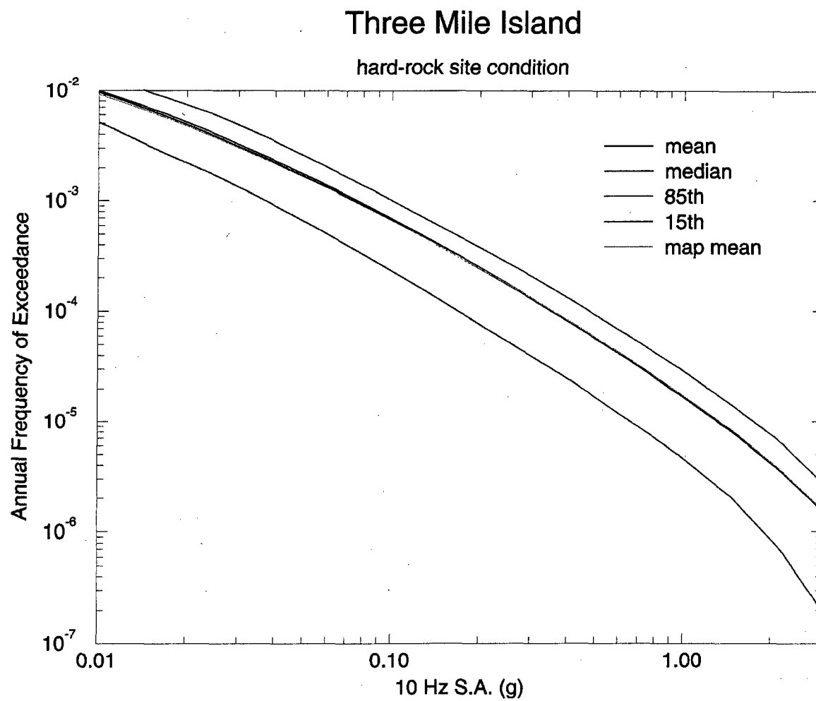
Figure 4. Hazard curves for 10 Hz S.A. at Three Mile Island. "Map mean" refers to the mean hazard curve derived from the procedure used in the 2002 national seismic hazard maps.
