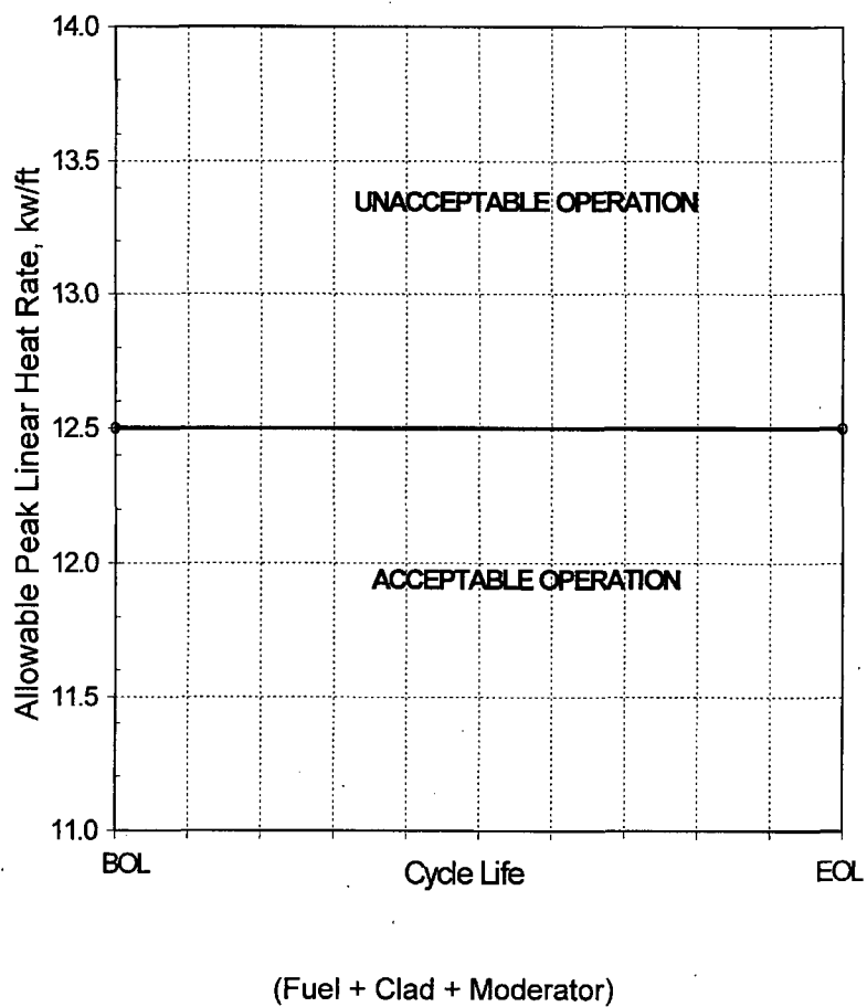
FIGURE 3.2-1 Allowable Peak Linear Heat Rate vs. Burnup
