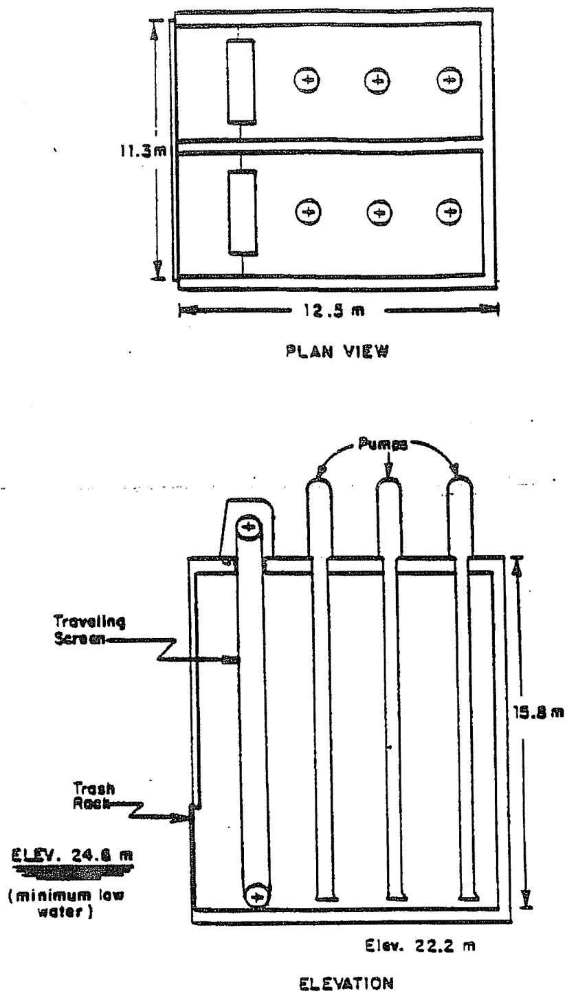
FIGURE 2-10. Schematic of 5G Pumphouse Intake
