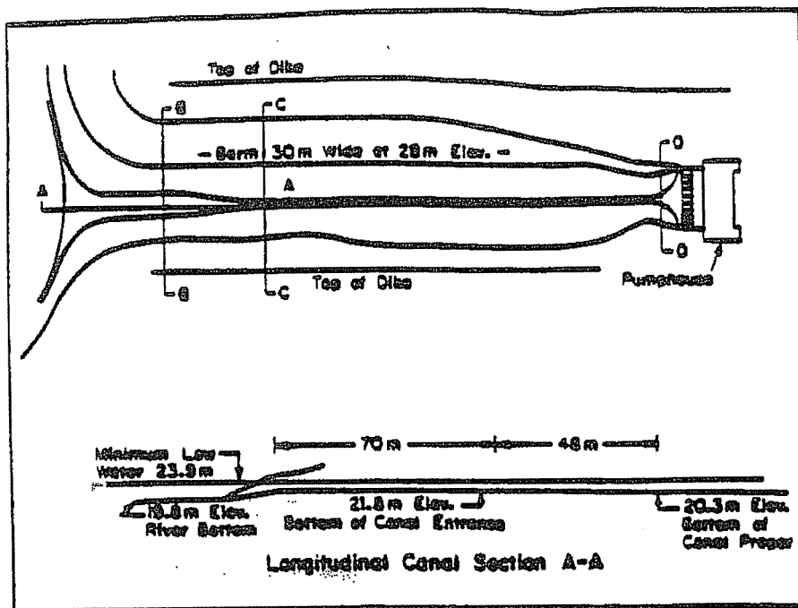
FIGURE 2-5. Plan View and Longitudinal Section of Entrance of 3G Canal
