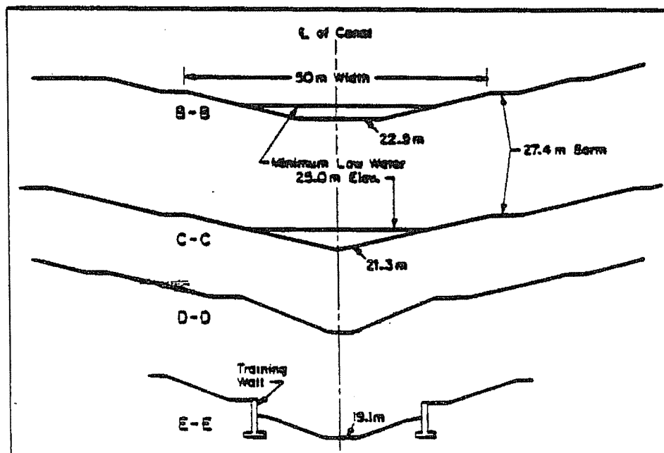
FIGURE 2-4. Cross Sections of 1G Canal at Points Designated in Figure 2-3
