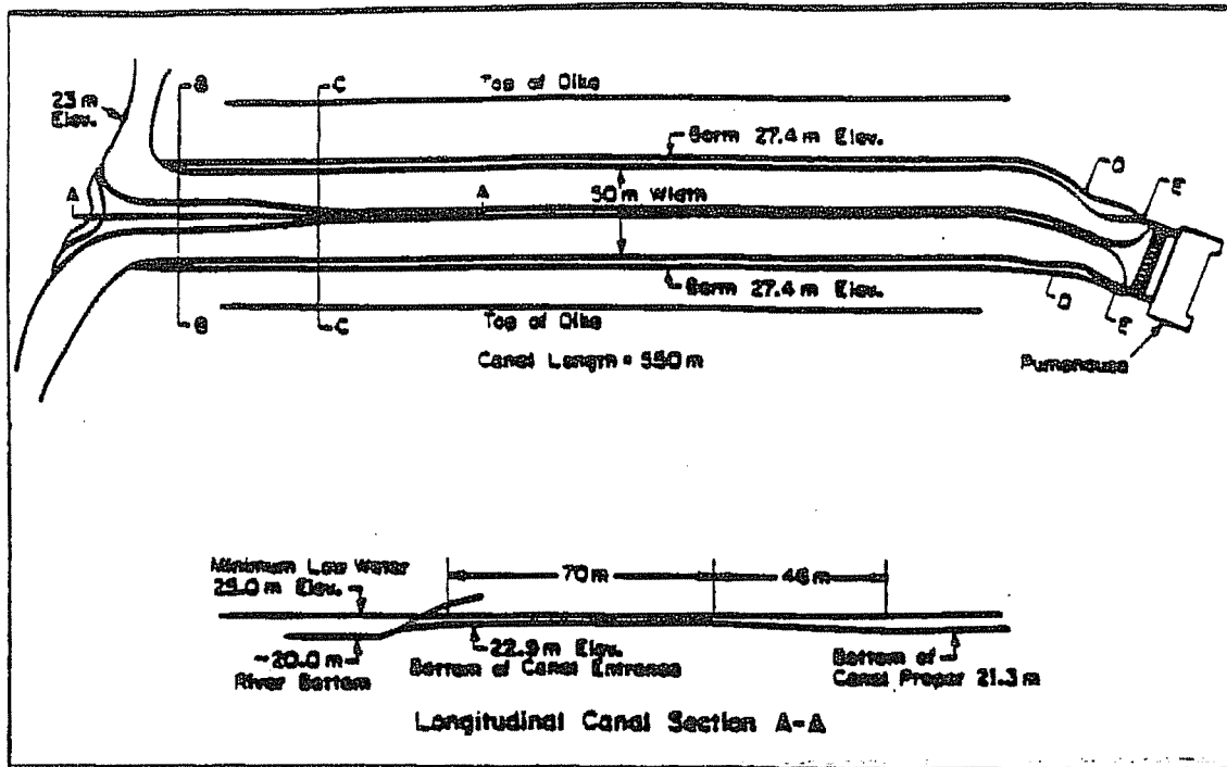
FIGURE 2-3. Plan View and Longitudinal Section of Entrance of 1G Canal
