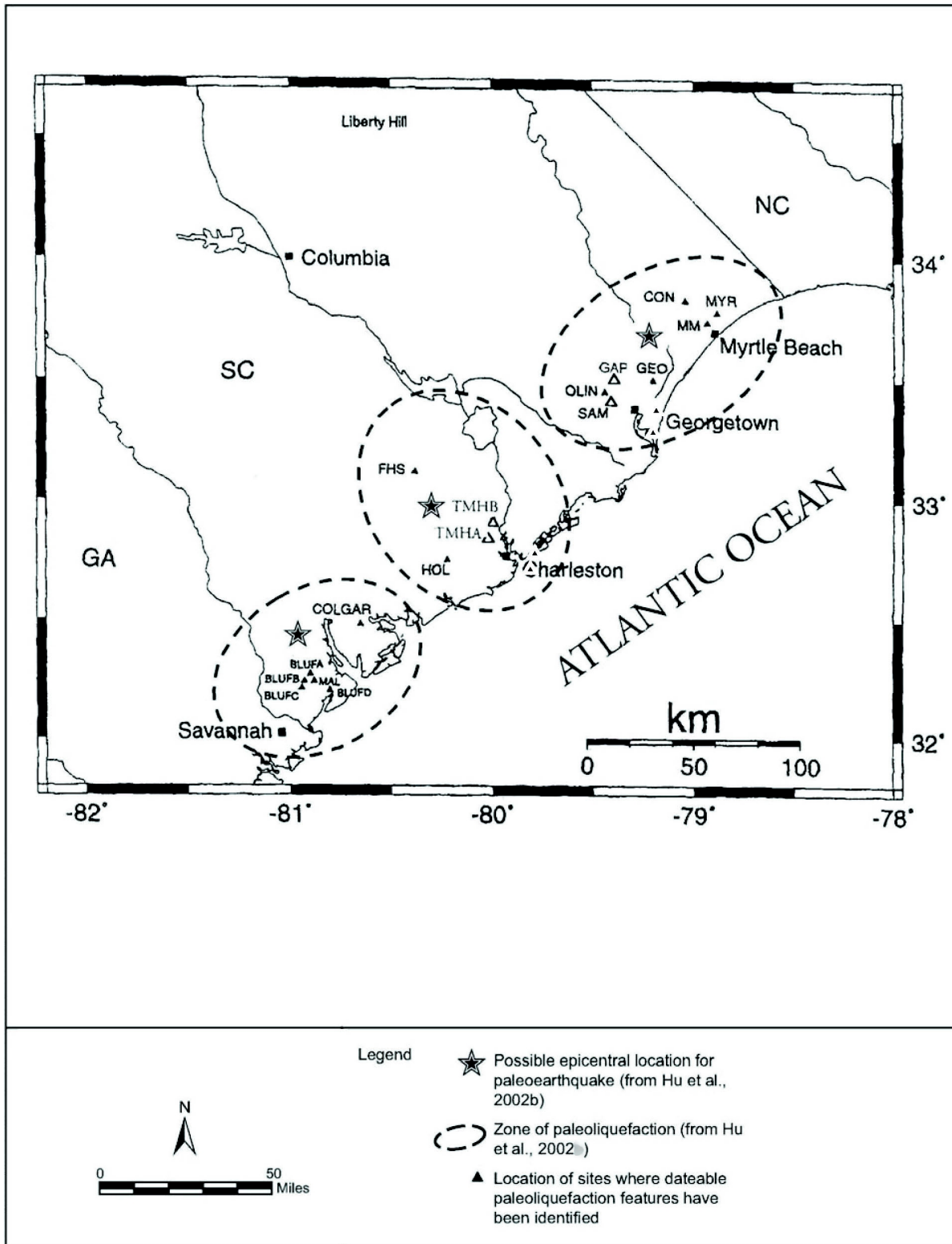
FIGURE 2.5-226 Distribution of Paleoliquefaction Sites in South Carolina and North Carolina
