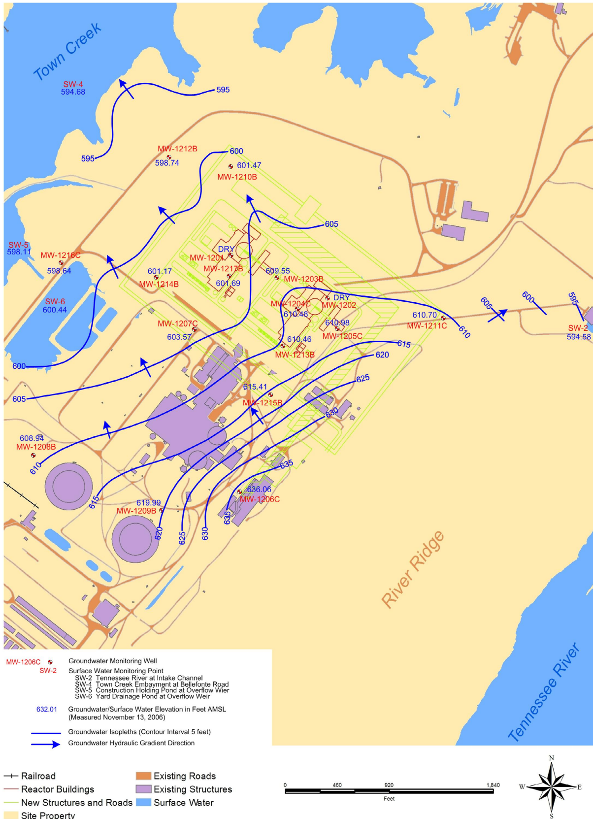
FIGURE 2.4.12-215 November 2006 Groundwater Potentiometric Surface Map
