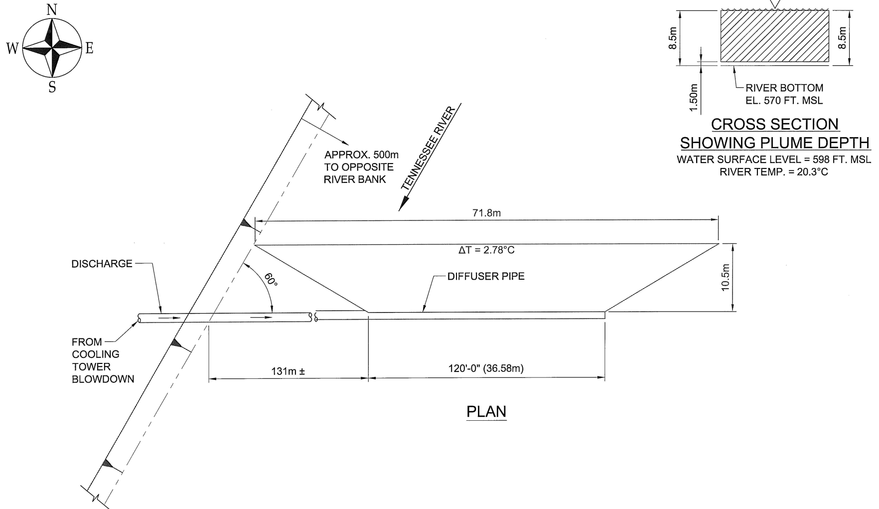
FIGURE 5.3-10 Mean River Temperature, Maximum Reverse River Flow
