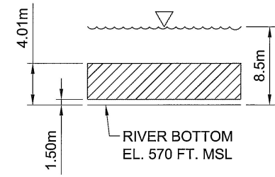
CROSS SECTION SHOWING PLUME DEPTH WATER SURFACE LEVEL = 598 FT. MSL RIVER TEMP. = 20.3°C
