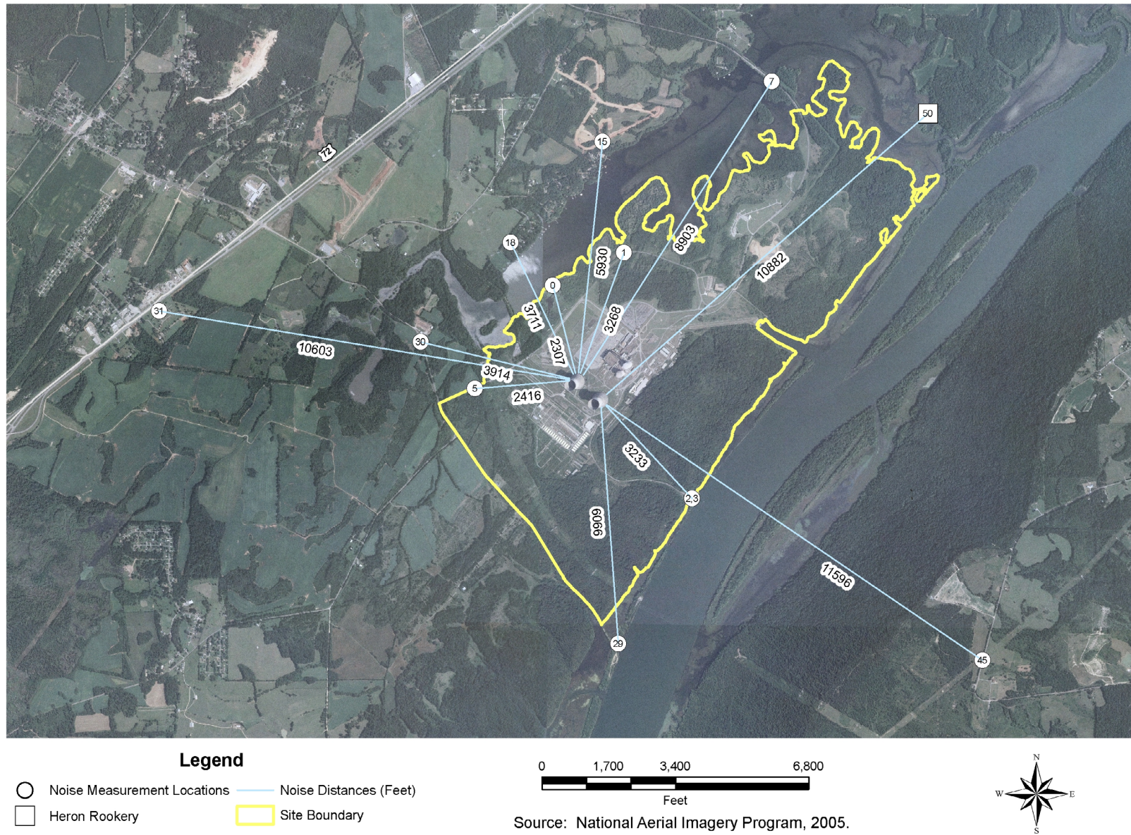
FIGURE 2.5-29 Noise Distances for BLN Site
