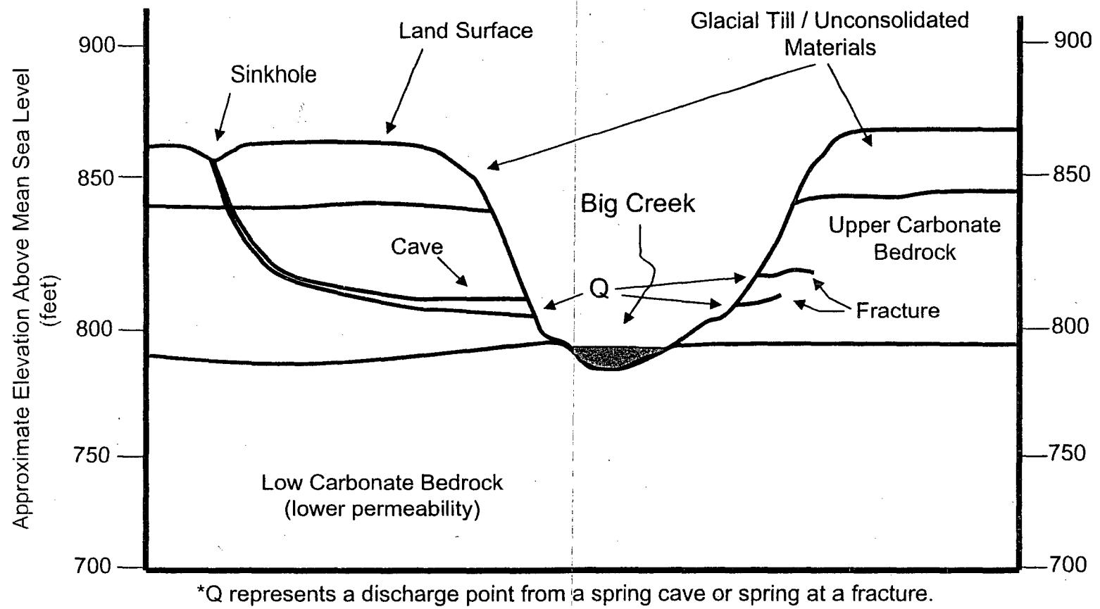
Figure 1. *Schematic Cross Section Through Big Creek Valley Within DU Impact Area Near Cave BC-12.
