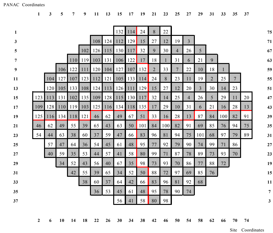
Figure 4.3-5. Hydraulic Control Unit Assignments
