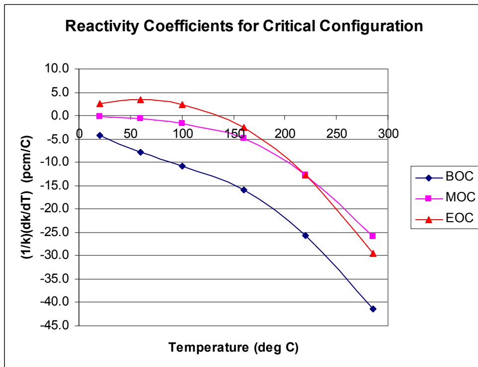
Figure 4.3-3. Moderator Temperature Coefficient for Reference Equilibrium Core Design
