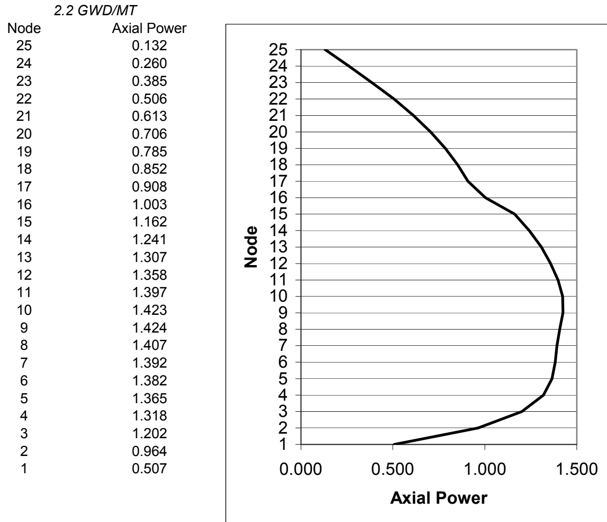
Figure 4A-3b. Relative Axial Power at 2.2 GWd/MT Exposure
