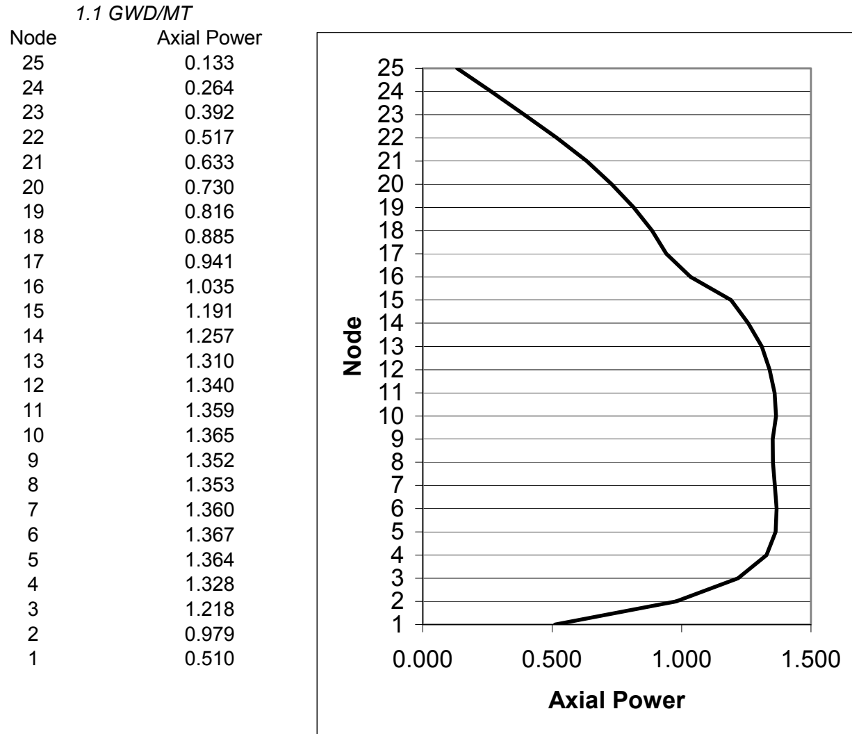
Figure 4A-2b. Relative Axial Power at 1.1 GWd/MT Exposure
