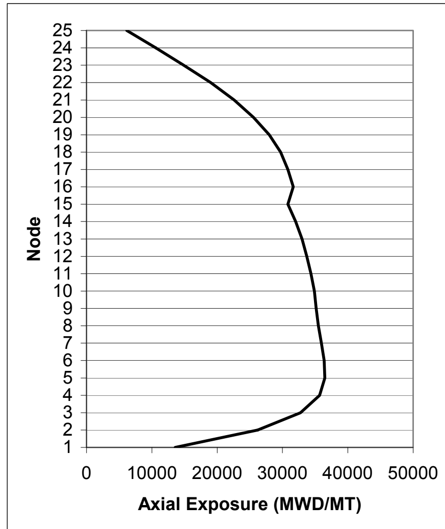
Figure 4A-14c. Axial Exposure at 14.3 GWd/MT Exposure
