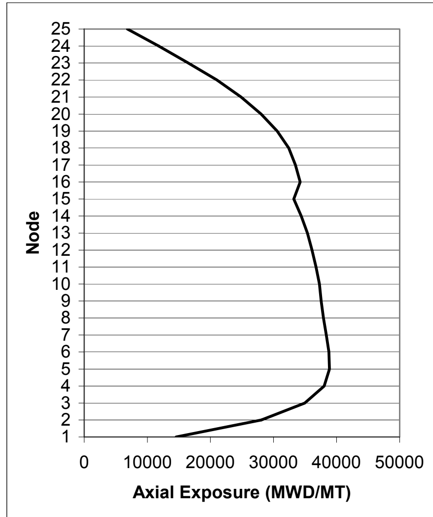
Figure 4A-16c. Axial Exposure at 16.5 GWd/MT Exposure
