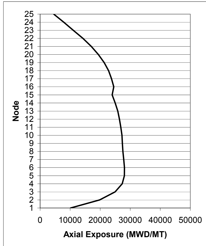
Figure 4A-8c. Axial Exposure at 7.7 GWd/MT Exposure
