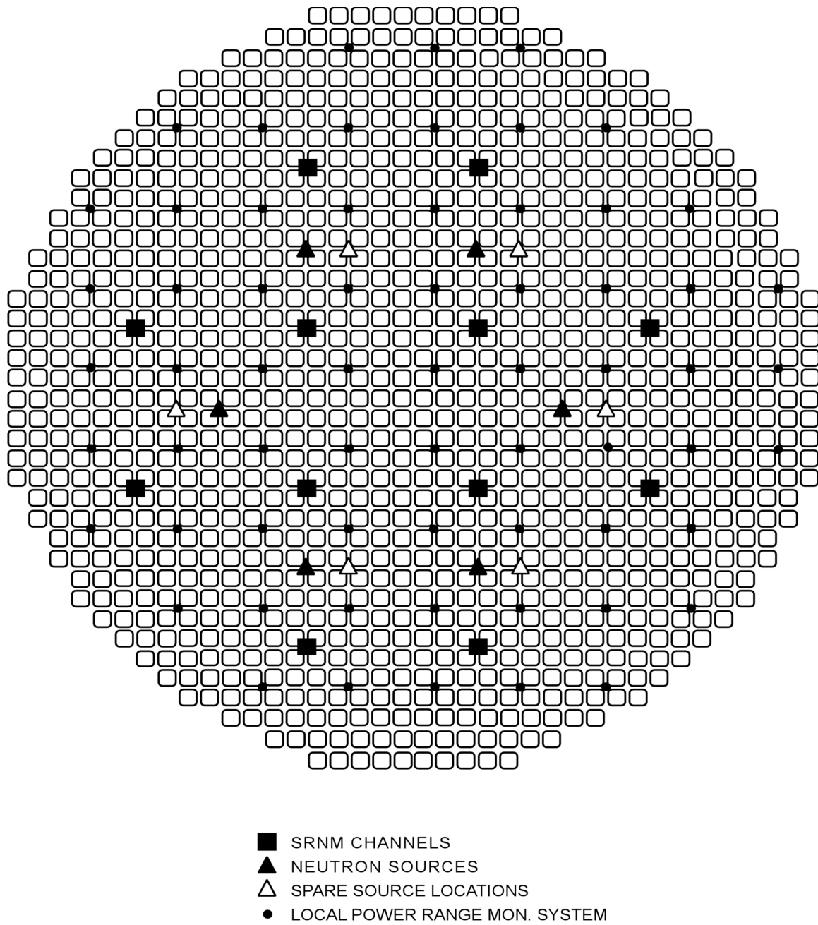
Figure 4.1-1. Core Configuration with Location of Instrumentation
