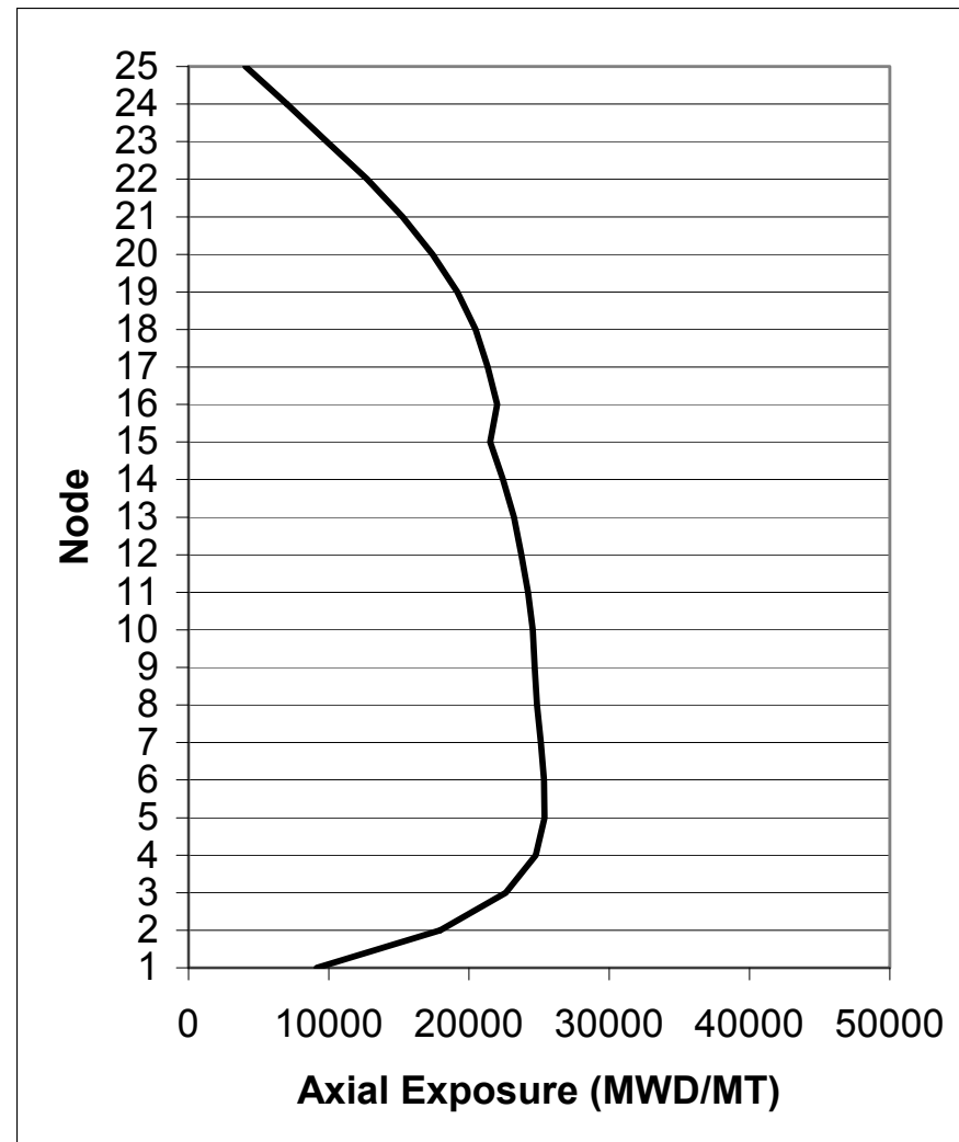
Figure 4A-6c. Axial Exposure at 5.5 GWd/MT Exposure
