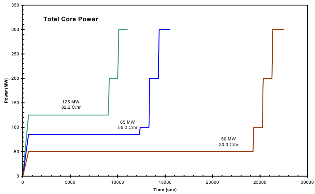
Figure 4D-11. TRACG Startup Simulation: Reactor Power Trajectories
