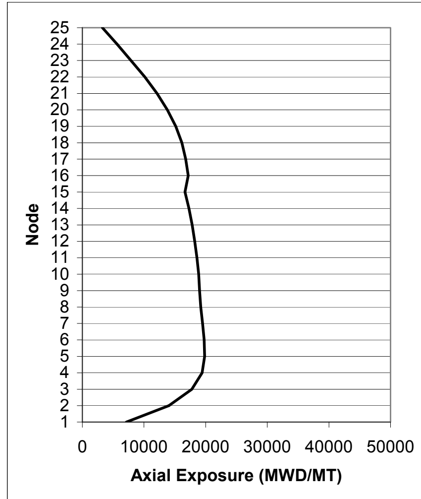
Figure 4A-2c. Axial Exposure at 1.1 GWd/MT Exposure
