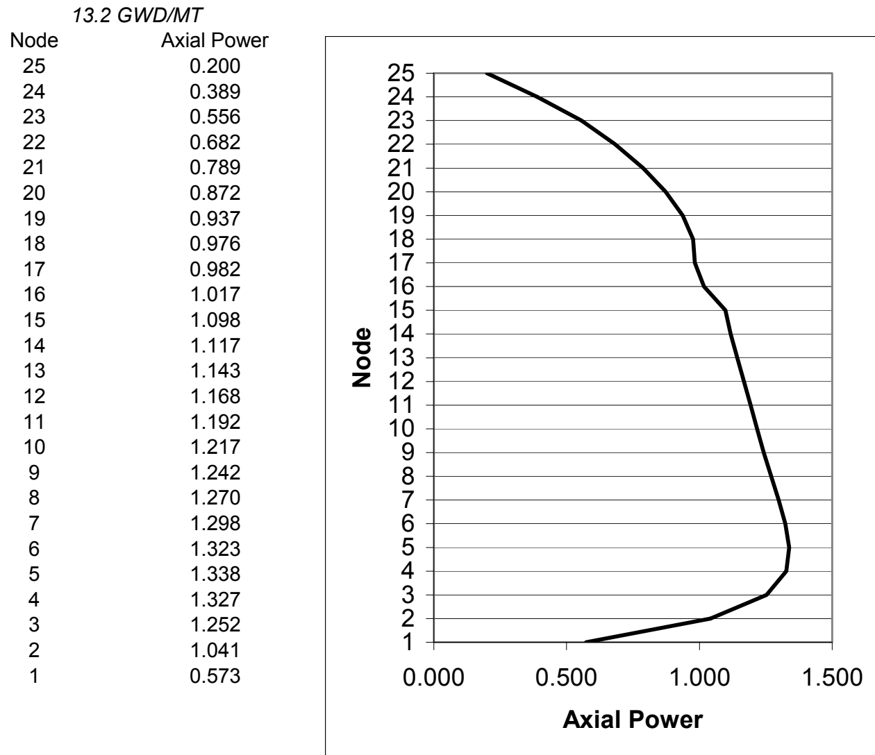
Figure 4A-13b. Relative Axial Power at 13.2 GWd/MT Exposure
