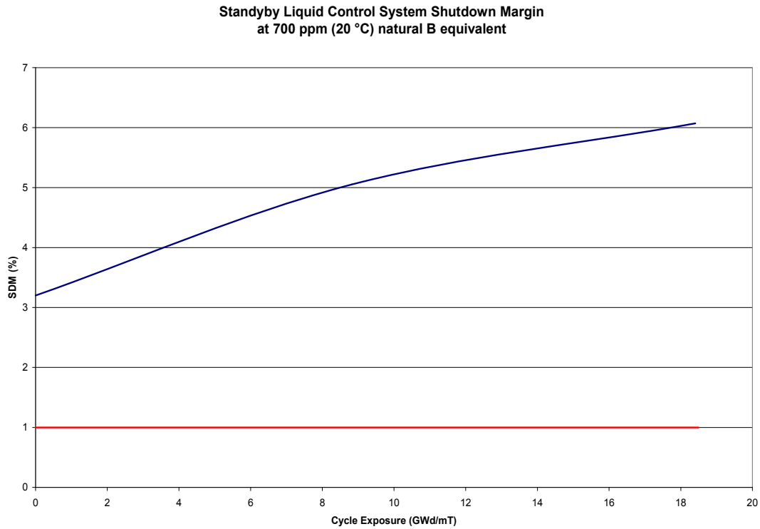
Figure 4.3-4. SLCS Shutdown Margin for Reference Equilibrium Core Design
