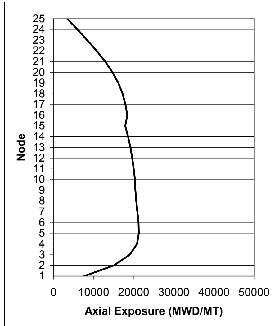
Figure 4A-3c. Axial Exposure at 2.2 GWd/MT Exposure
