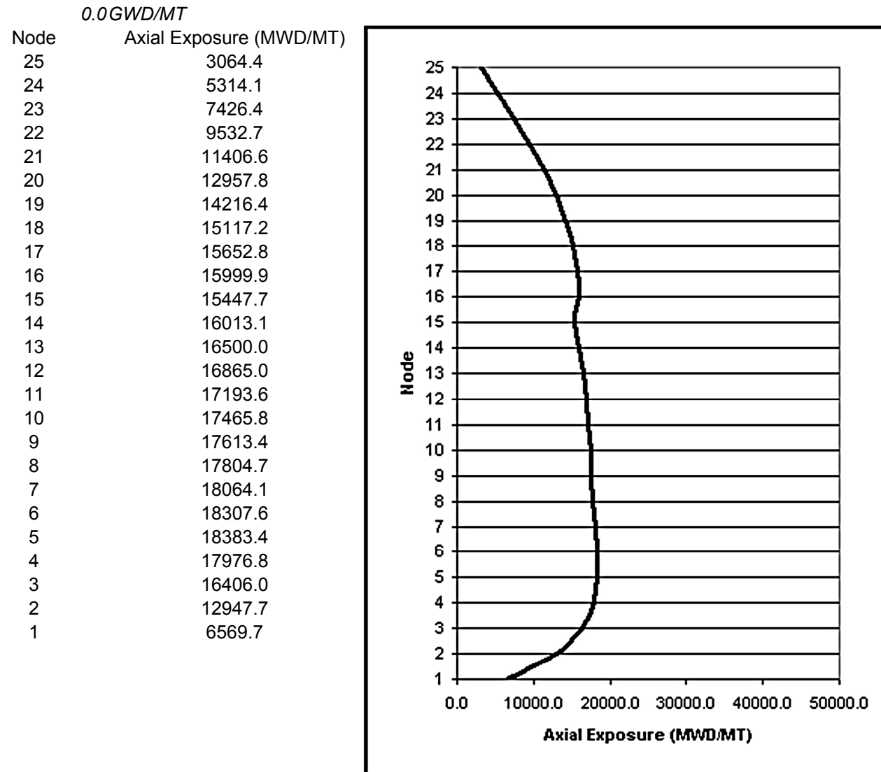
Figure 4A-1c. Axial Exposure at 0.0 GWd/MT Exposure
