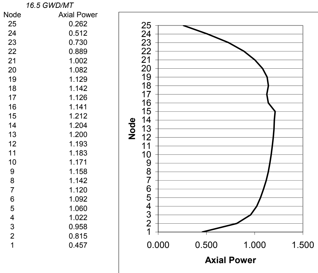
Figure 4A-16b. Relative Axial Power at 16.5 GWd/MT Exposure
