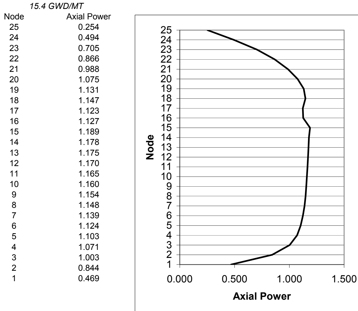
Figure 4A-15b. Relative Axial Power at 15.4 GWd/MT Exposure
