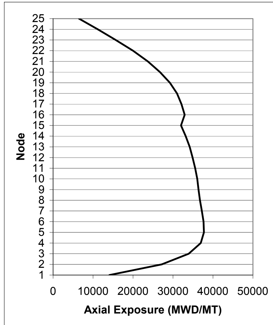
Figure 4A-15c. Axial Exposure at 15.4 GWd/MT Exposure
