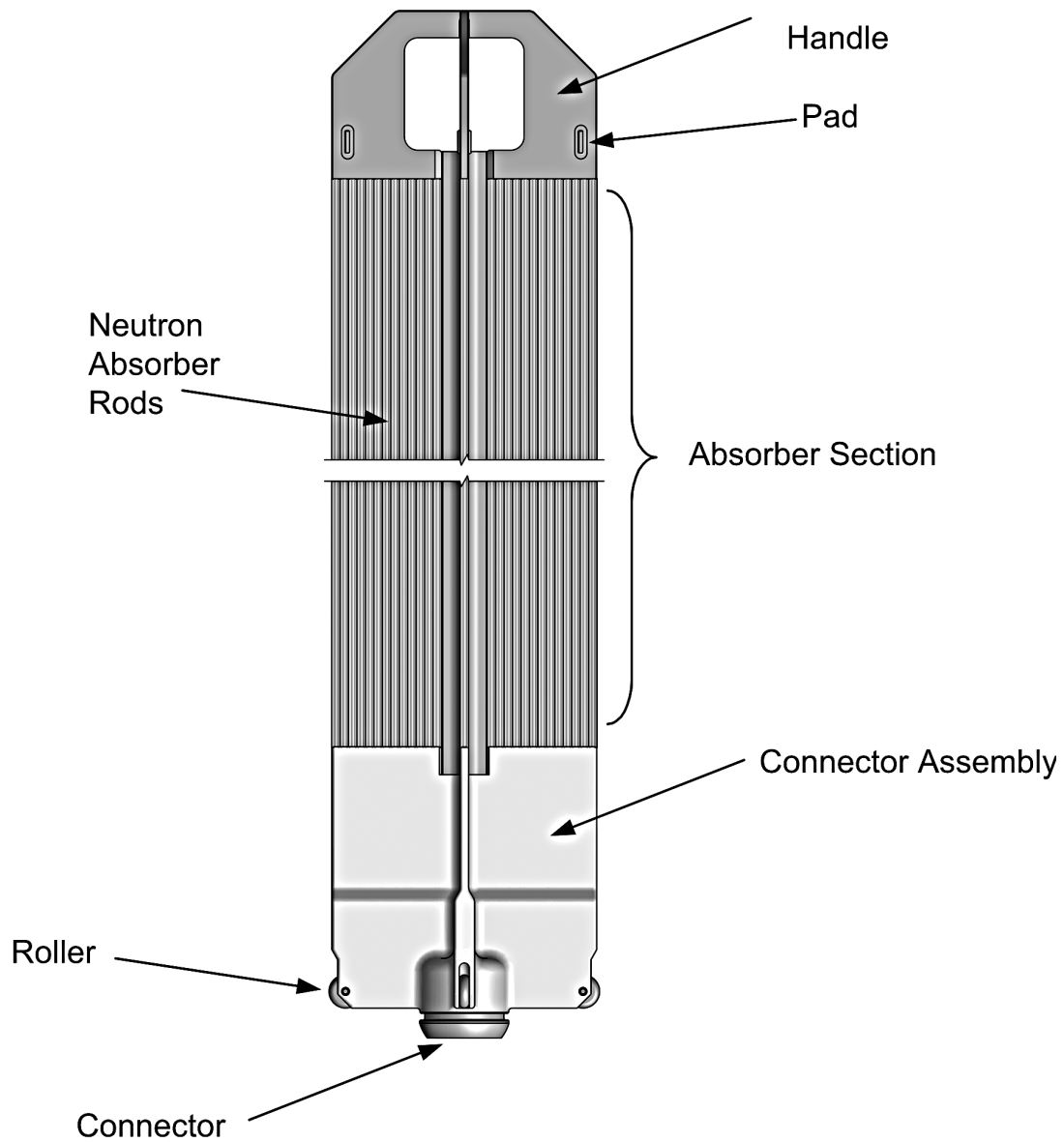
Figure 4.2-3. Typical Control Rod Assembly
