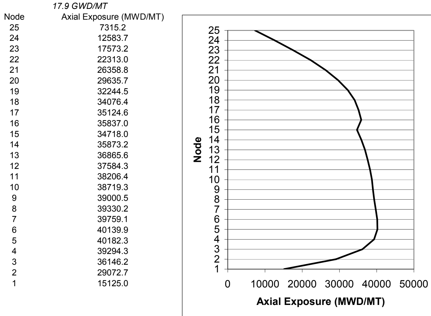
Figure 4A-17c. Axial Exposure at 17.9 GWd/MT Exposure
