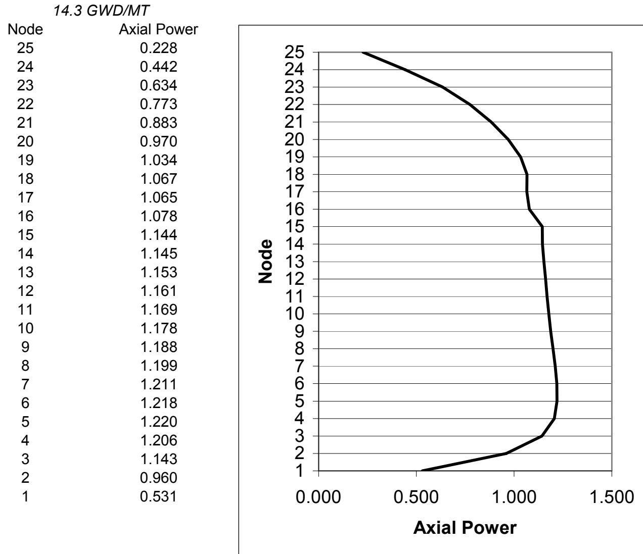
Figure 4A-14b. Relative Axial Power at 14.3 GWd/MT Exposure
