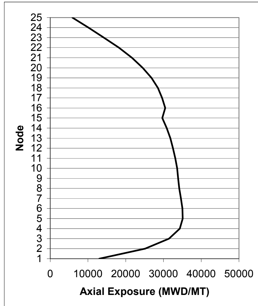
Figure 4A-13c. Axial Exposure at 13.2 GWd/MT Exposure
