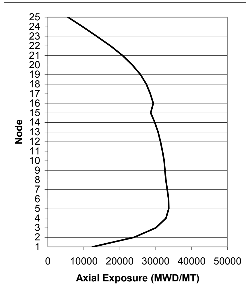
Figure 4A-12c. Axial Exposure at 12.1 GWd/MT Exposure
