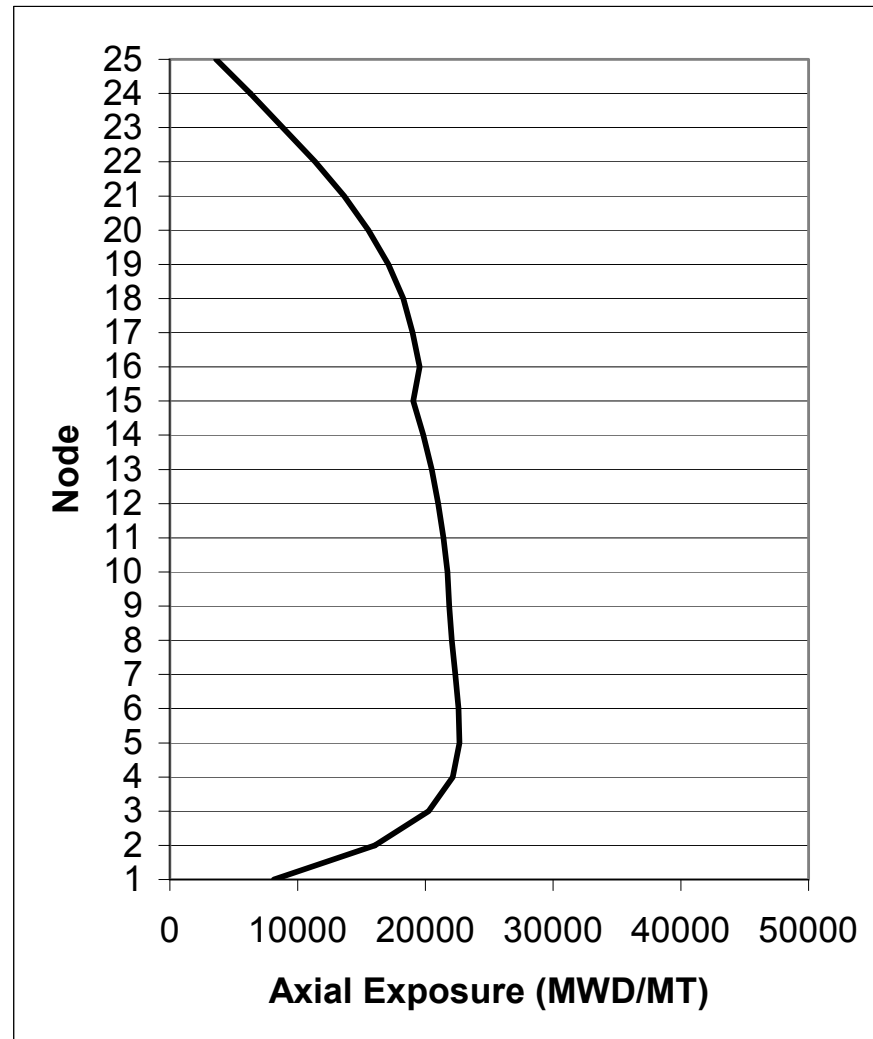
Figure 4A-4c. Axial Exposure at 3.3 GWd/MT Exposure
