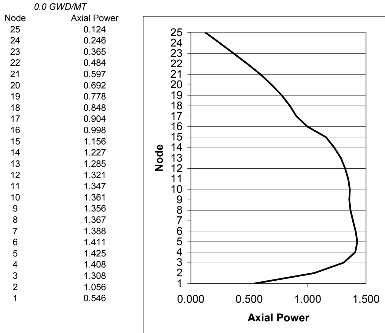
Figure 4A-1b. Relative Axial Power at 0.0 GWd/MT
