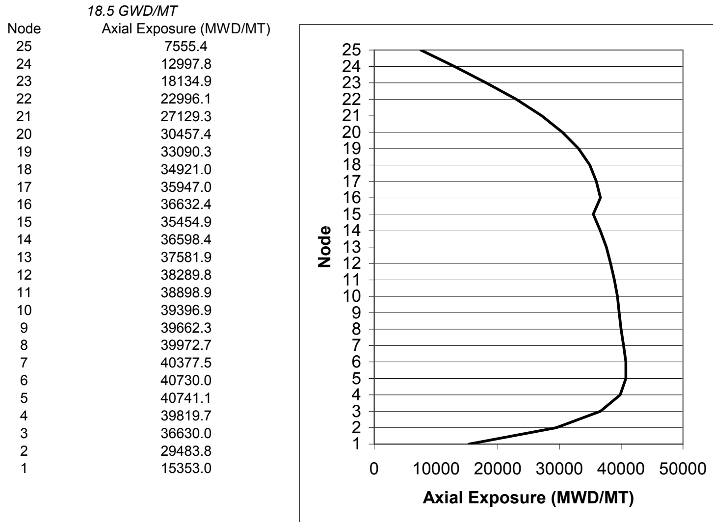
Figure 4A-18c. Axial Exposure at 18.5 GWd/MT Exposure
