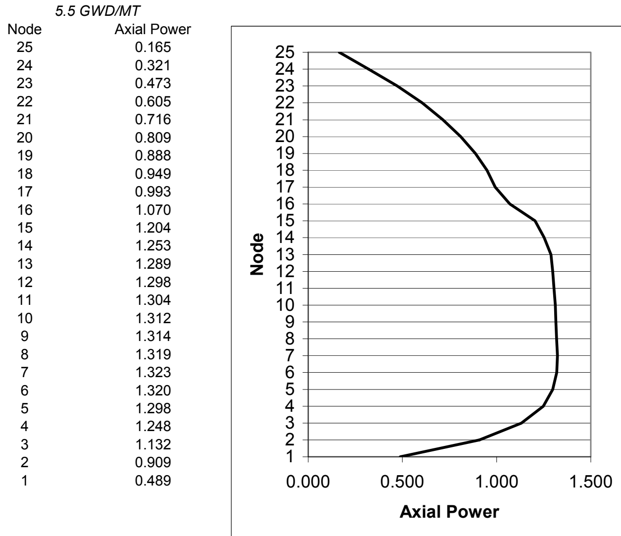
Figure 4A-6b. Relative Axial Power at 5.5 GWd/MT Exposure
