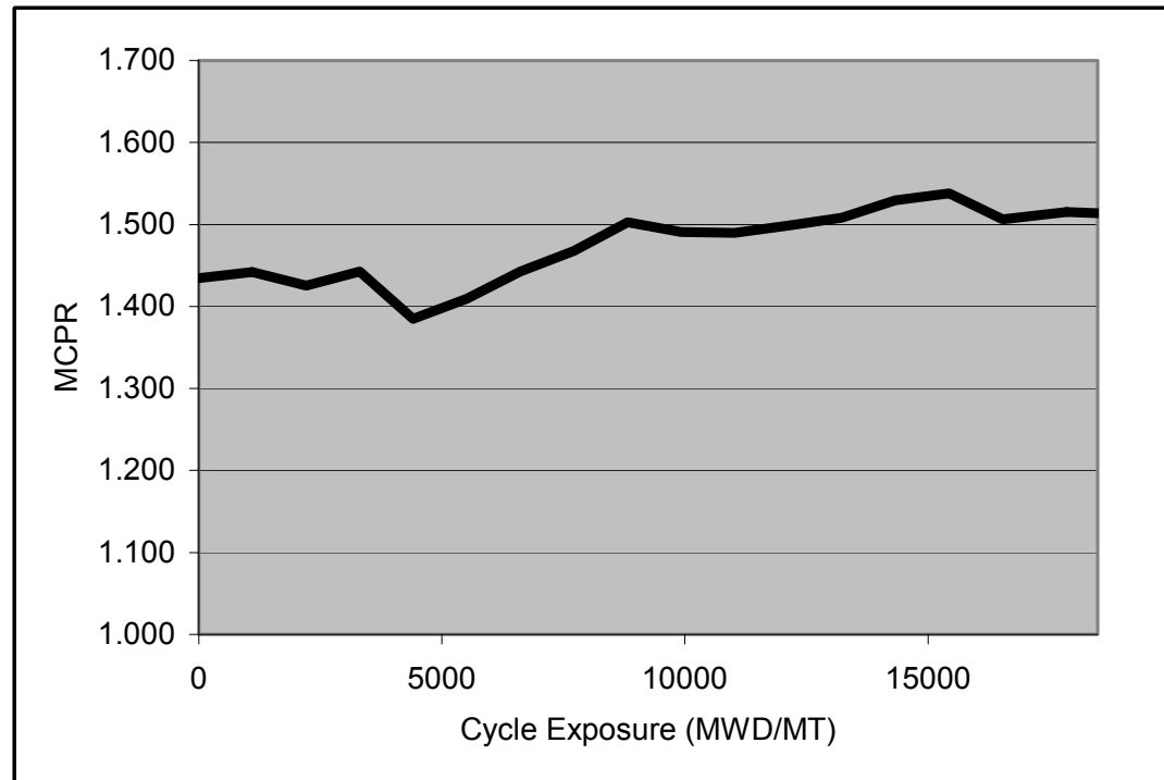
Figure 4A-19. Minimum Critical Power Ratio (MCPR) as a Function of Exposure
