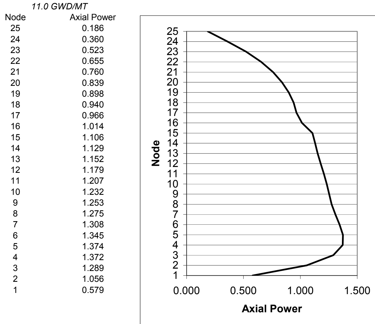
Figure 4A-11b. Relative Axial Power at 11.0 GWd/MT Exposure
