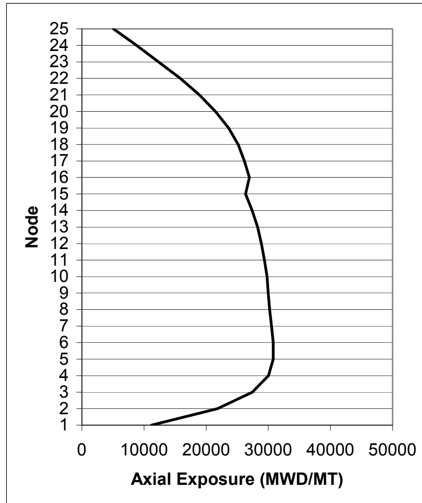
Figure 4A-10c. Axial Exposure at 9.9 GWd/MT Exposure
