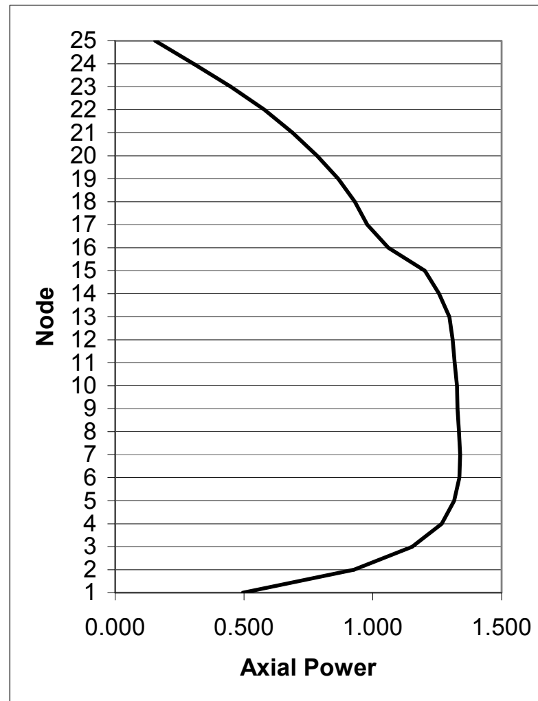
Figure 4A-5b. Relative Axial Power at 4.4 GWd/MT Exposure
