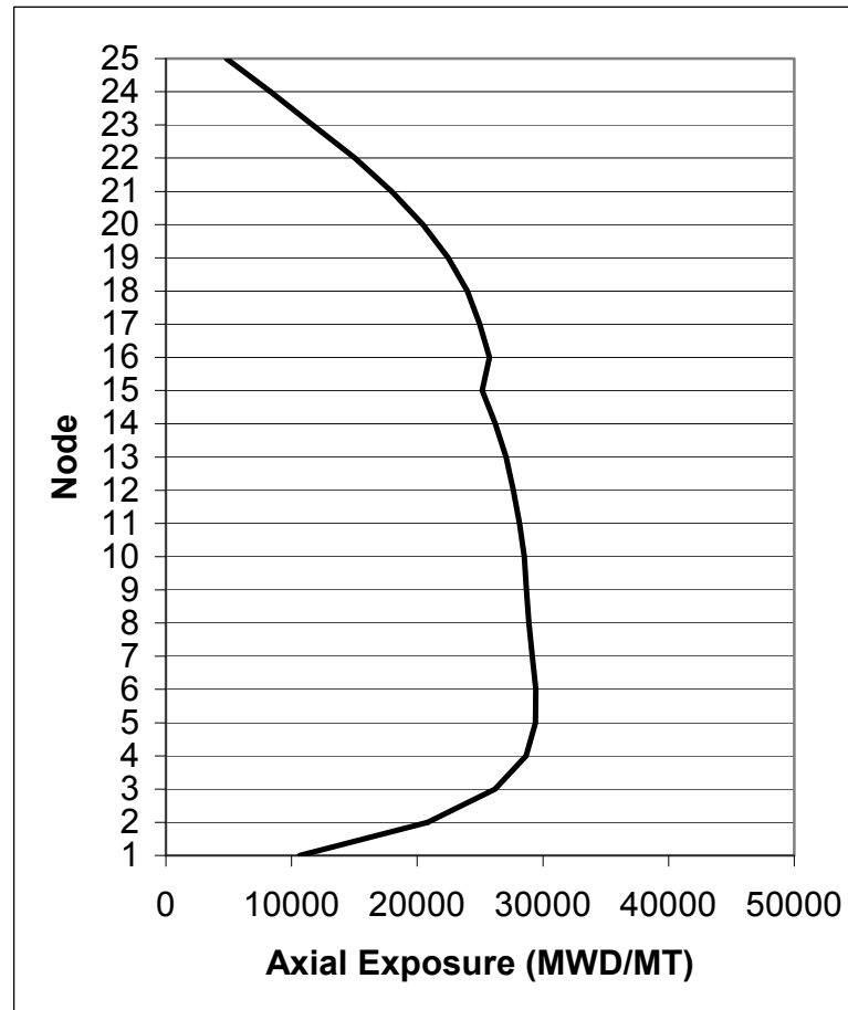
Figure 4A-9c. Axial Exposure at 8.8 GWd/MT Exposure
