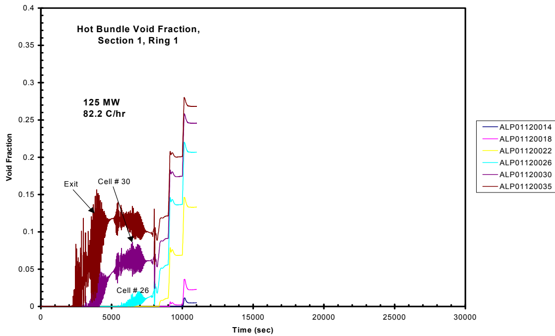
Figure 4D-20. Hot Bundle Void Fraction (125 MWt heatup)
