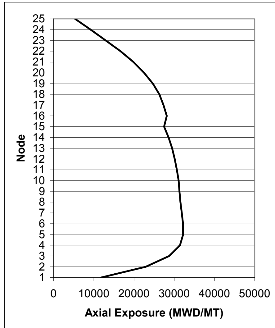
Figure 4A-11c. Axial Exposure at 11.0 GWd/MT Exposure
