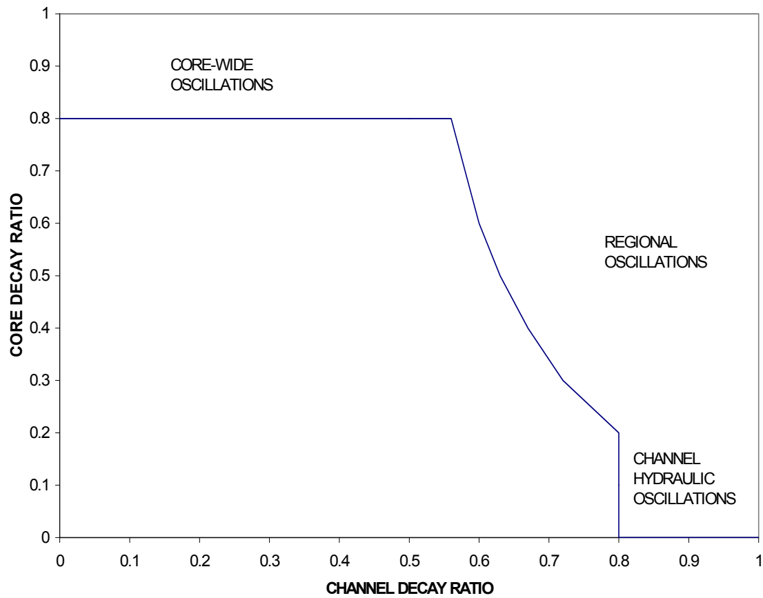
Figure 4D-1. Two-Dimensional Stability Map for ESBWR
