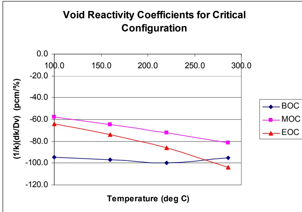
Figure 4.3-2. Moderator Void Coefficient for Reference Equilibrium Core Design
