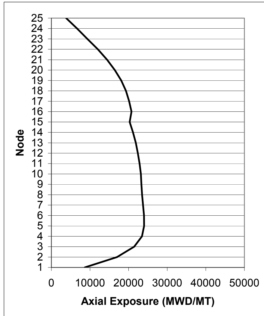
Figure 4A-5c. Axial Exposure at 4.4 GWd/MT Exposure
