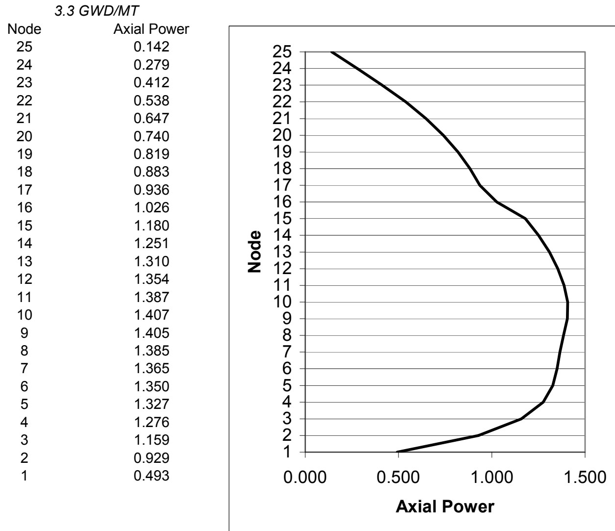
Figure 4A-4b. Relative Axial Power at 3.3 GWd/MT Exposure
