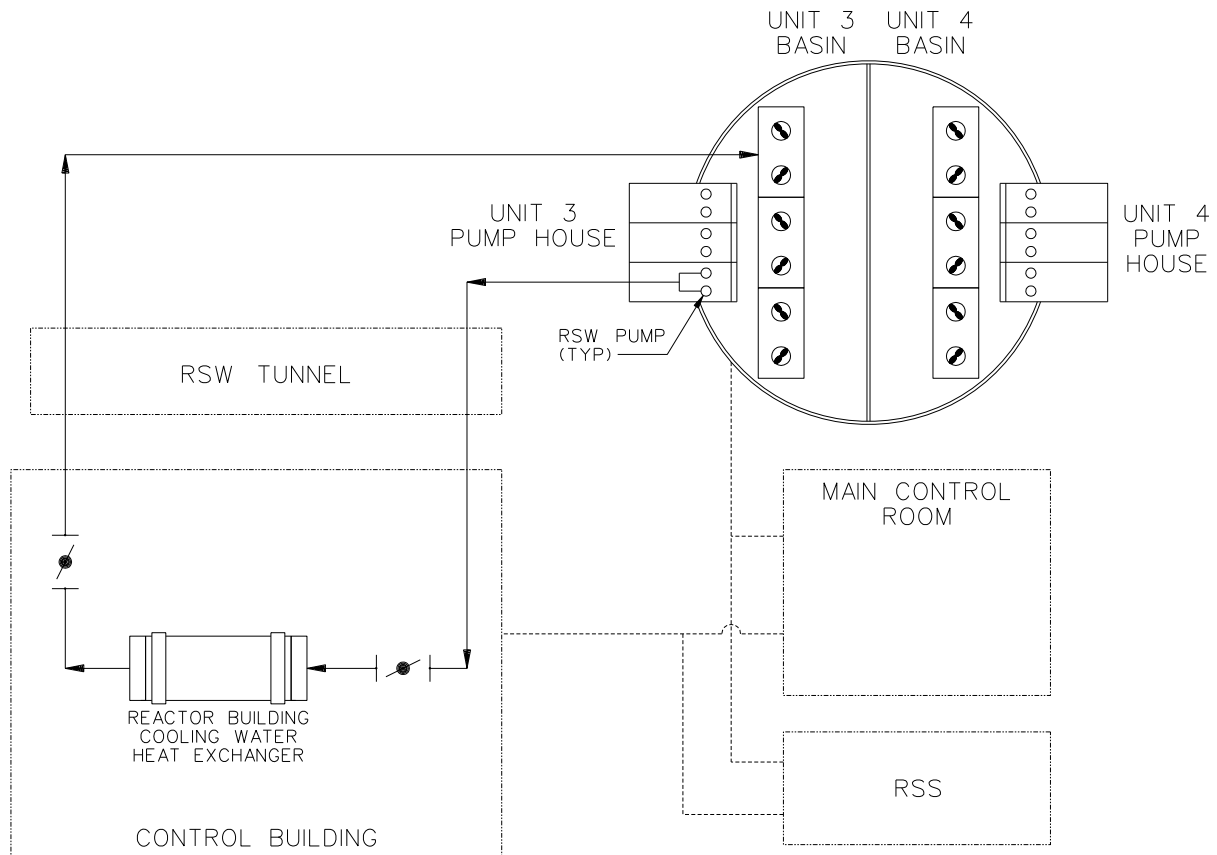
Figure 9.3-1 UHS and Reactor Service Water System
