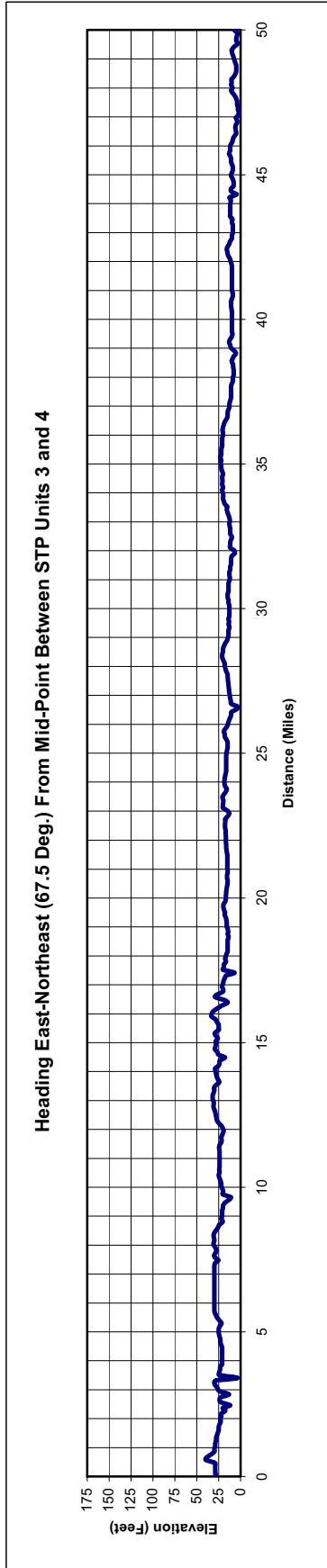
Figure 2.7-16 Terrain Elevation Profiles Within 50 Miles of the STP Site (Sheet 2 of 8)
