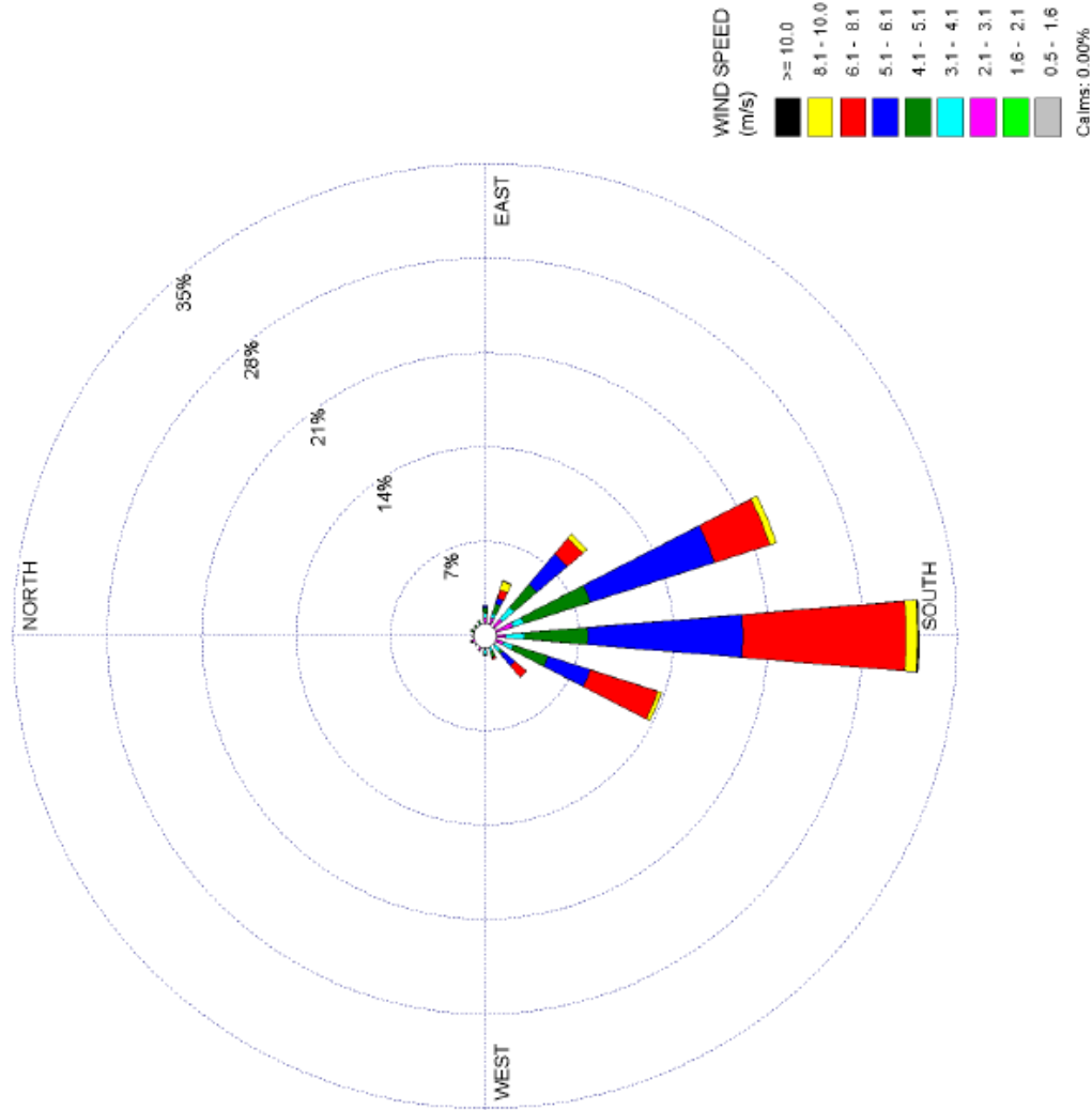
Figure 2.7-13 STP 60-Meter Level 3-Year Composite Wind Rose - July (1997, 1999, and 2000) - Page 7 of 12
