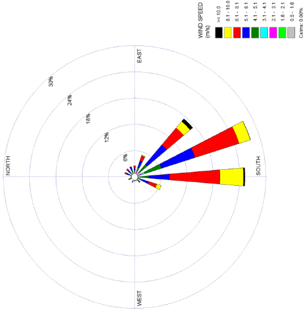
Figure 2.7-13 STP 60-Meter Level 3-Year Composite Wind Rose - June (1997, 1999, and 2000) - Page 6 of 12
