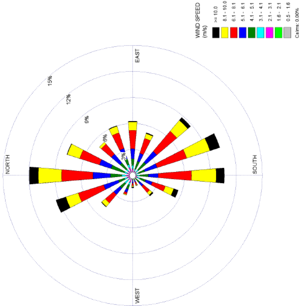
Figure 2.7-9 STP 60-Meter Level 3-Year Composite Wind Rose - Winter (1997, 1999, and 2000)
