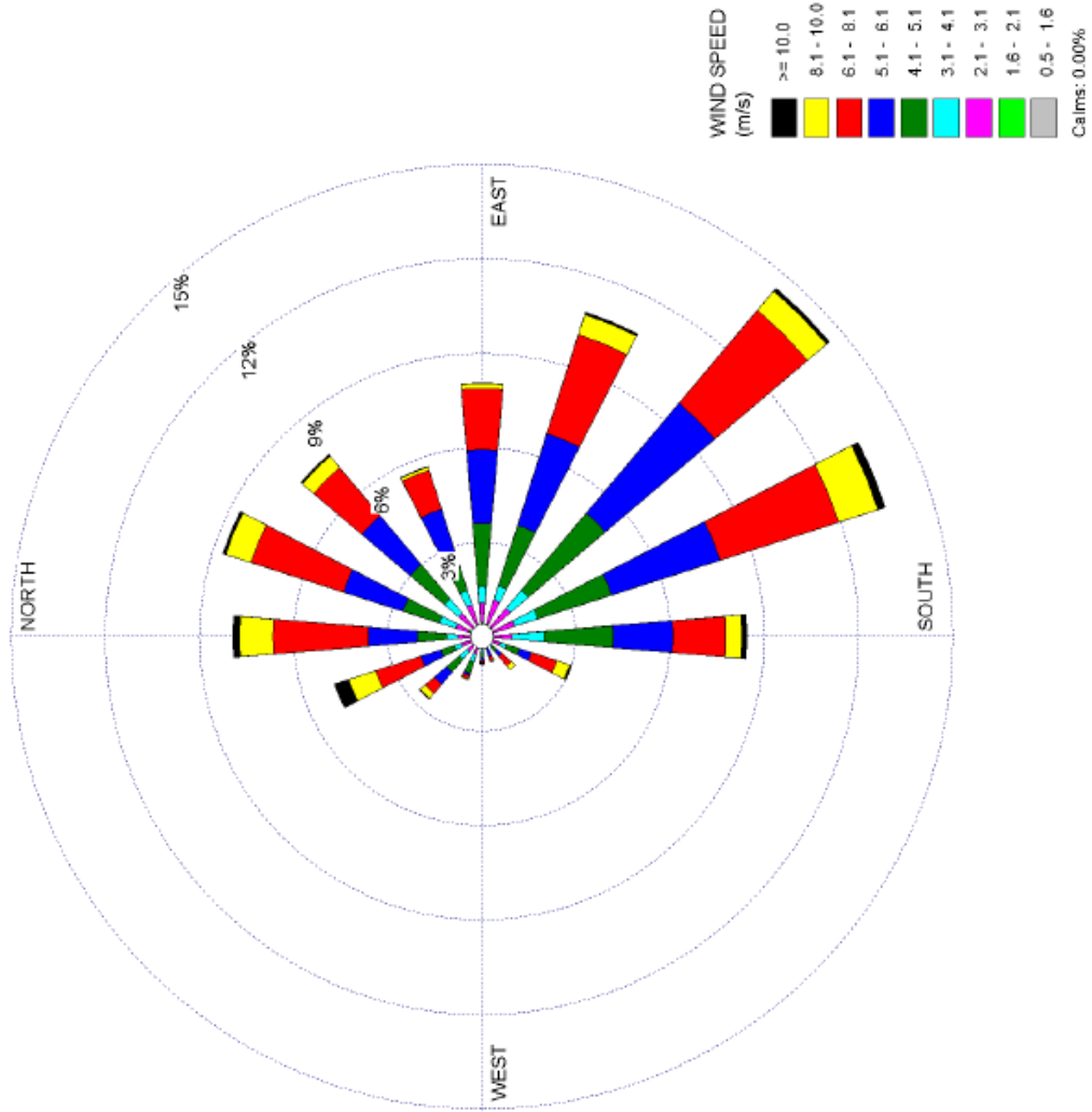
Figure 2.7-12 STP 60-Meter Level 3-Year Composite Wind Rose - Autumn (1997, 1999, and 2000)
