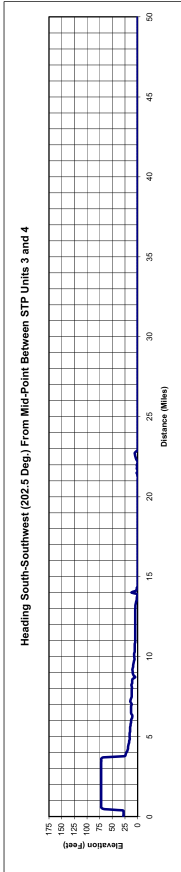
Figure 2.7-16 Terrain Elevation Profiles Within 50 Miles of the STP Site (Sheet 5 of 8)
