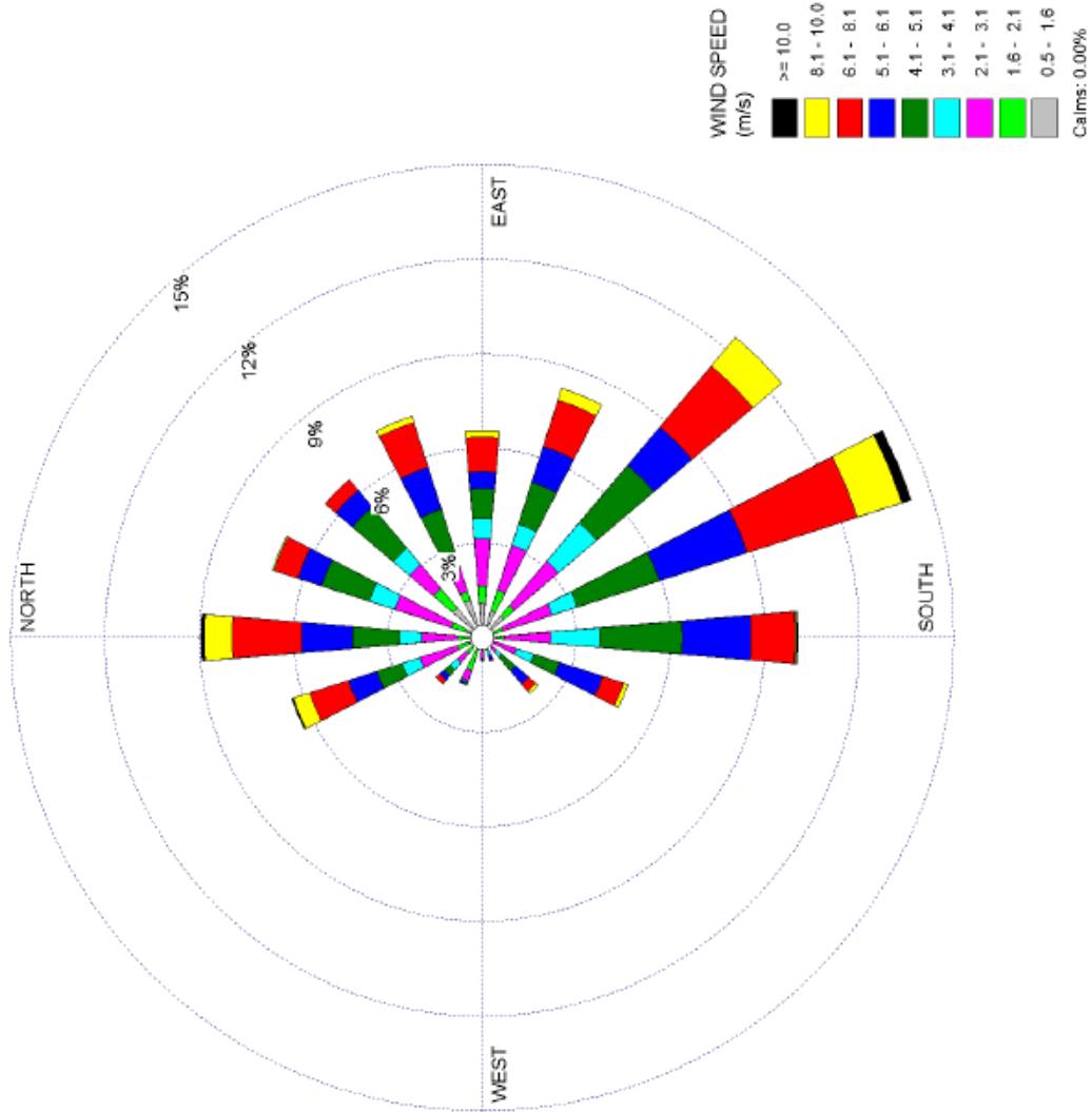
Figure 2.7-7 STP 10-Meter Level 3-Year Composite Wind Rose - February (1997, 1999, and 2000) - Page 2 of 12
