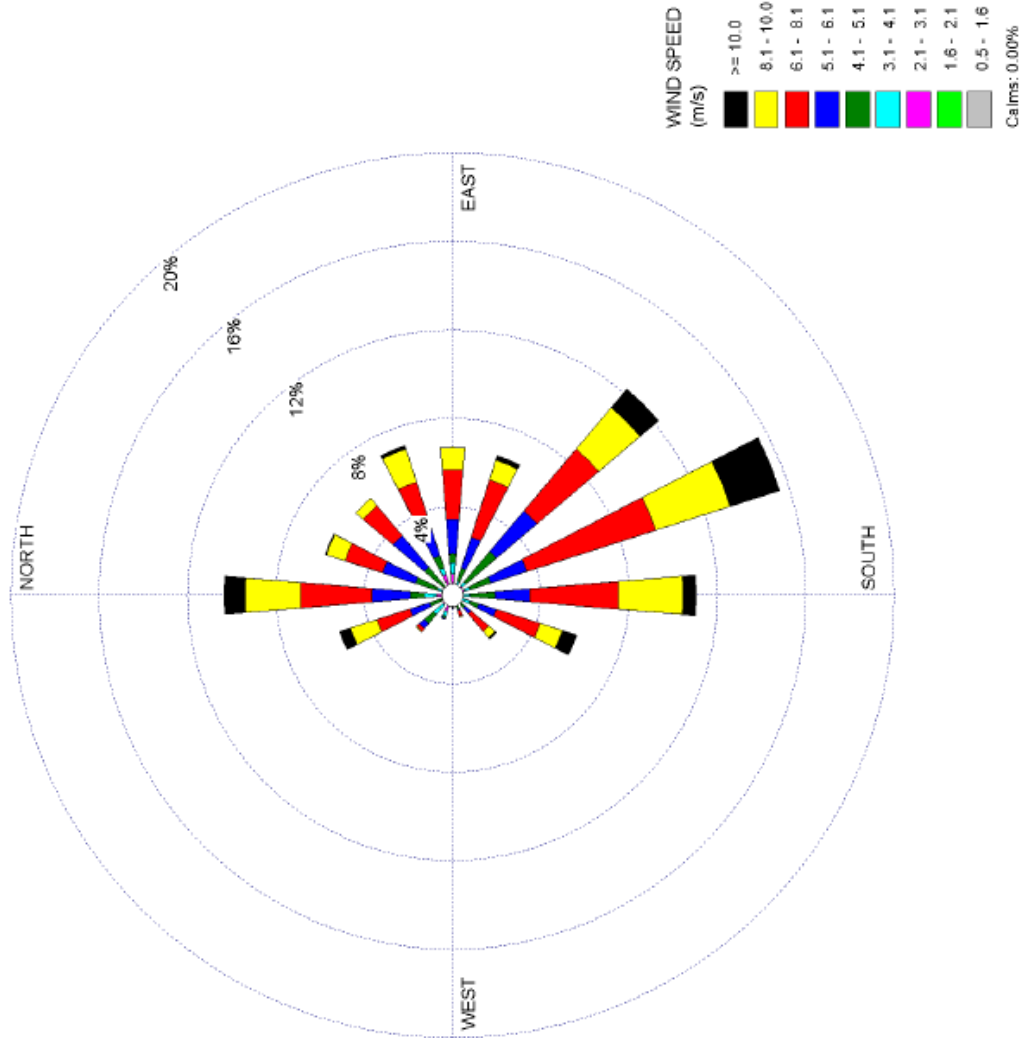
Figure 2.7-13 STP 60-Meter Level 3-Year Composite Wind Rose - February (1997, 1999, and 2000) - Page 2 of 12
