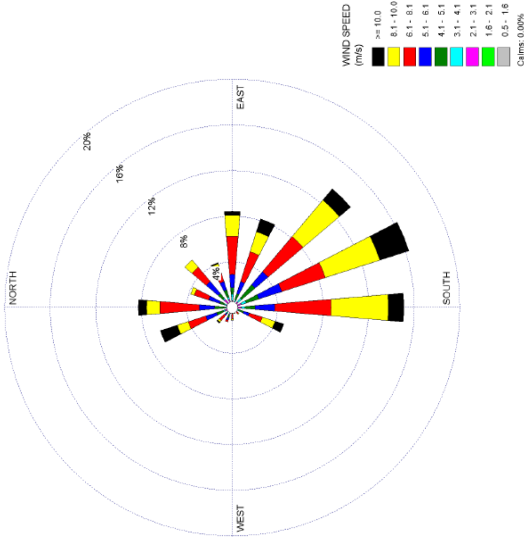
Figure 2.7-13 STP 60-Meter Level 3-Year Composite Wind Rose - April (1997, 1999, and 2000) - Page 4 of 12
