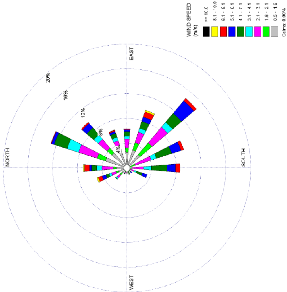
Figure 2.7-7 STP 10-Meter Level 3-Year Composite Wind Rose - September (1997, 1999, and 2000) - Page 9 of 12
