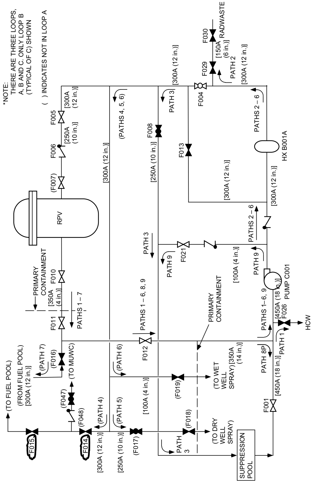
Figure 19L-3 Potential Path for Draining RPV Through Residual Heat Removal System (Pump On)
