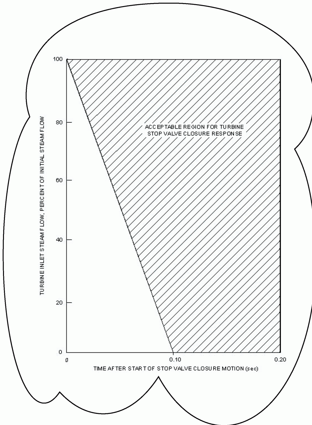
Figure 10.2-1 Turbine Stop Valve Closure Characteristic
