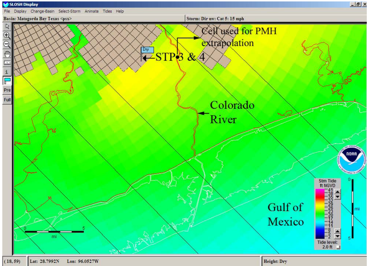
Figure 2.4S.5-6 The Maximum of Maximum (MOM) Storm Surge for a Category 5 Hurricane at STP 3 & 4
