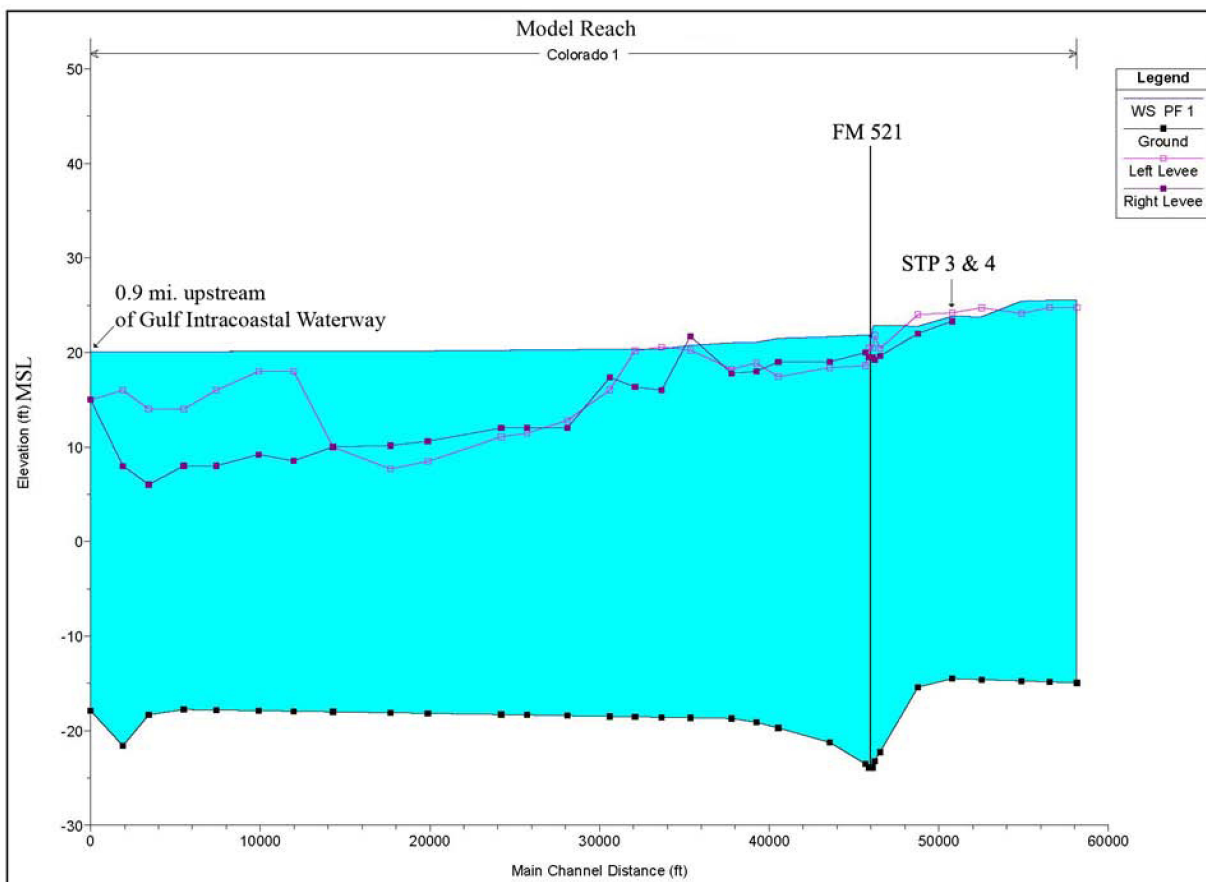
Longitudinal Profile of Water Surface (WS) Elevation
