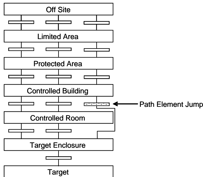
Figure 2-16. Adversary sequence diagram with a jump.
