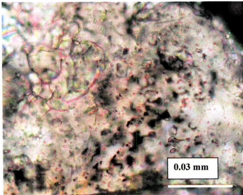
Figure 9. Cross-polarized light image showing small, red, hematite inclusions in calcite.
