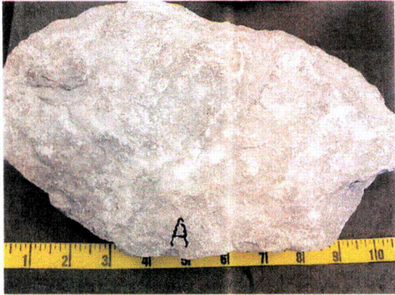
Figure 1. Rock Fragment A.
