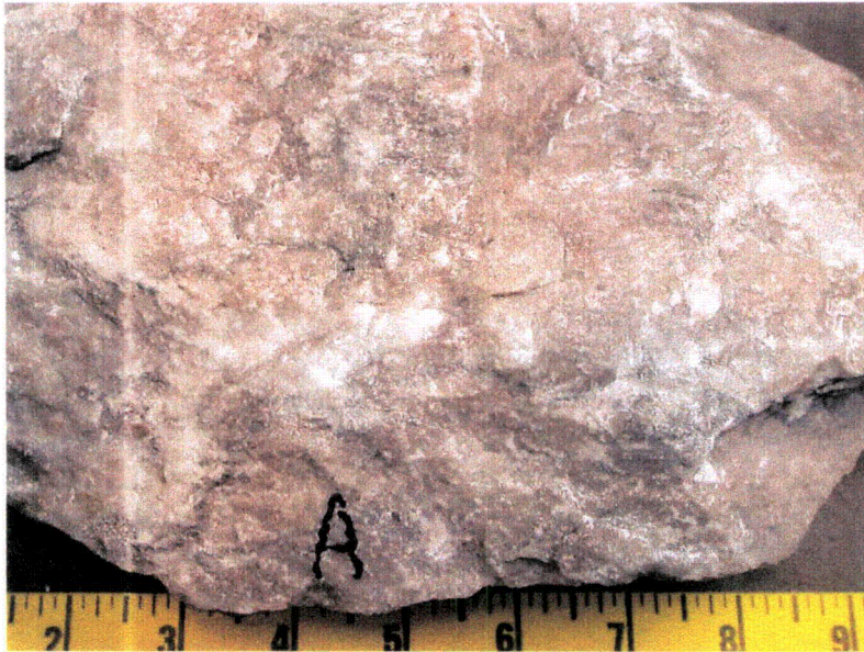
Figure 4. After washing, the Rock Fragment A is shown to be mottled pinkish-beige, gray and white.
