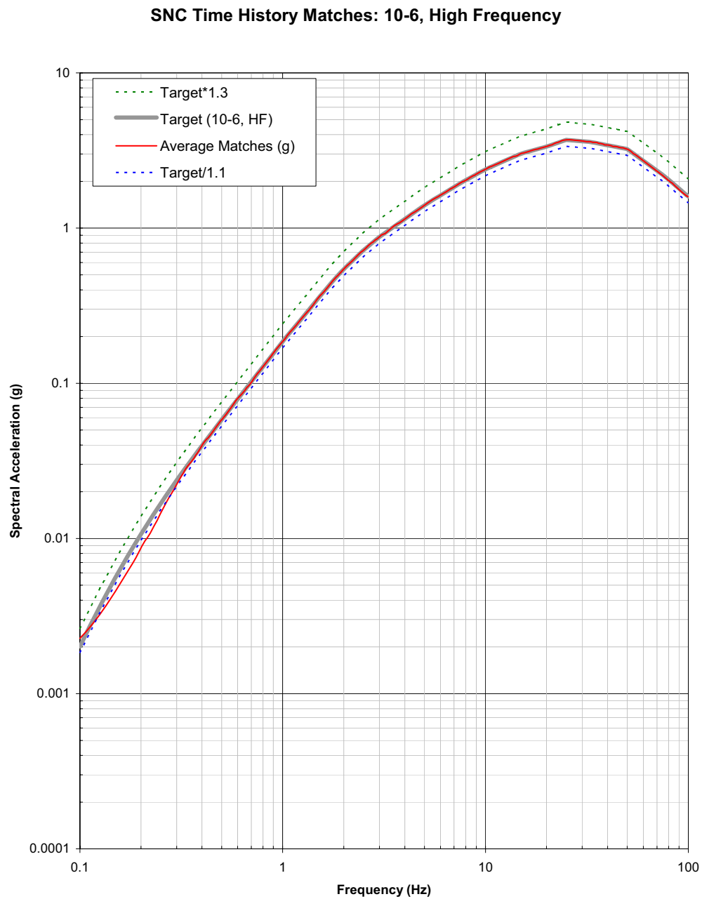
Figure 5. Comparison between the linear average of the suite of 30 spectrum compatible time histories (red line), target spectrum (thick gray line), target spectrum divided by 1.1 (dashed blue line), and target spectrum multiplied by 1.3 (dashed green line) for the high frequency 10^{-6} case.
