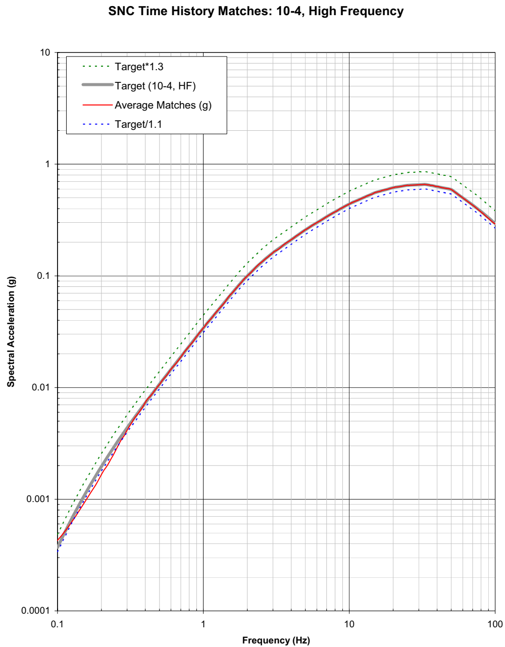
Figure 1. Comparison between the linear average of the suite of 30 spectrum compatible time histories (red line), target spectrum (thick gray line), target spectrum divided by 1.1 (dashed blue line), and target spectrum multiplied by 1.3 (dashed green line) for the high frequency 10 -4 case.
