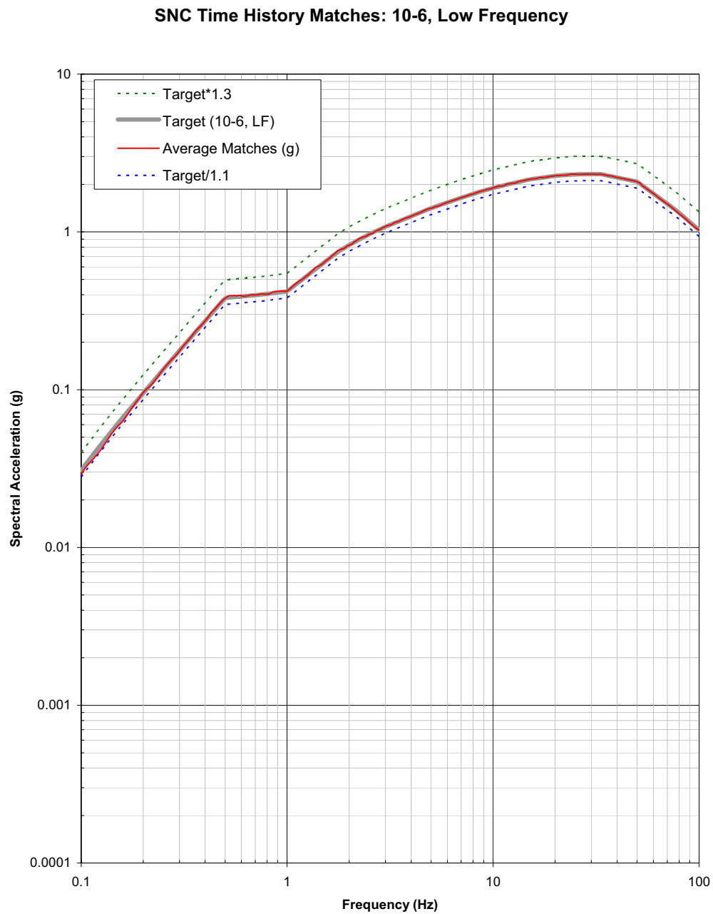
Figure 6. Comparison between the linear average of the suite of 30 spectrum compatible time histories (red line), target spectrum (thick gray line), target spectrum divided by 1.1 (dashed blue line), and target spectrum multiplied by 1.3 (dashed green line) for the low frequency 10^{-6} case.
