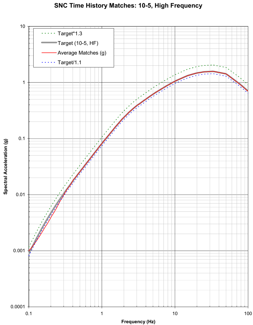
Figure 3. Comparison between the linear average of the suite of 30 spectrum compatible time histories (red line), target spectrum (thick gray line), target spectrum divided by 1.1 (dashed blue line), and target spectrum multiplied by 1.3 (dashed green line) for the high frequency 10^{-5} case.
