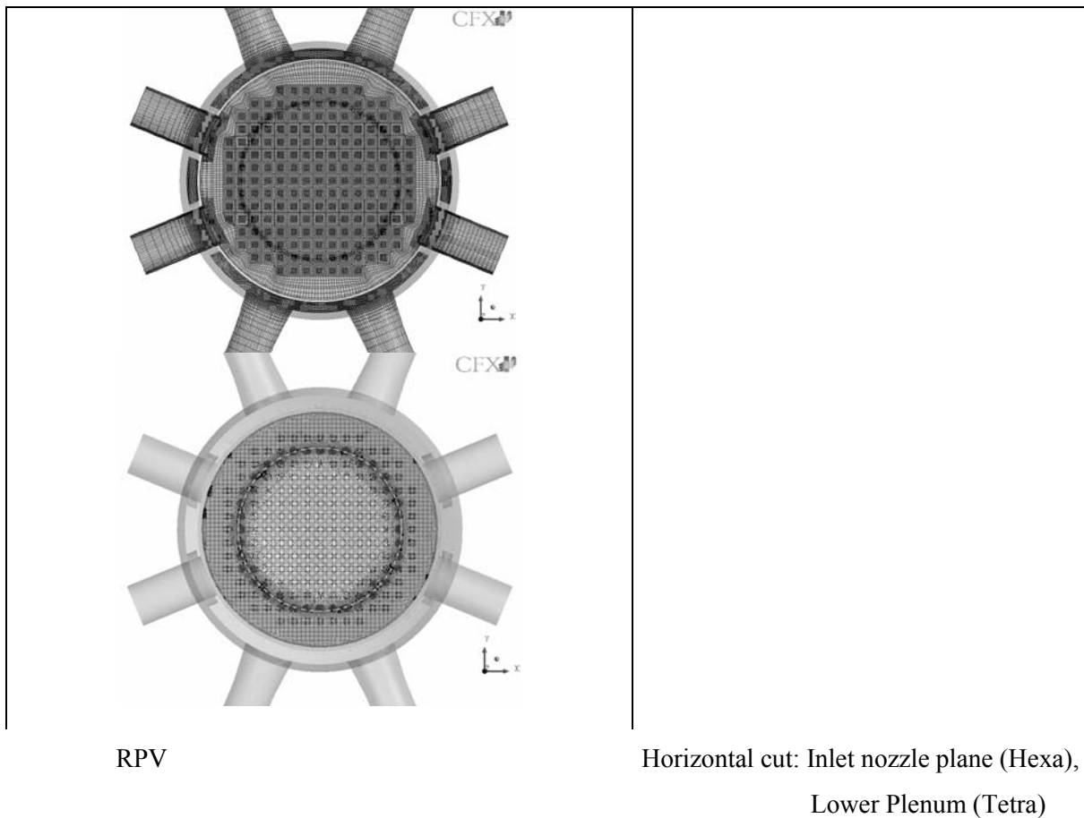
Figure 11.1. Hybrid mesh based on tetrahedral and hexahedral elements
