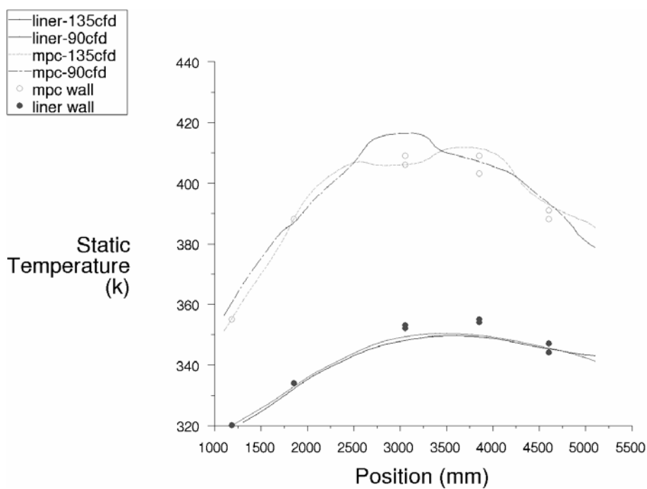
Figure 11.18 MPC and liner walls axial temperature, using low Reynolds k-\epsilon turbulence model
