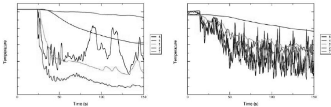
Figure 11.7. : Level 750 mm results of the CFX-5 reference calculation (left) and UPTF experiment (right). For legend see Figure 11.4
