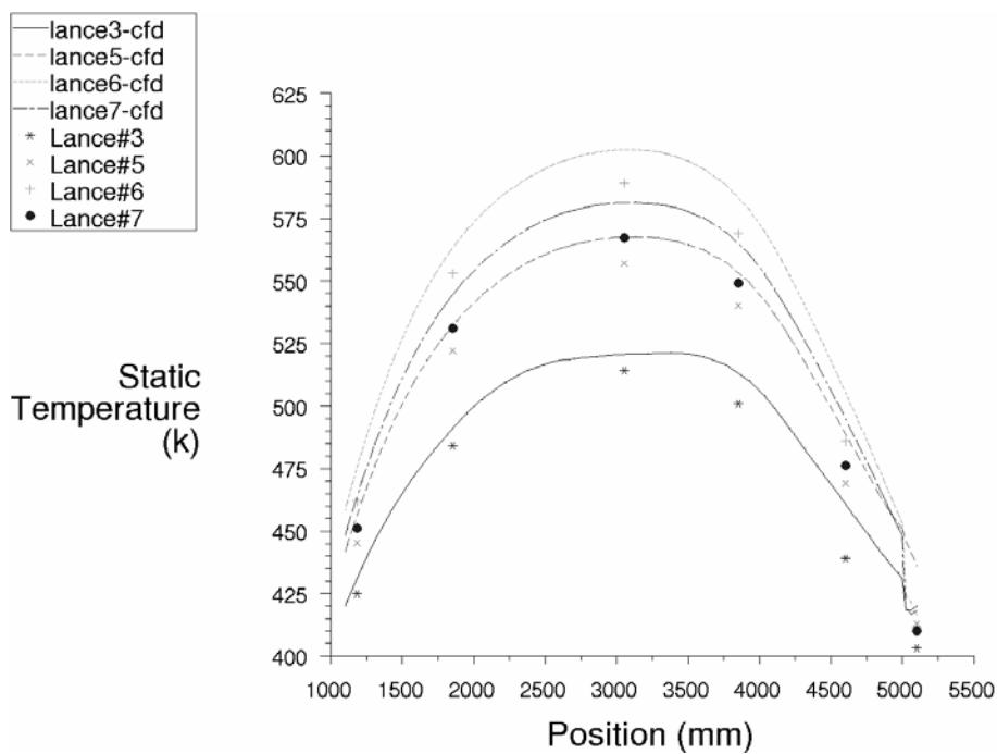
Figure 11.22 Fuel region axial temperature, using laminar option
