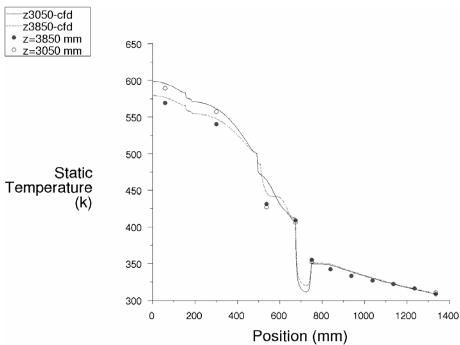
Figure 11.14 Radial temperature plot at 3.05 and 3.85 m elevation using SST k-\omega turbulence model
