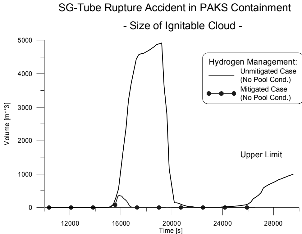
Figure 11.28 Size of ignitable clouds for unmitigated and mitigated cases
