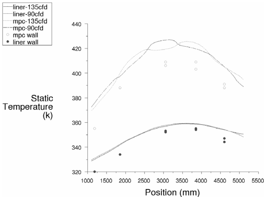
Figure 11.24 MPC and liner walls axial temperature using laminar option
