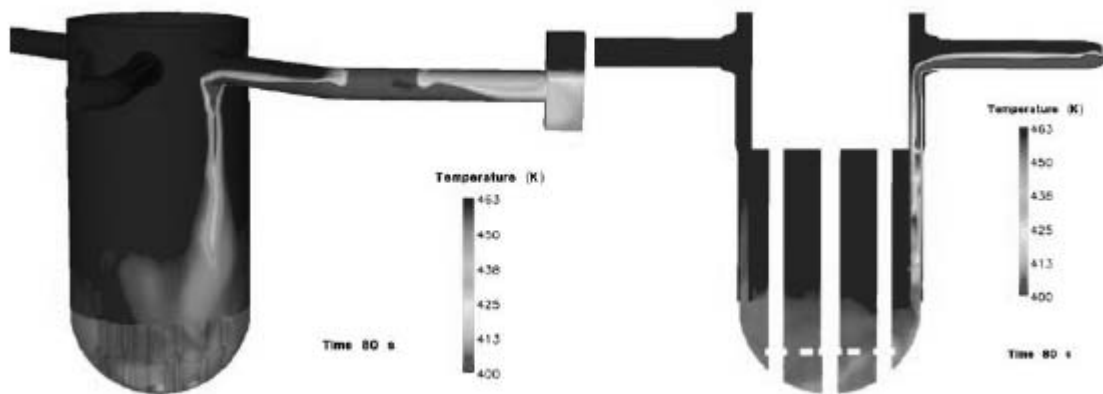
Figure 11.5. Vessel and fluid temperatures on the vessel and cold leg walls (left) and a cross-section through the middle of the cold leg with ECC injection (right)
