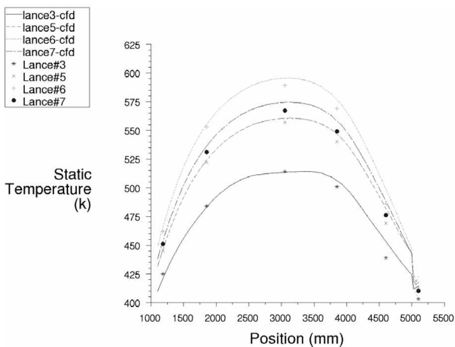
Figure 11.13 Fuel region axial temperature, using SST k-\omega turbulence model
