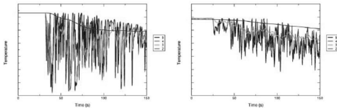
Figure 11.8. Level 4500 mm results of the CFX-5 reference calculation (left) and UPTF experiment (right). For legend see Figure 11.4
