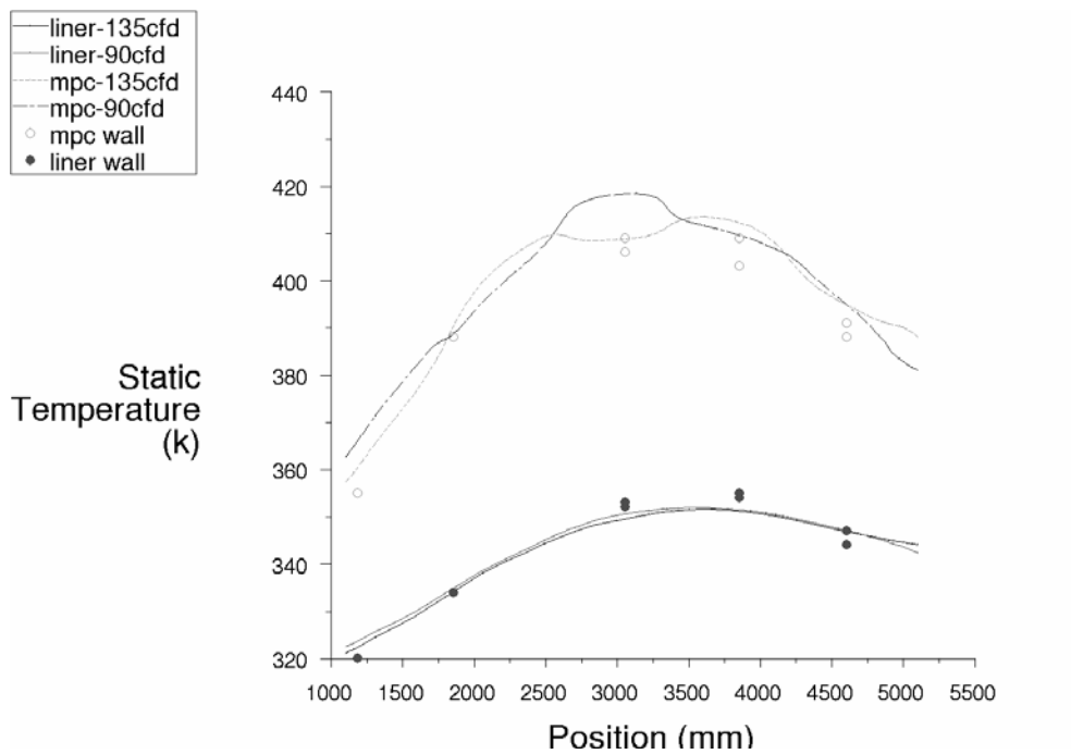
Figure 11.15 MPC and liner walls axial temperature, using SST k-\omega turbulence model
