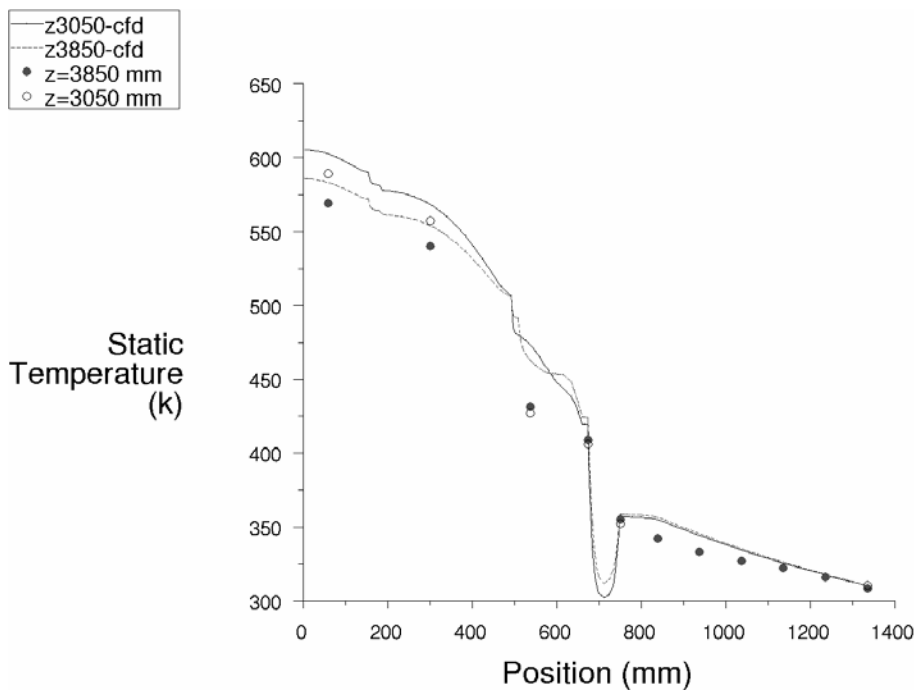
Figure 11.23 Radial temperature at 3.05 and 3.85 m, using laminar option
