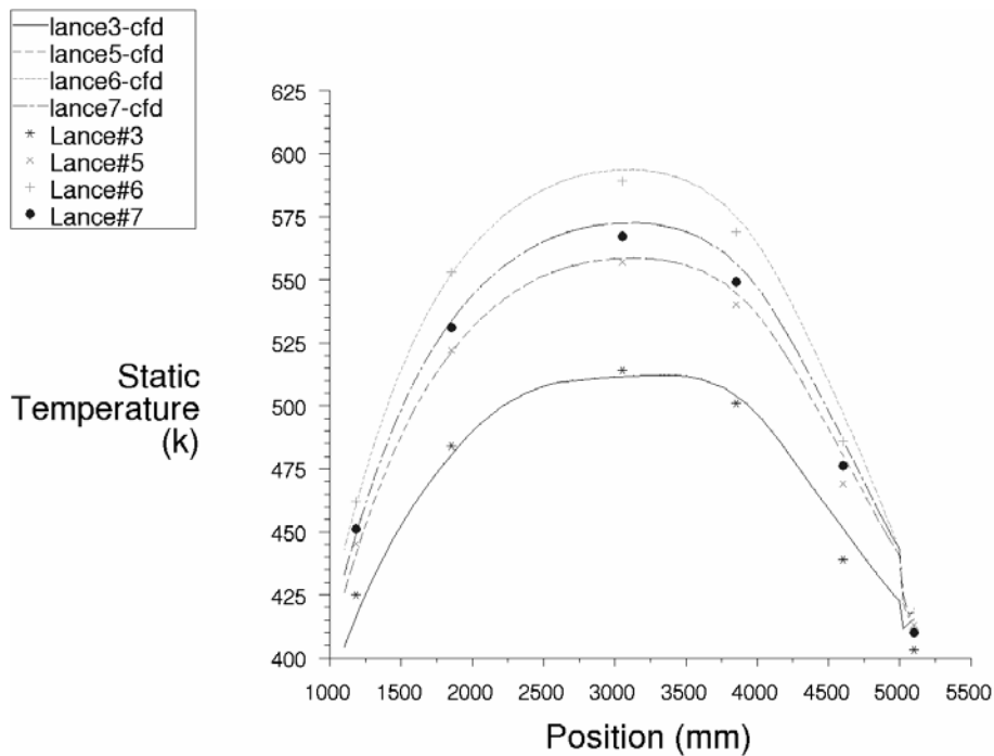
Figure 11.16 Fuel region axial temperature, using low Reynolds k-\epsilon turbulence model.
