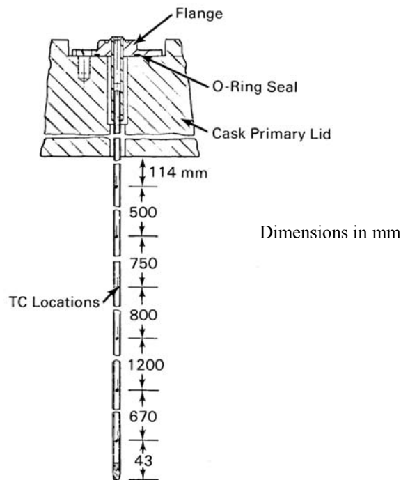
Figure 11.11, Thermocouple Lance
