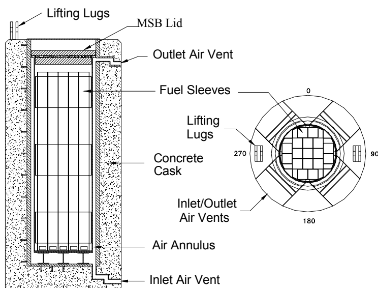
Figure 11.10 Schematic of the ventilated concrete cask system.
