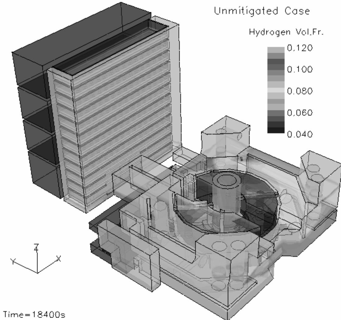
Figure 11.26 Distribution of hydrogen in the containment in the unmitigated case
