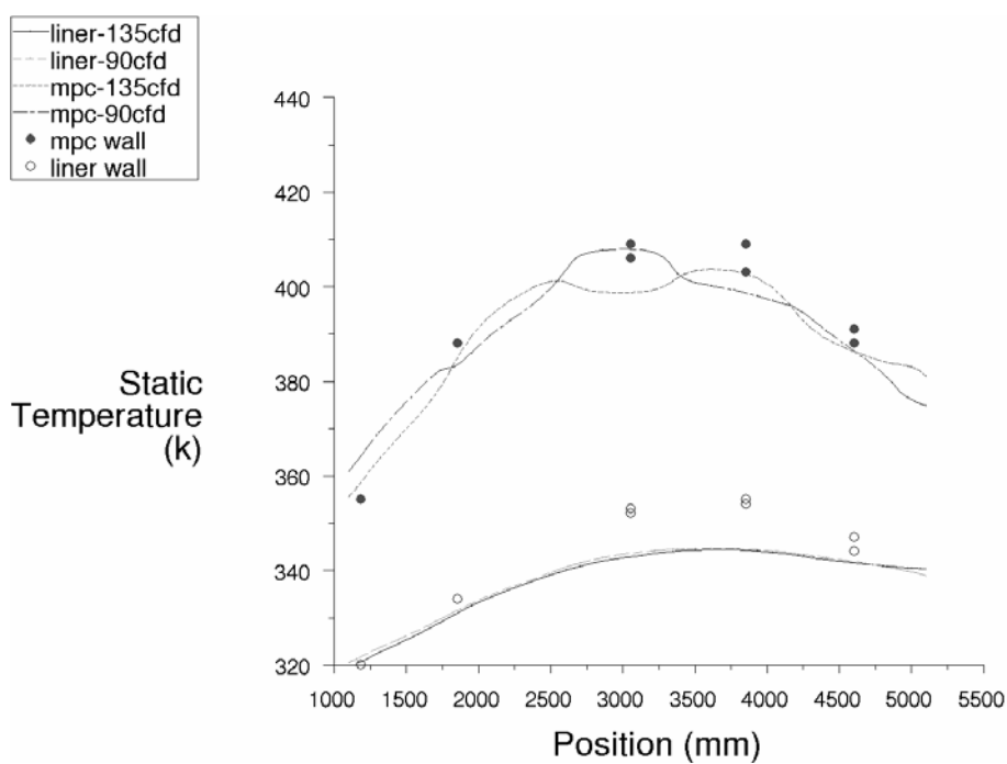
Figure 11.21 MPC and liner walls axial temperature, using standard k- \epsilon turbulence model
