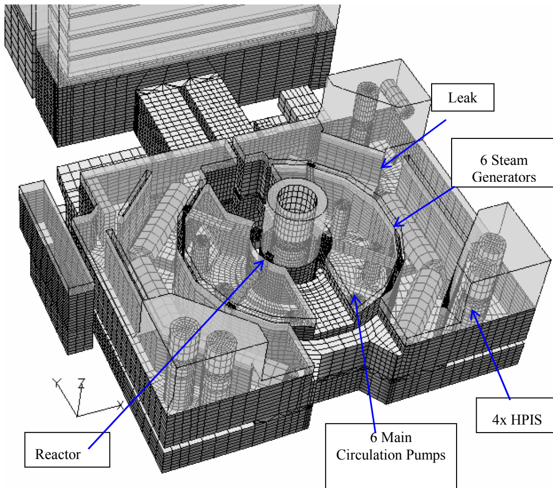
Figure 11.25 View of main components and the surface mesh of the modeled containment
