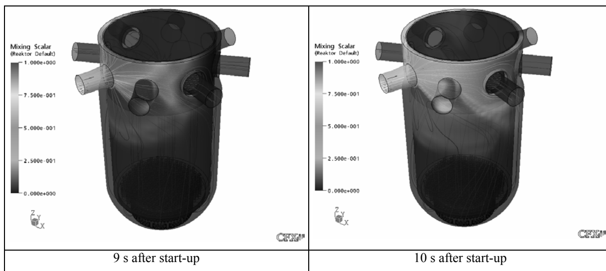
Figure 11.2. Time dependent mixing scalar distribution in the downcomer, CFX-5
