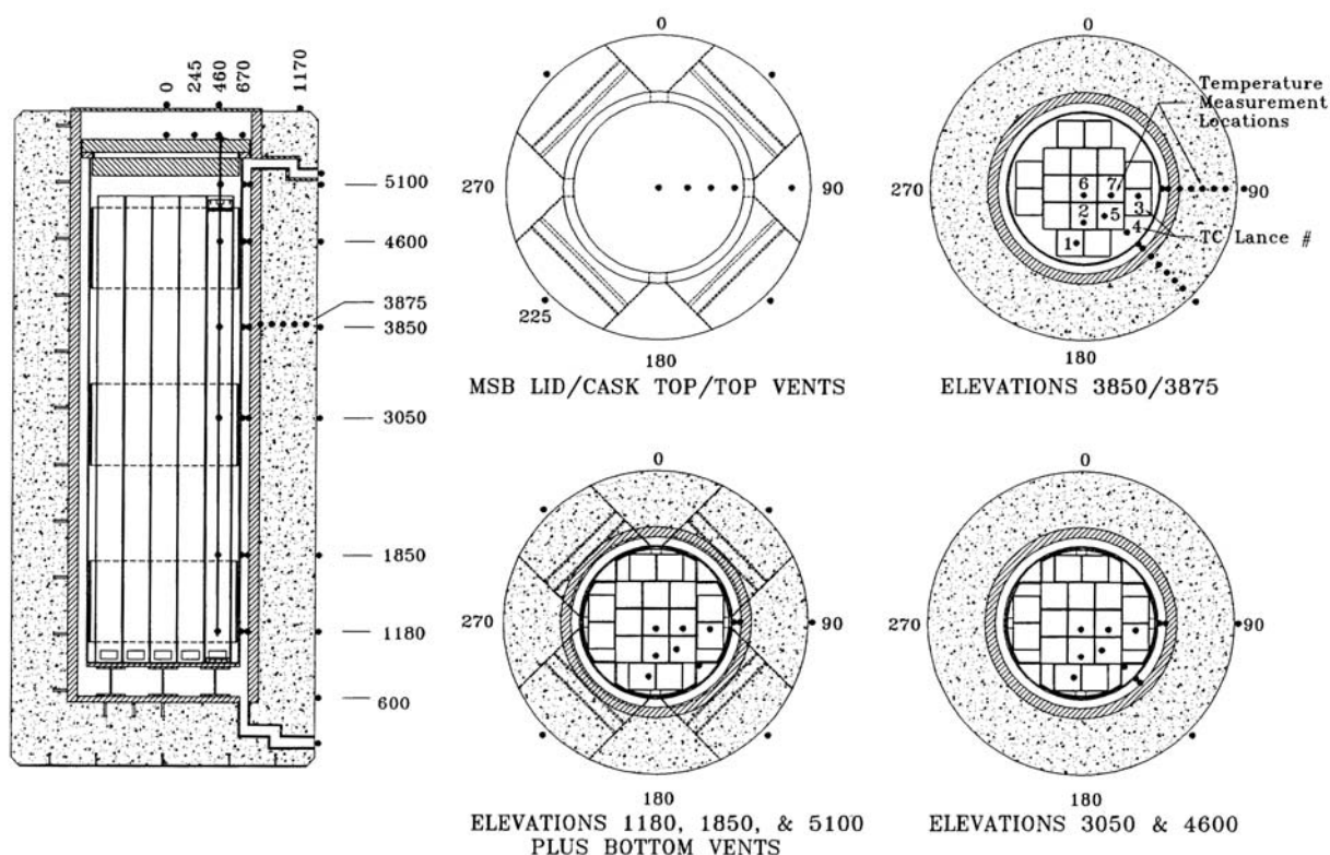
Figure 11.12 Temperature Measurement Locations Used During the VSC-17 Performance Test
