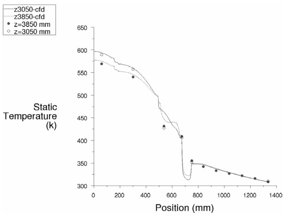
Figure 11.17 Radial Temperature at 3.05 and 3.85 m elevation, using low Reynolds k-\epsilon turbulence
