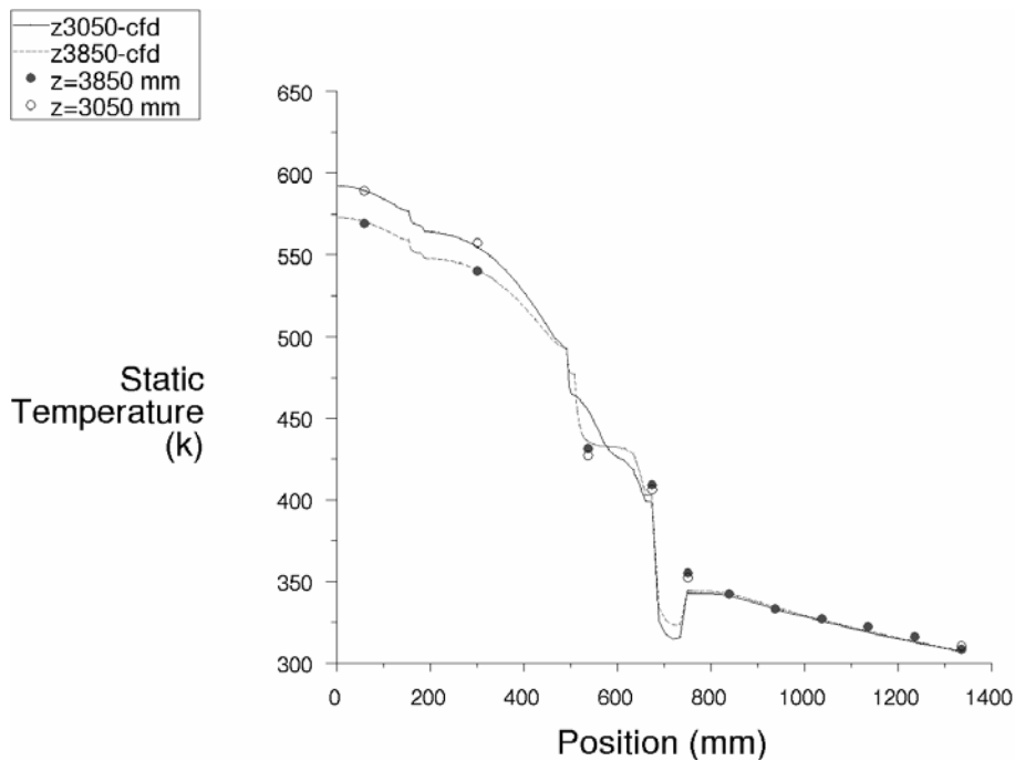
Figure 11.20 Radial temperature at 3.05 and 3.85 m, using standard k- \epsilon turbulence model
