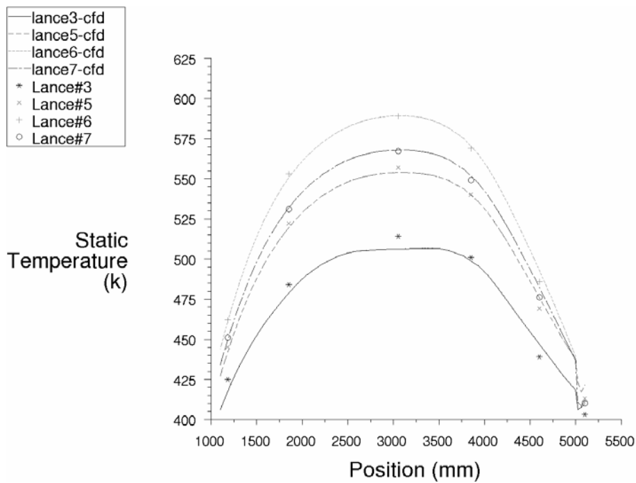
Figure 11.19 Fuel region axial temperature, using standard k- \epsilon turbulence model
