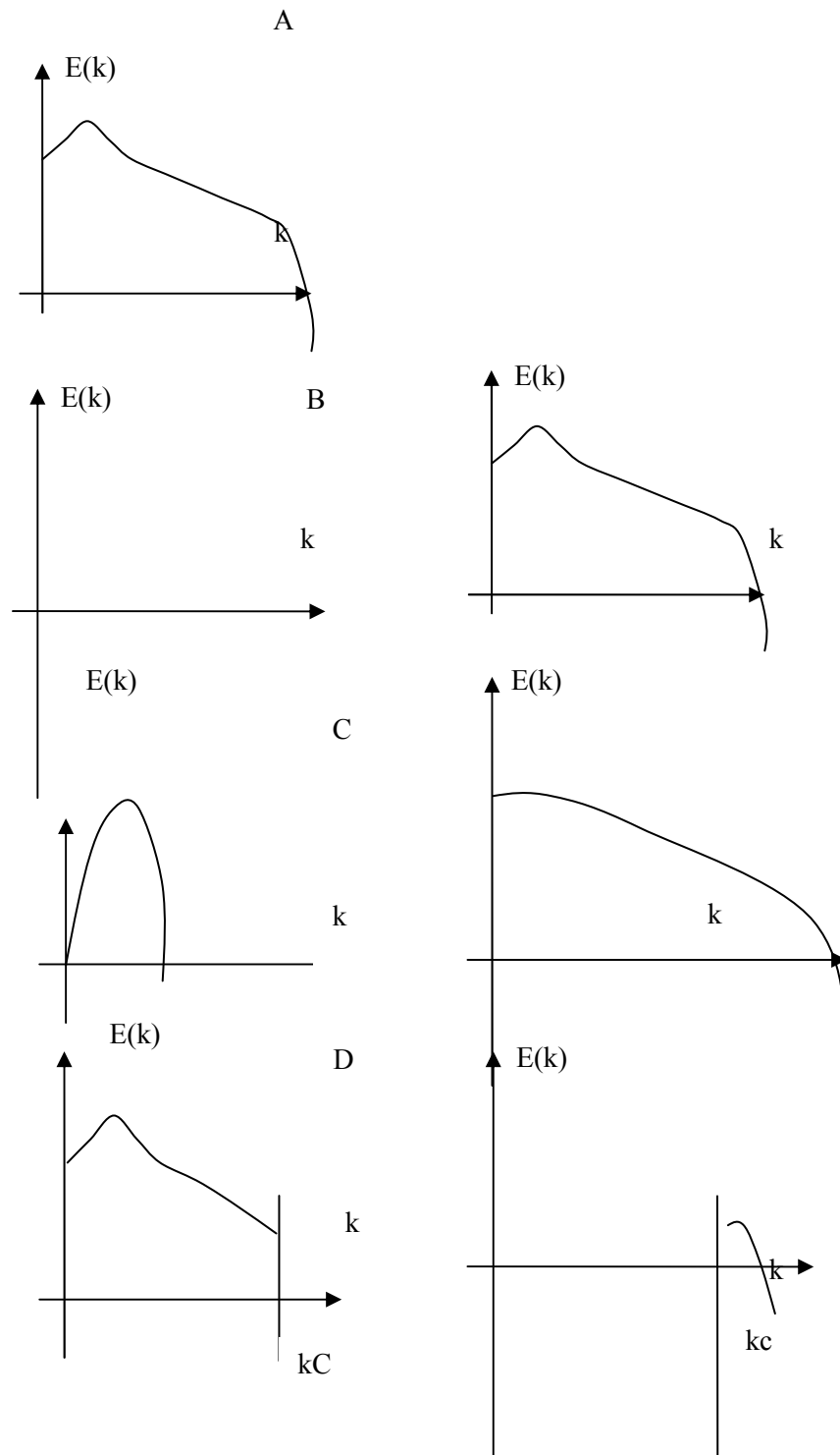
Fig. 5.1 Part of the turbulent spectrum that is explicitly simulated (Left) and modelled (Right) for DNS (A); steady RANS (B); U-RANS (C) and LES (D); from [172].
