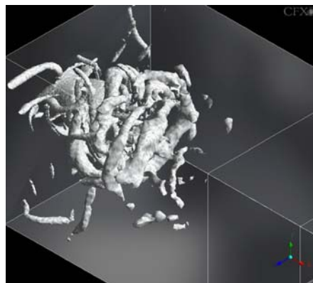
Figure 5.3 Iso-surfaces of S^2-\Omega^2 for ITS combustion chamber computed with SST-SAS model
