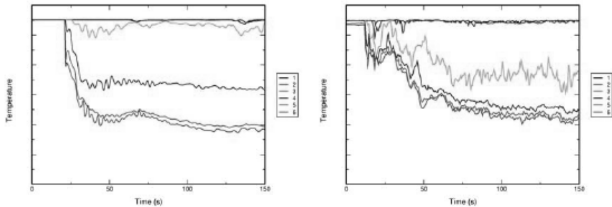
Figure 11.6. Stalk 3 results of the CFX-5 reference calculation (left) and UPTF experiment (right). For location see Figure 11.4
