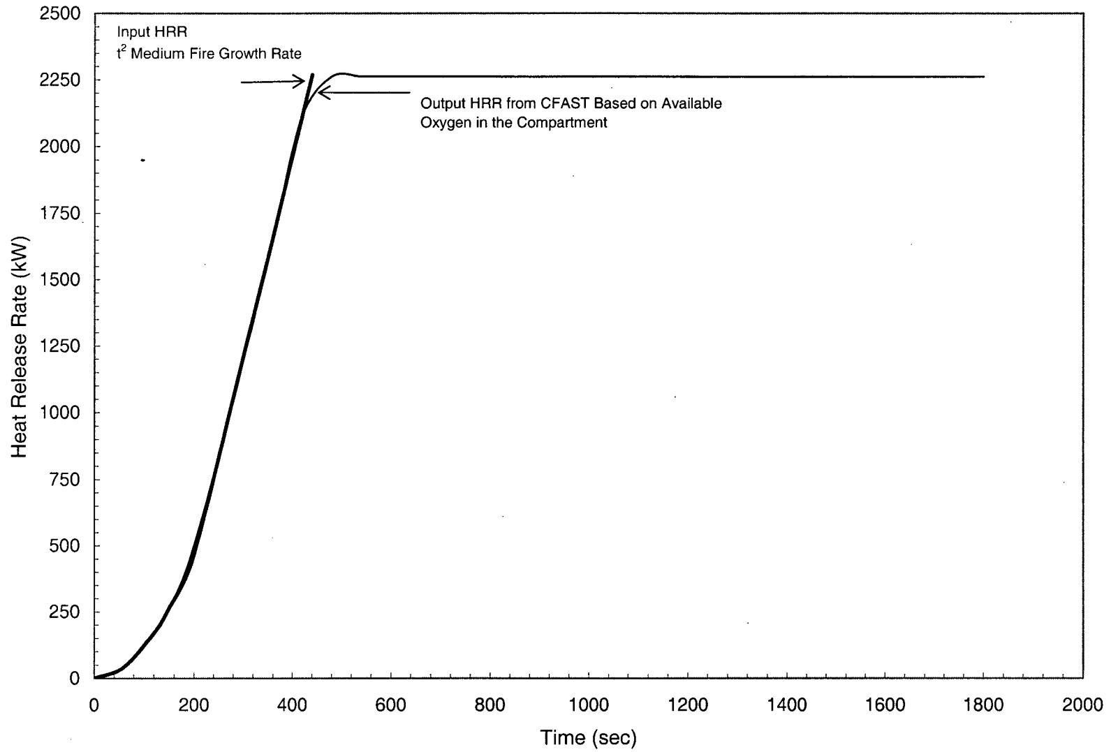
Heat Release Rate for Radiation Protection Office
