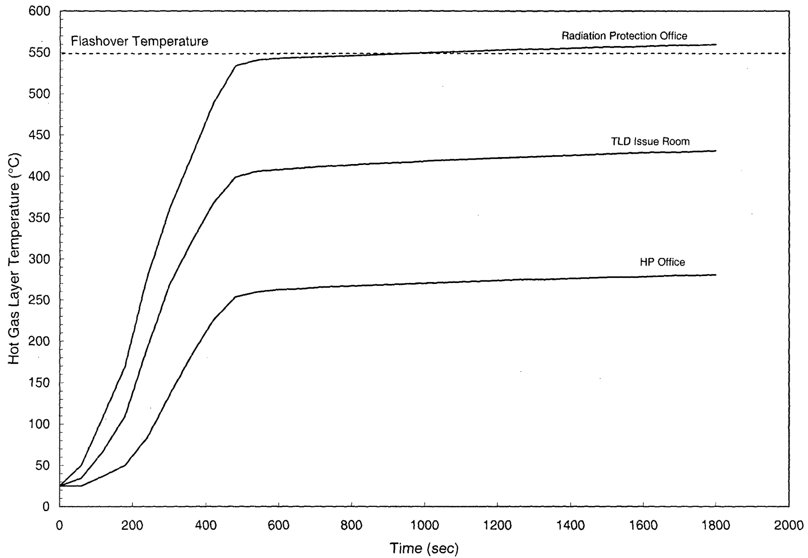
Temperature in Radiation Protection Office, TLD Issue Room, and HP Office
