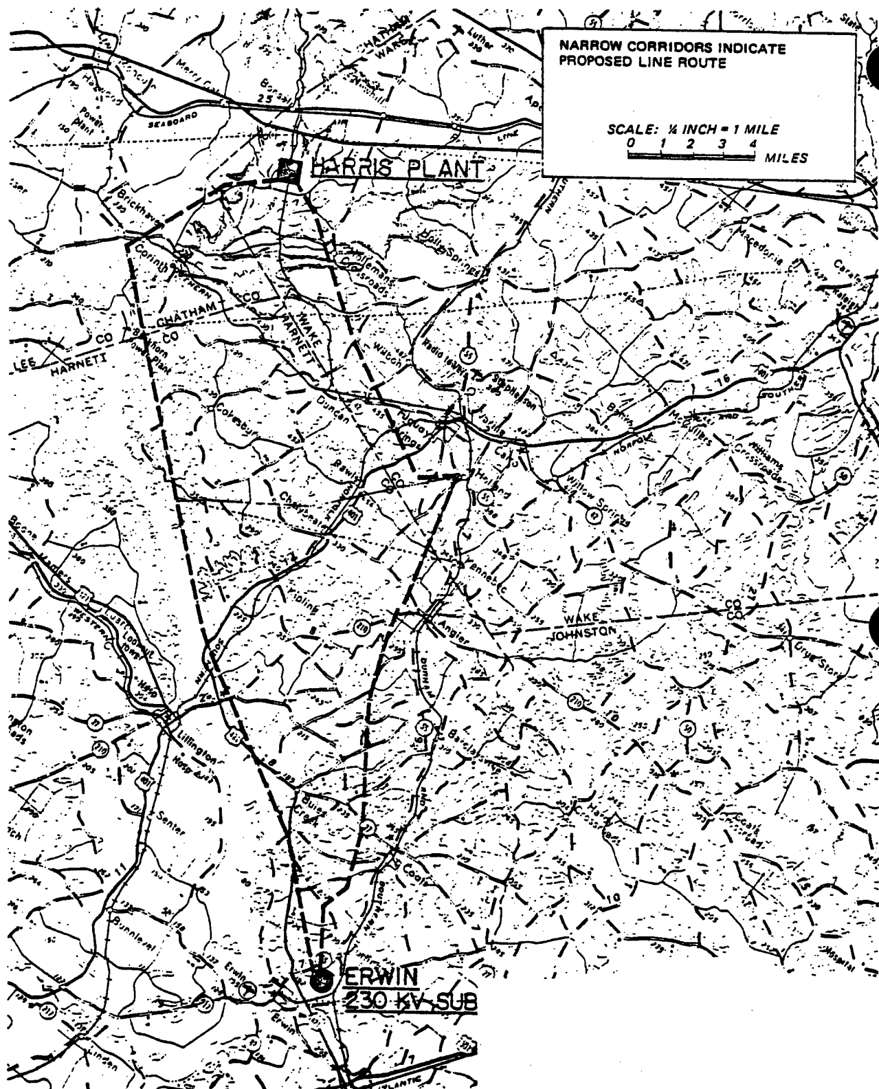
Figure 5.3 Harris-Lillington-Erwin South (proposed) and Harris-Fuquay-Erwin North 230-kV lines (Source: ER-OL Figure 3.9.0-2, Amendment 3)
