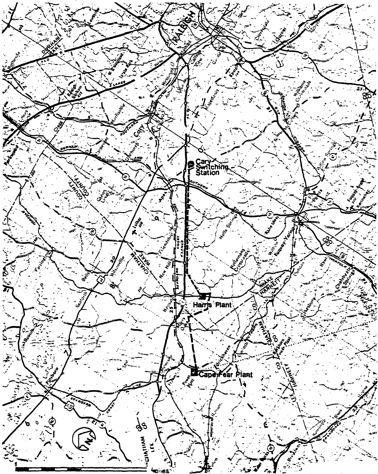
Figure 5.2 Harris-Cary switching 230-kV line and Harris-Cape Fear 230-kV line (Source: ER-0L Figure 3.9.0-1, Amendment 3)
