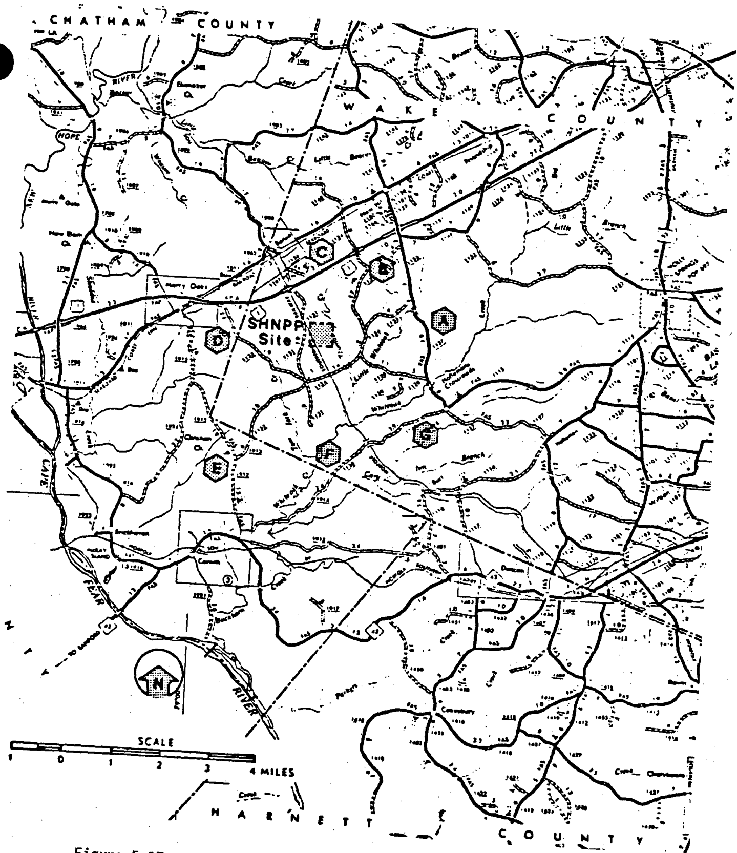
Figure 5.17 Ambient noise measurement locations in the Shearon Harris site vicinity (from ER-0L Figure 2.7.2-1)
