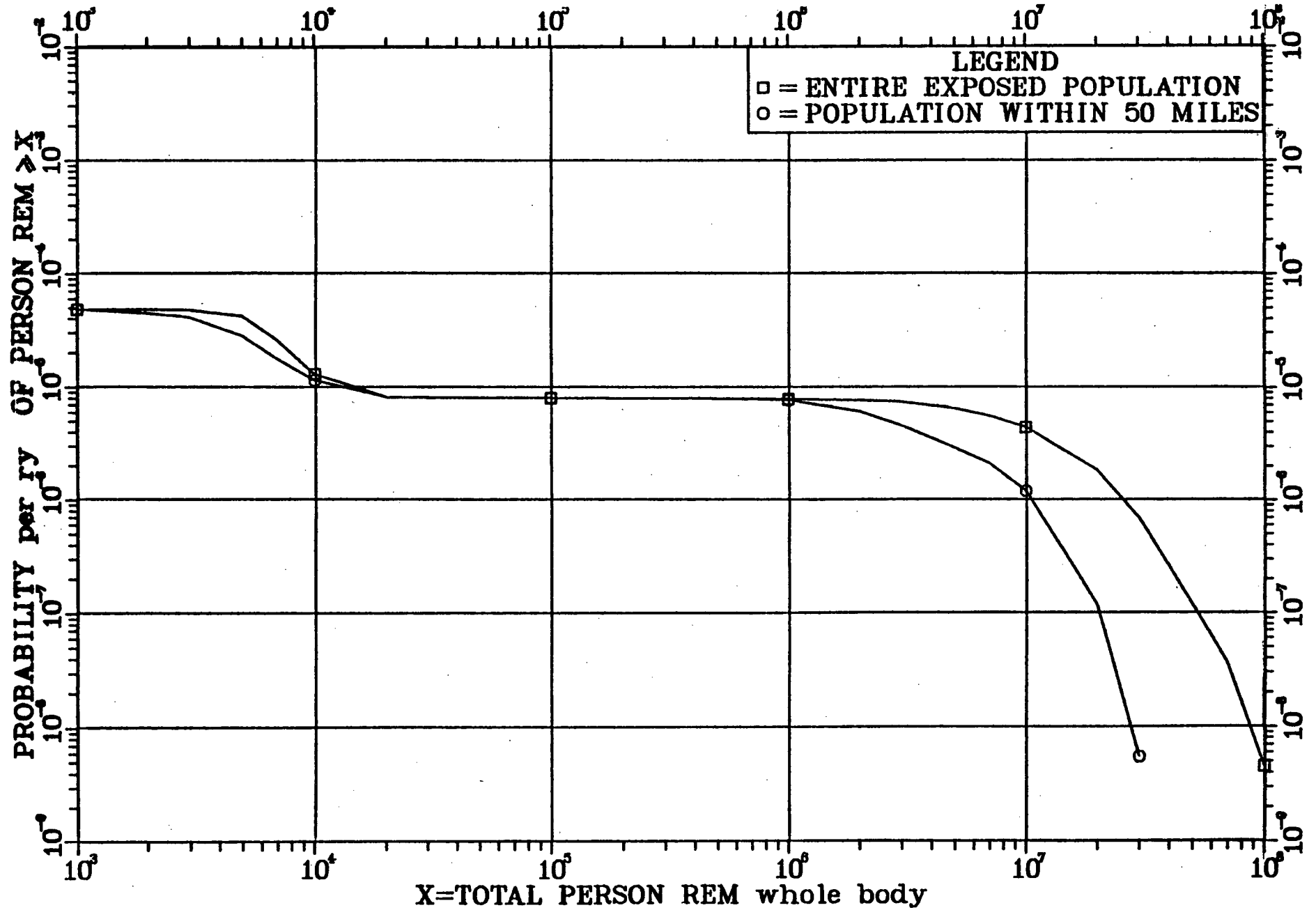
Figure 5.9 Probability distributions of population exposures (see Section 5.9.4.5(7) for a discussion of uncertainties in peak estimate) (50 mi = 80 km)
