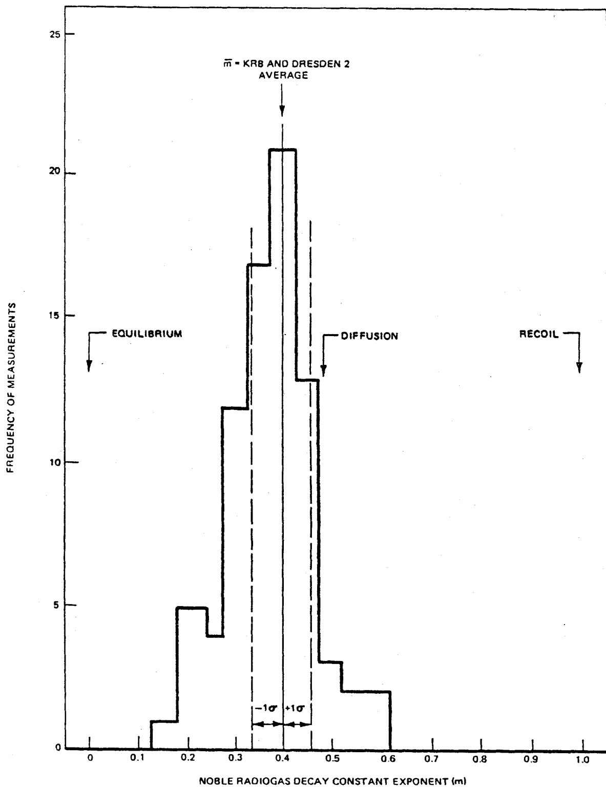
Figure 11.1-1. Noble Radiogas Decay Constant Exponent Frequency Histogram
